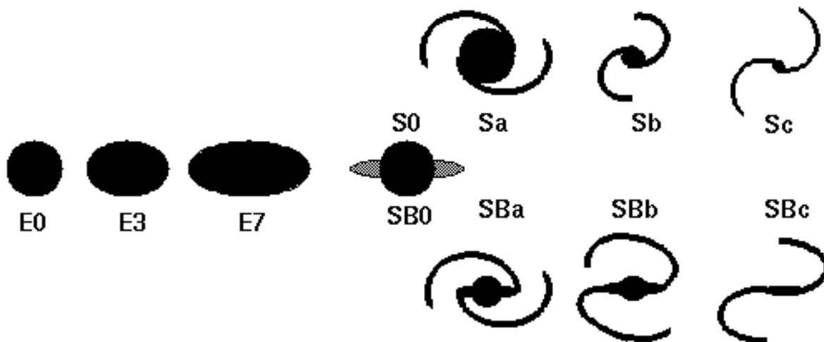
Figure 1: A simple schematic of Hubble's Tuning Fork
