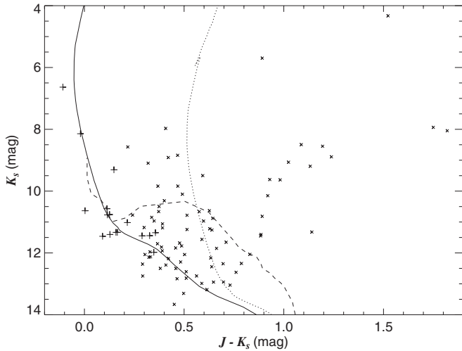
Figure 11. Color–magnitude diagram for 2MASS J and K_s magnitudes (in the same format as Figure 10). The bright, red object (top, right) is IRAS 20161+4035.
