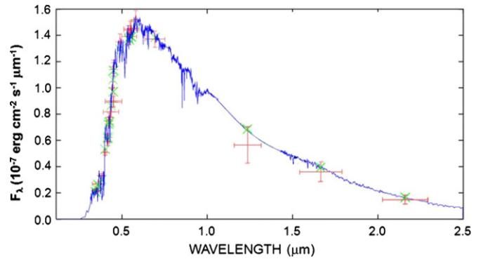
Figure 3. HR 2582 SED fit. The solid-line spectrum is a K1 III spectral template from Pickles (1998). The crosses indicate photometry values from the literature and the horizontal bars represent bandwidths of the filters used. The X-shaped symbols show the flux value of the spectral template integrated over the filter transmission.
