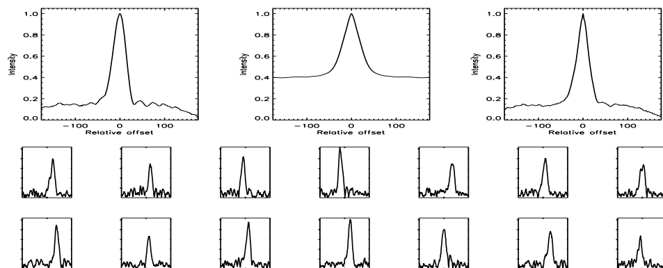
FIGURE B.210: SFP inspection for HD 079096 with S1-E1 on UT 2008/04/14, seq 001
