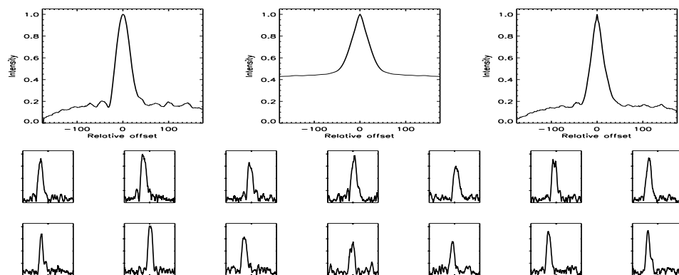
FIGURE B.211: SFP inspection for HD 079096 with S1-E1 on UT 2008/04/14, seq 002
