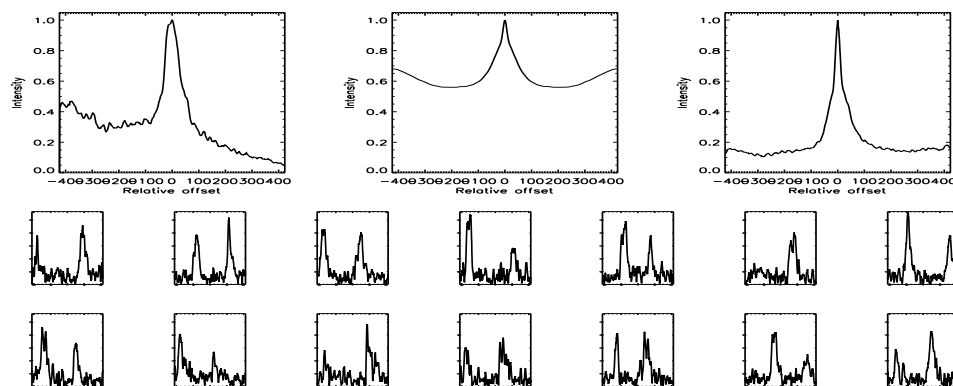
FIGURE B.214: SFP inspection for HD 079096 with S2-E2 on UT 2007/11/29, seq 002
