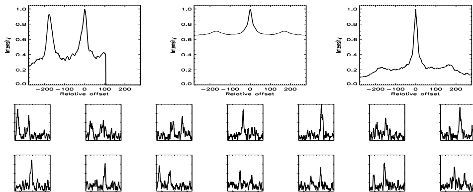
FIGURE B.205: SFP inspection for HD 079096 with S1-E1 on UT 2007/02/25, seq 002
