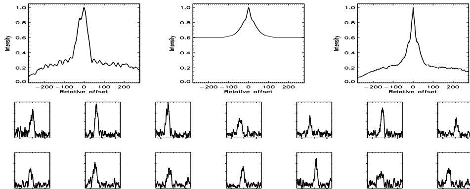
FIGURE B.203: SFP inspection for HD 079096 with S1-E1 on UT 2007/02/06, seq 003
