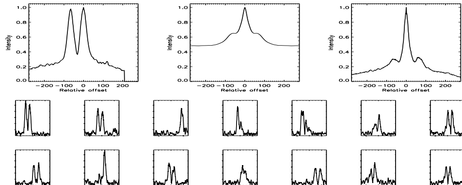
FIGURE B.209: SFP inspection for HD 079096 with S1-E1 on UT 2007/03/11, seq 001
