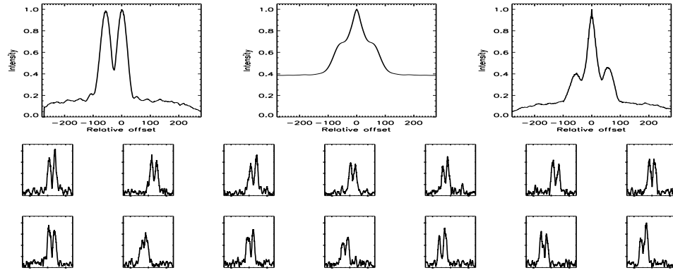
FIGURE B.206: SFP inspection for HD 079096 with S1-E1 on UT 2007/03/09, seq 001
