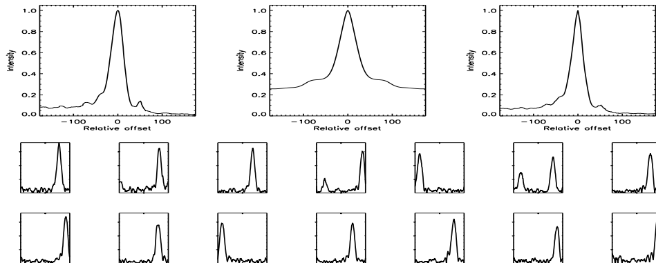
FIGURE B.386: SFP inspection for HD 137763 with S1-W1 on UT 2008/04/14, seq 001
