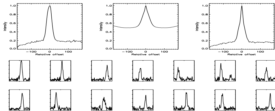
FIGURE B.390: SFP inspection for HD 137763 with S2-W2 on UT 2008/06/09, seq 001
