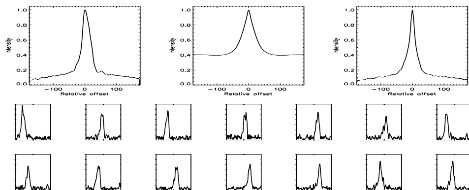
FIGURE B.385: SFP inspection for HD 137763 with S1-E1 on UT 2008/06/23, seq 001
