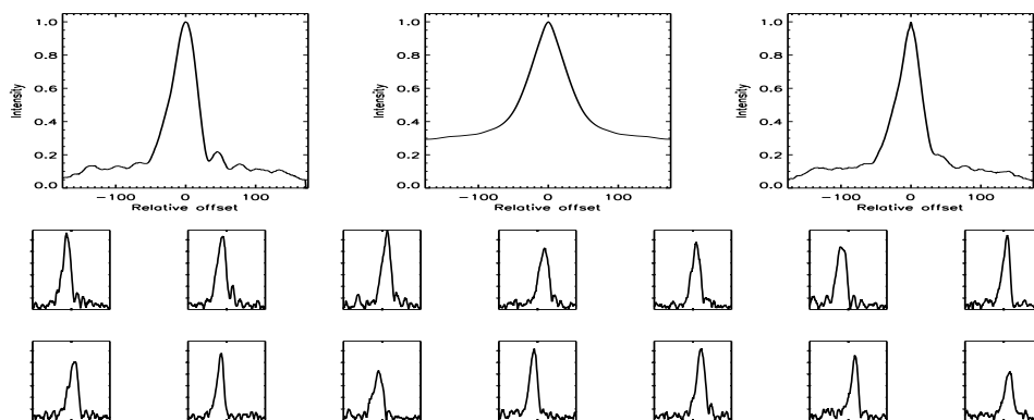
FIGURE B.388: SFP inspection for HD 137763 with S1-W1 on UT 2008/07/07, seq 001
