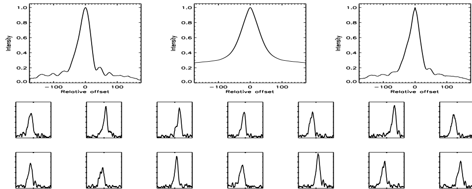
FIGURE B.389: SFP inspection for HD 137763 with S1-W1 on UT 2008/07/07, seq 002
