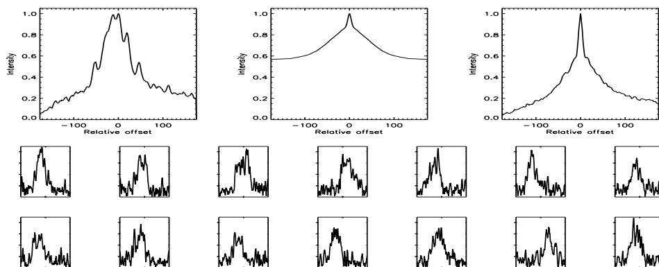
FIGURE B.387: SFP inspection for HD 137763 with S1-W1 on UT 2008/06/22, seq 001
