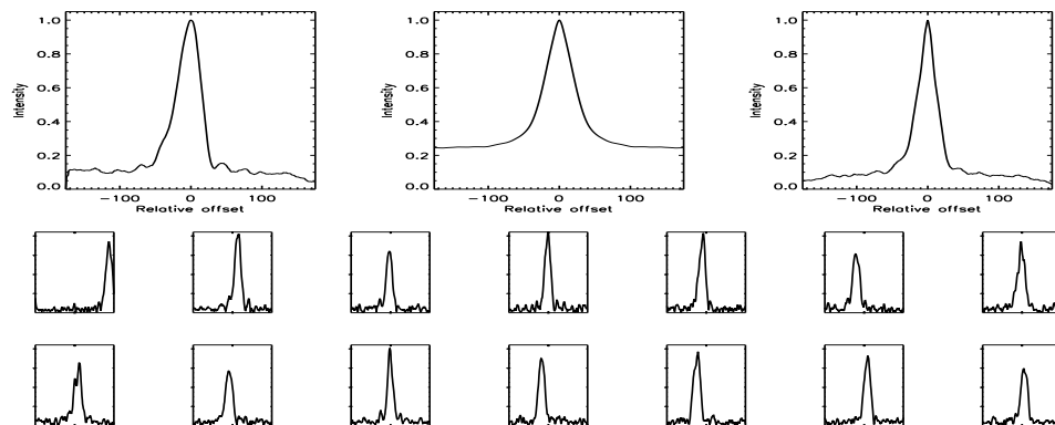
FIGURE B.383: SFP inspection for HD 136923 with S1-W1 on UT 2008/04/13, seq 002
