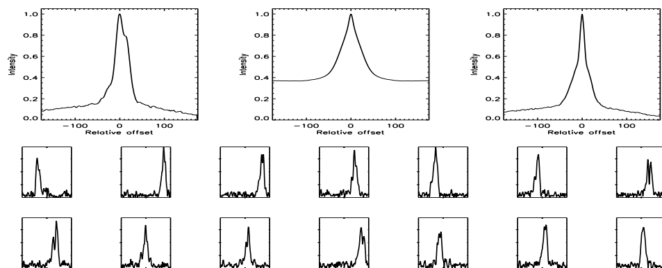
FIGURE B.391: SFP inspection for HD 137778 with S1-E1 on UT 2008/04/25, seq 001
