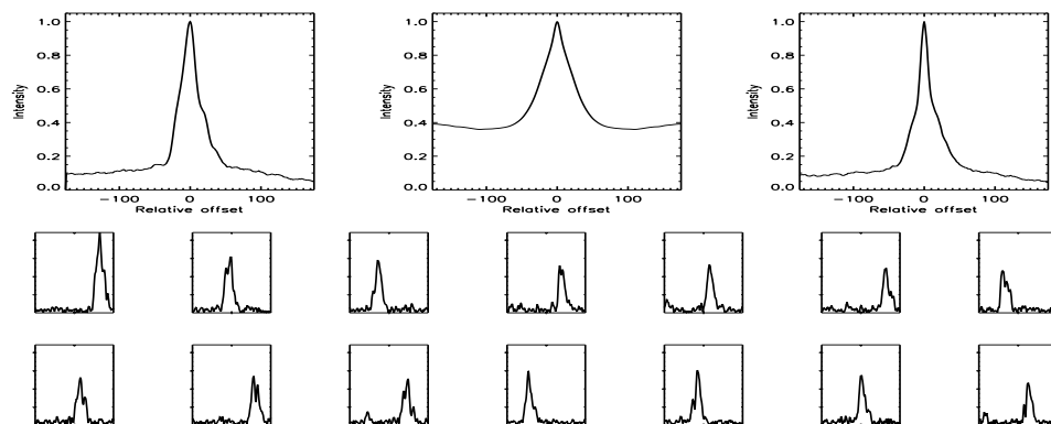
FIGURE B.384: SFP inspection for HD 137763 with S1-E1 on UT 2008/04/25, seq 001
