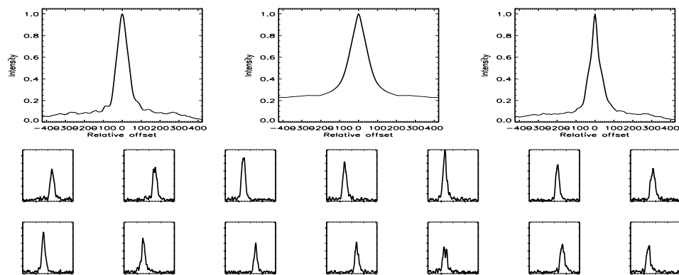
FIGURE B.114: SFP inspection for HD 025457 with S1-W1 on UT 2007/10/31, seq 002
