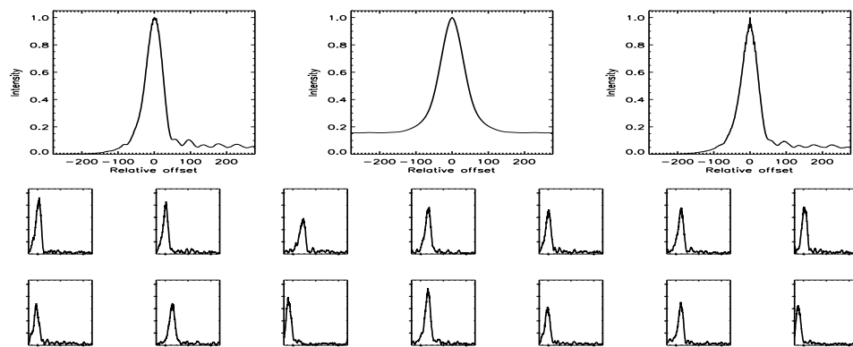
FIGURE B.249: SFP inspection for HD 098230 with S1-E1 on UT 2007/05/17, seq 001
