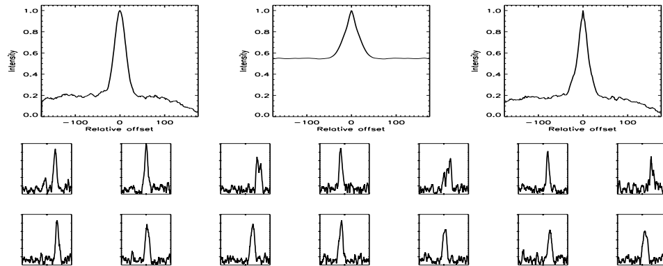
FIGURE B.272: SFP inspection for HD 101206 with S1-E1 on UT 2008/04/12, seq 002
