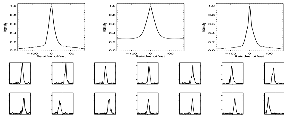
FIGURE B.651: SFP inspection for HD 222404 with S1-W1 on UT 2008/04/26, seq 001
