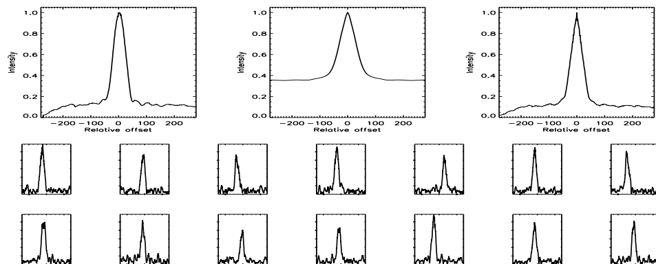
FIGURE B.617: SFP inspection for HD 217107 with S1-W1 on UT 2007/08/14, seq 002
