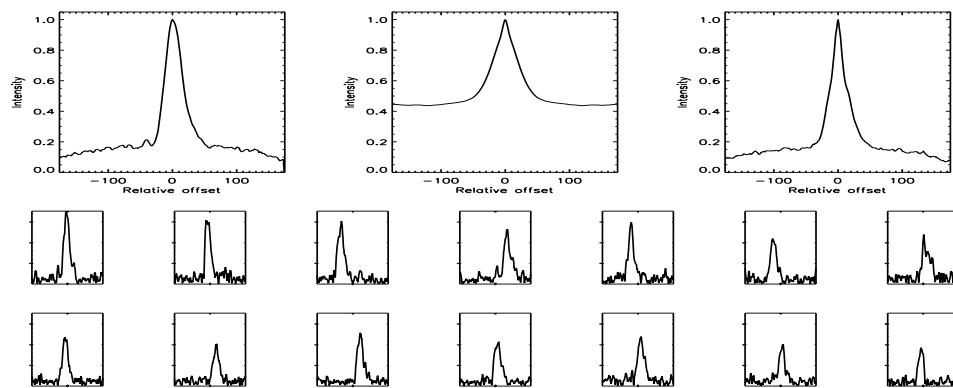
FIGURE B.252: SFP inspection for HD 098230 with S1-E1 on UT 2008/04/13, seq 001
