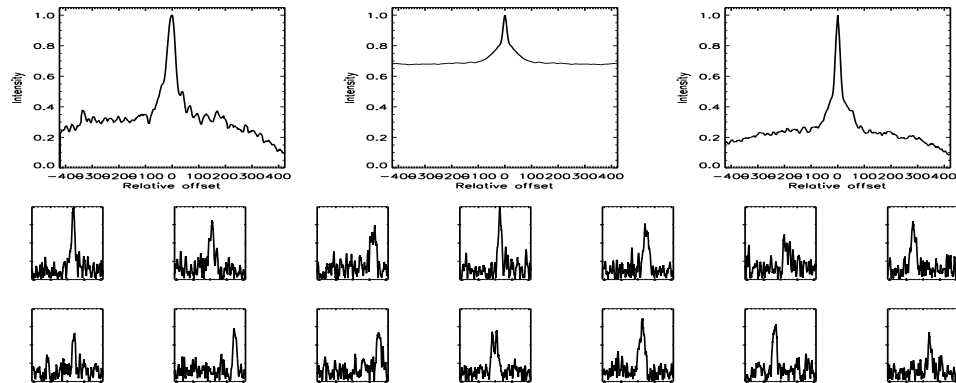
FIGURE B.83: SFP inspection for HD 018632 with S1-E1 on UT 2007/11/01, seq 001
