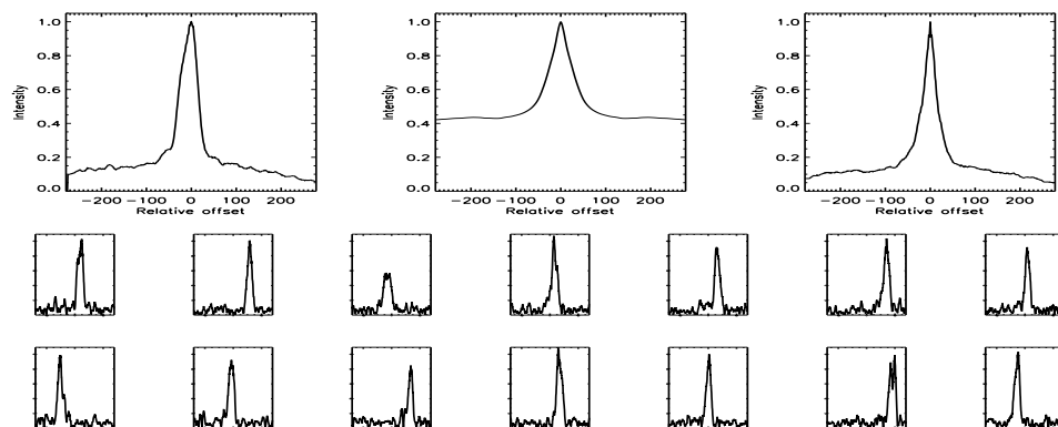
FIGURE B.315: SFP inspection for HD 121560 with S1-W1 on UT 2007/04/24, seq 001
