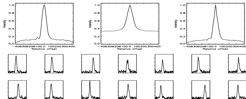
FIGURE B.645: SFP inspection for HD 222143 with S1-E1 on UT 2007/08/18, seq 002
