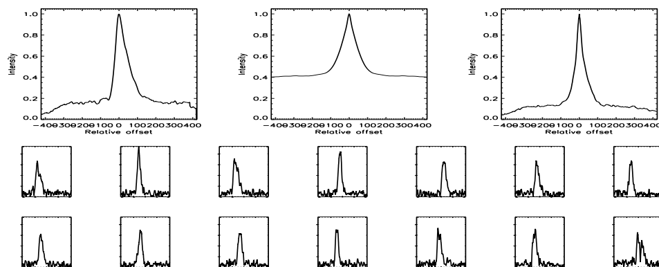
FIGURE B.640: SFP inspection for HD 221354 with S1-W1 on UT 2007/09/16, seq 001
