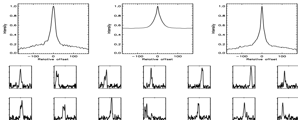
FIGURE B.597: SFP inspection for HD 210277 with S1-E1 on UT 2008/06/23, seq 001
