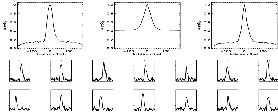
FIGURE B.567: SFP inspection for HD 192263 with S1-E1 on UT 2008/07/06, seq 001
