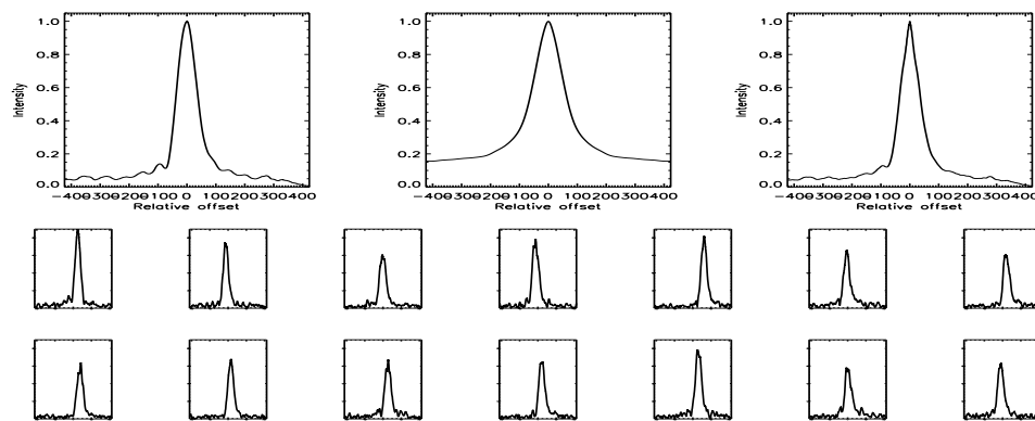
FIGURE B.63: SFP inspection for HD 016160 with S1-E1 on UT 2007/08/15, seq 001
