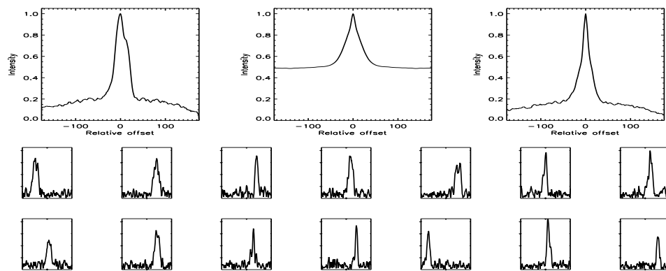
FIGURE B.480: SFP inspection for HD 165401 with S1-E1 on UT 2008/07/05, seq 001
