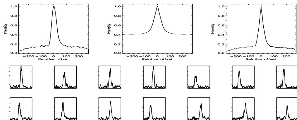
FIGURE B.295: SFP inspection for HD 115404 with S1-E1 on UT 2007/02/06, seq 001
