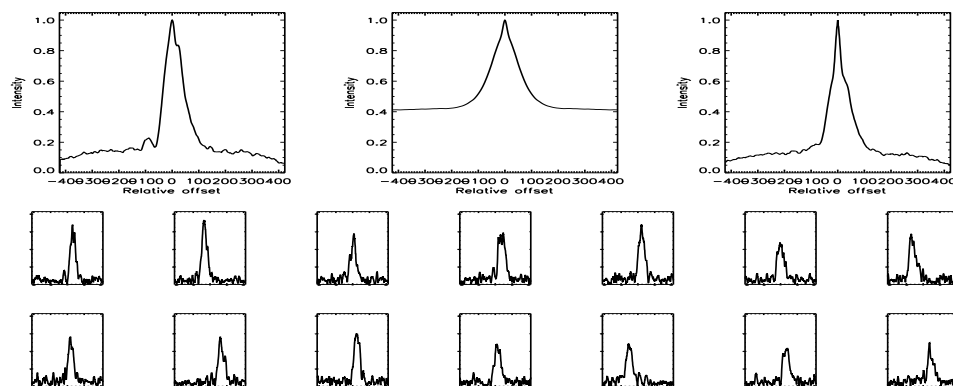
FIGURE B.103: SFP inspection for HD 022879 with S2-E2 on UT 2007/09/27, seq 003
