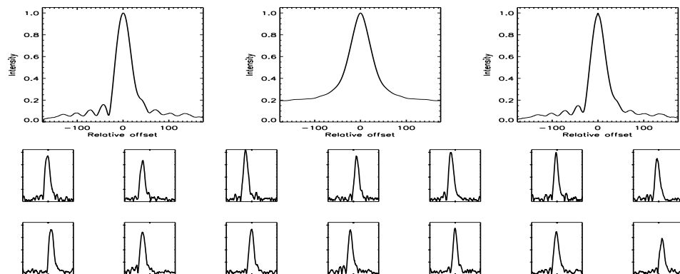
FIGURE B.431: SFP inspection for HD 149806 with S1-W1 on UT 2008/04/14, seq 001
