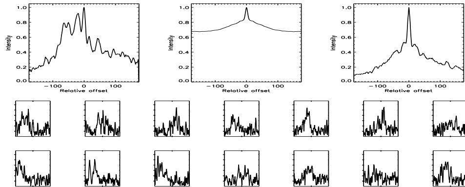
FIGURE B.569: SFP inspection for HD 192263 with S1-W1 on UT 2008/06/22, seq 001
