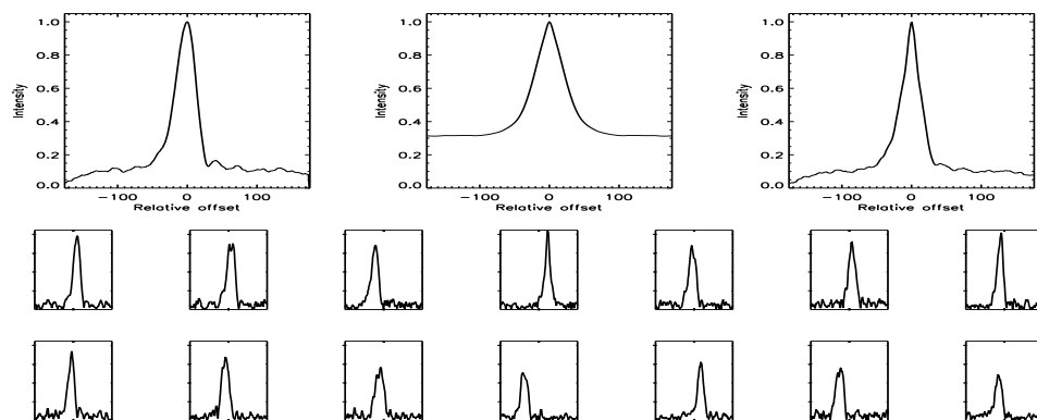
FIGURE B.376: SFP inspection for HD 136202 with S1-E1 on UT 2008/04/13, seq 001
