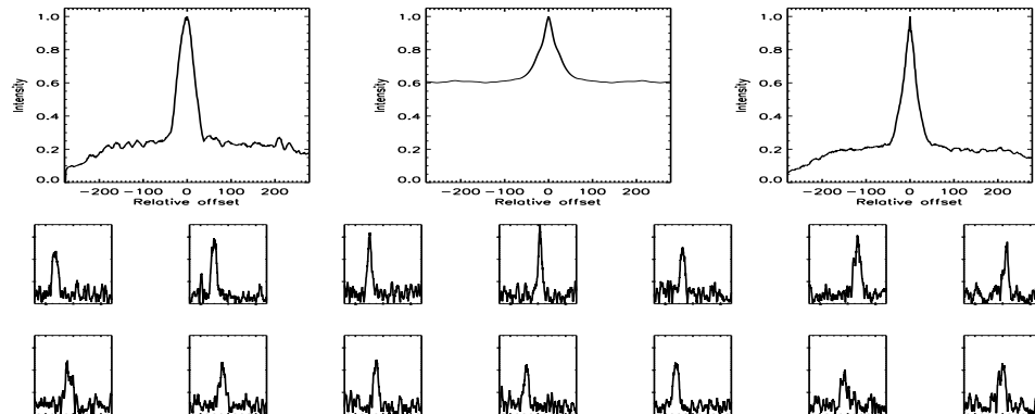
FIGURE B.215: SFP inspection for HD 079969 with S1-E1 on UT 2007/02/06, seq 001
