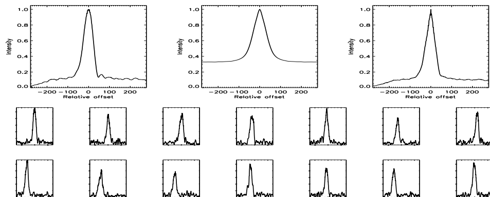
FIGURE B.467: SFP inspection for HD 160346 with S1-E1 on UT 2007/07/22, seq 003
