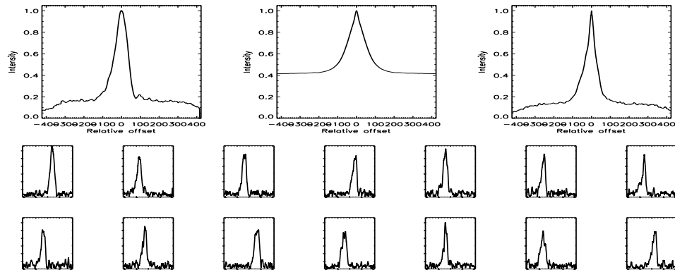
FIGURE B.563: SFP inspection for HD 191785 with S1-W1 on UT 2007/07/24, seq 002
