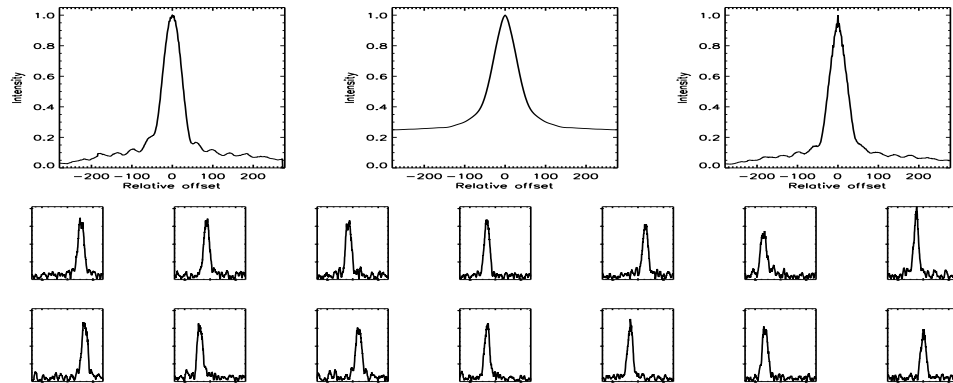
FIGURE B.542: SFP inspection for HD 190067 with S1-E1 on UT 2007/07/22, seq 002
