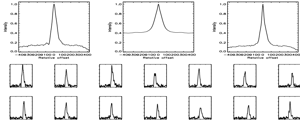
FIGURE B.86: SFP inspection for HD 018757 with S1-W1 on UT 2007/09/16, seq 002
