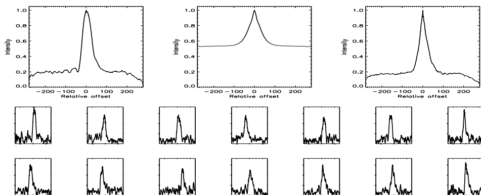
FIGURE B.595: SFP inspection for HD 208313 with S1-E1 on UT 2007/08/14, seq 001
