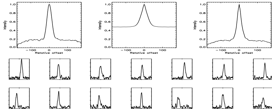
FIGURE B.611: SFP inspection for HD 215152 with S1-W1 on UT 2008/07/07, seq 001
