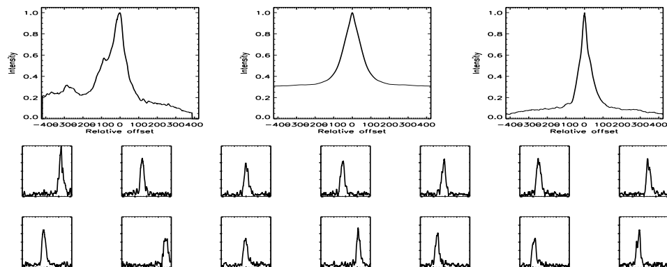
FIGURE B.161: SFP inspection for HD 041593 with S1-E1 on UT 2007/10/31, seq 001
