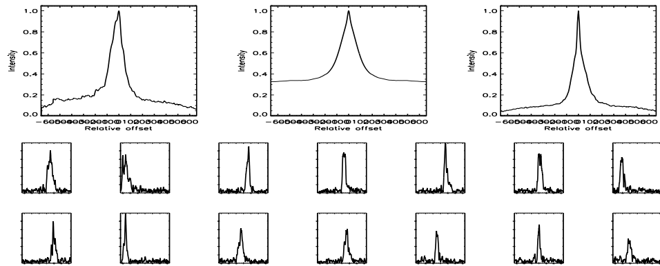
FIGURE B.60: SFP inspection for HD 012051 with S2-W1 on UT 2007/09/17, seq 001
