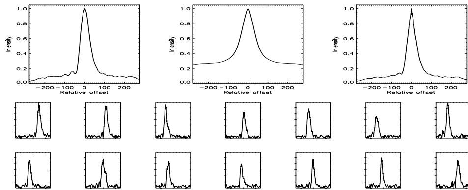
FIGURE B.27: SFP inspection for HD 004628 with S1-W1 on UT 2007/08/14, seq 002
