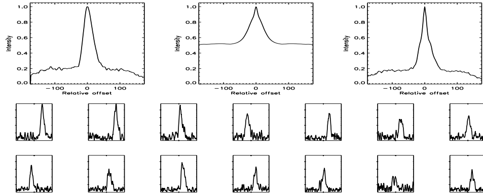
FIGURE B.224: SFP inspection for HD 082443 with S1-E1 on UT 2008/04/13, seq 002
