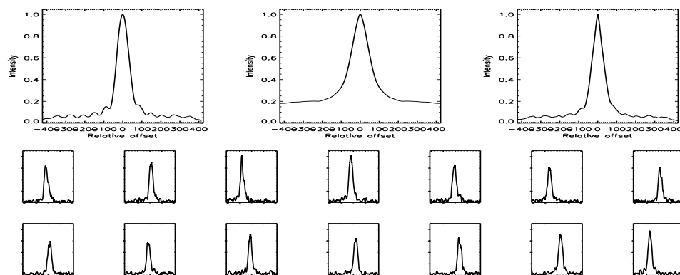
FIGURE B.148: SFP inspection for HD 037394 with S2-E2 on UT 2007/11/19, seq 003
