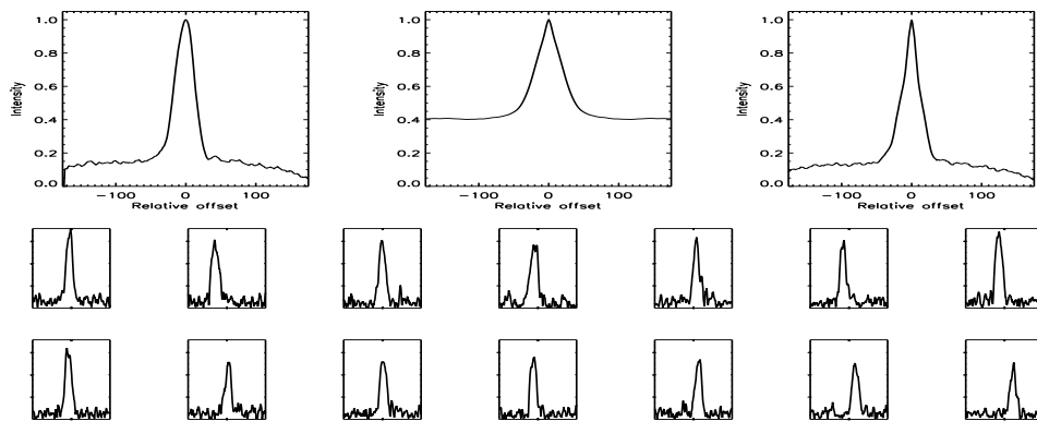
FIGURE B.439: SFP inspection for HD 153557 with S2-W1 on UT 2008/06/24, seq 001
