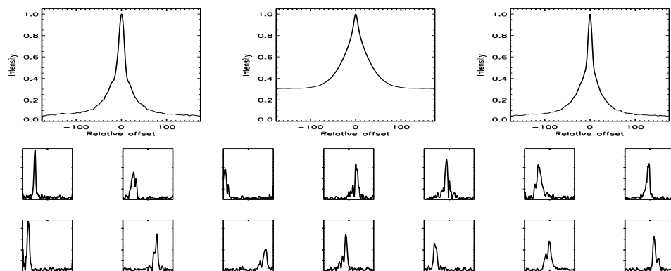
FIGURE B.169: SFP inspection for HD 046588 with S1-W1 on UT 2008/04/26, seq 001
