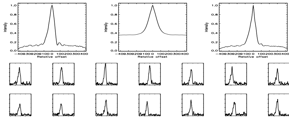
FIGURE B.117: SFP inspection for HD 025457 with S2-E2 on UT 2007/09/27, seq 002
