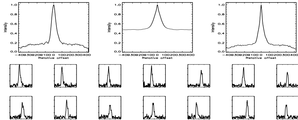
FIGURE B.107: SFP inspection for HD 024409 with S1-W1 on UT 2007/09/16, seq 001
