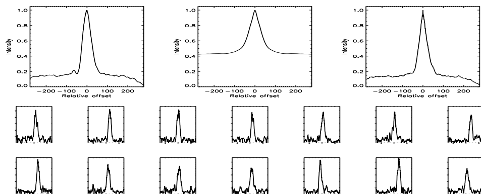
FIGURE B.619: SFP inspection for HD 217813 with S1-E1 on UT 2007/08/14, seq 001
