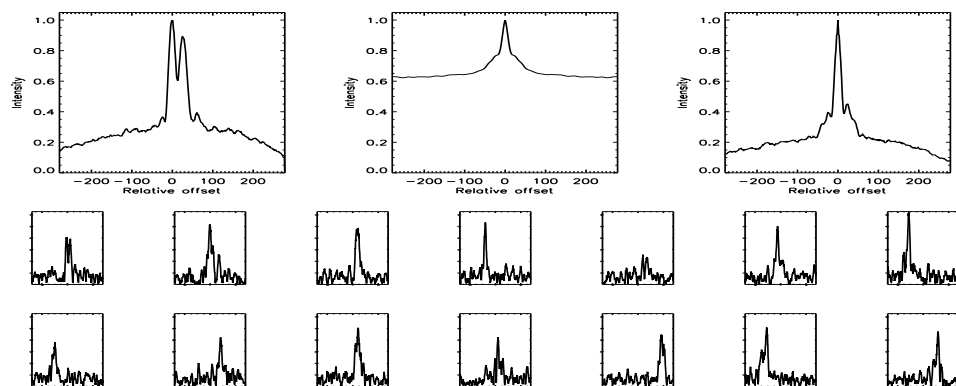
FIGURE B.139: SFP inspection for HD 037008 with S1-E1 on UT 2007/01/25, seq 001
