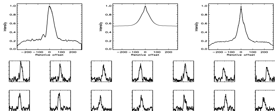
FIGURE B.163: SFP inspection for HD 041593 with S2-E2 on UT 2007/09/26, seq 002
