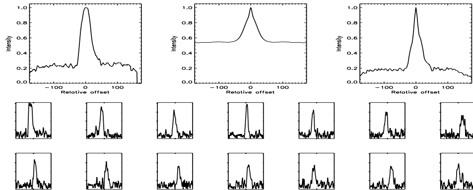
FIGURE B.581: SFP inspection for HD 198425 with S1-E1 on UT 2008/07/23, seq 001
