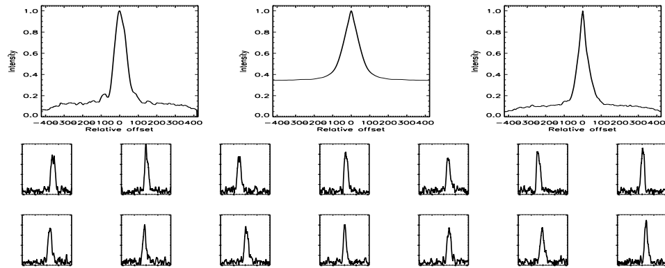
FIGURE B.141: SFP inspection for HD 037008 with S2-E2 on UT 2007/11/19, seq 001
