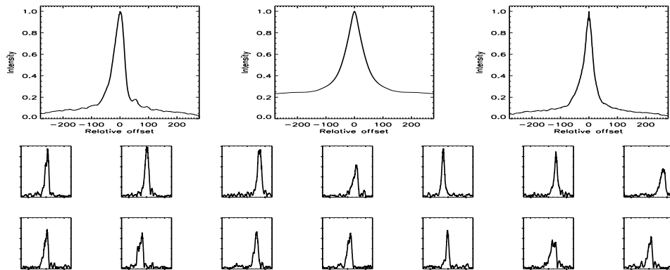
FIGURE B.421: SFP inspection for HD 146233 with S1-E1 on UT 2007/03/08, seq 001
