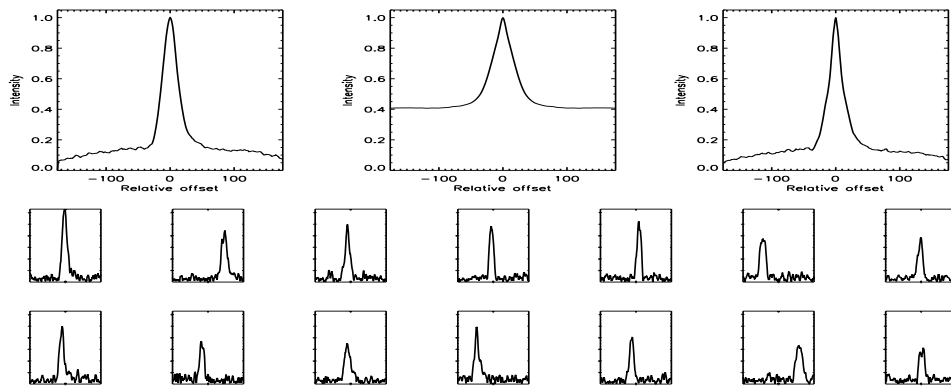
FIGURE B.438: SFP inspection for HD 153557 with S1-W1 on UT 2008/04/12, seq 001
