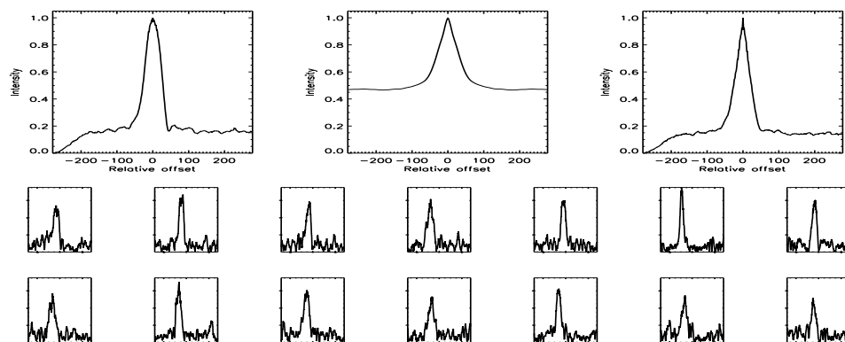
FIGURE B.550: SFP inspection for HD 190470 with S1-W1 on UT 2007/08/17, seq 001
