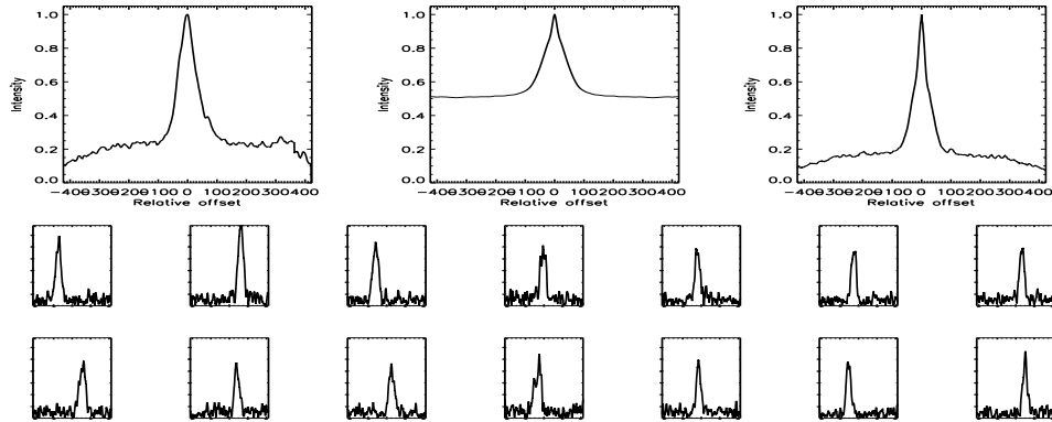
FIGURE B.119: SFP inspection for HD 025665 with S1-W1 on UT 2007/09/16, seq 001
