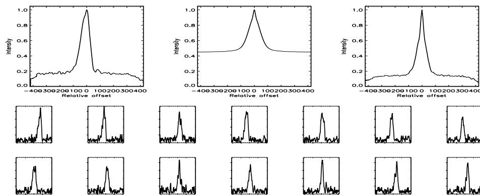
FIGURE B.642: SFP inspection for HD 221851 with S1-E1 on UT 2007/08/18, seq 002
