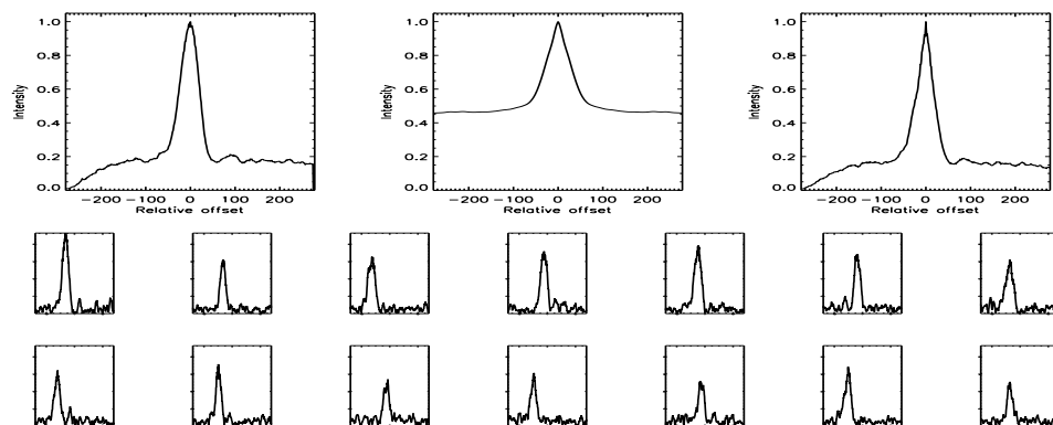
FIGURE B.468: SFP inspection for HD 160346 with S1-W1 on UT 2007/07/22, seq 001
