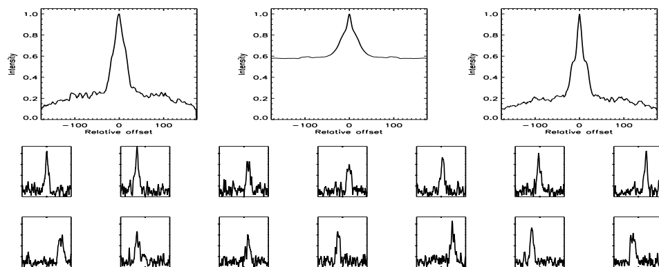
FIGURE B.292: SFP inspection for HD 114783 with S1-E1 on UT 2008/04/13, seq 001
