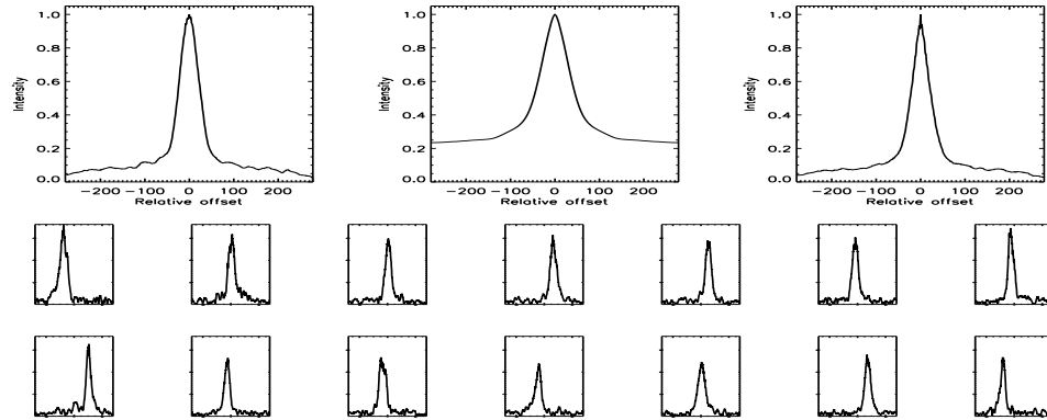
FIGURE B.26: SFP inspection for HD 004628 with S1-E1 on UT 2007/08/14, seq 001
