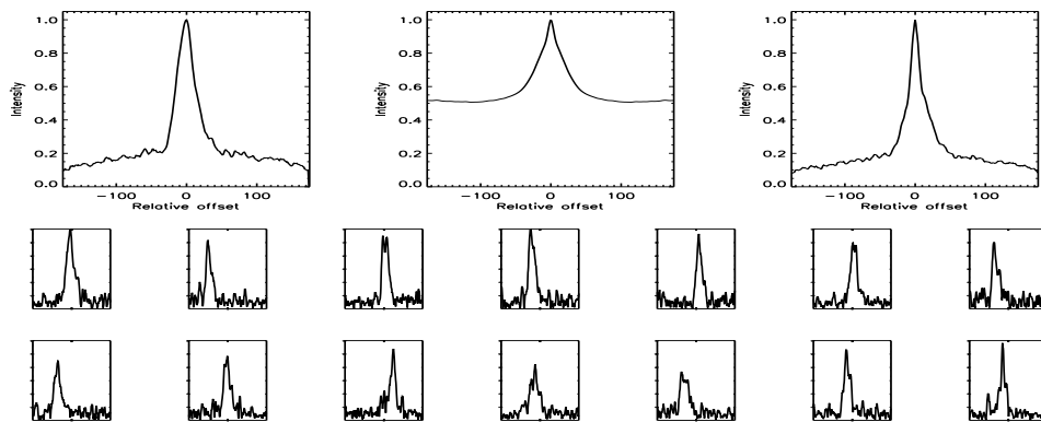
FIGURE B.10: SFP inspection for HD 001562 with S1-W1 on UT 2008/07/08, seq 001
