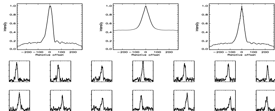
FIGURE B.604: SFP inspection for HD 210667 with S1-E1 on UT 2007/07/26, seq 001
