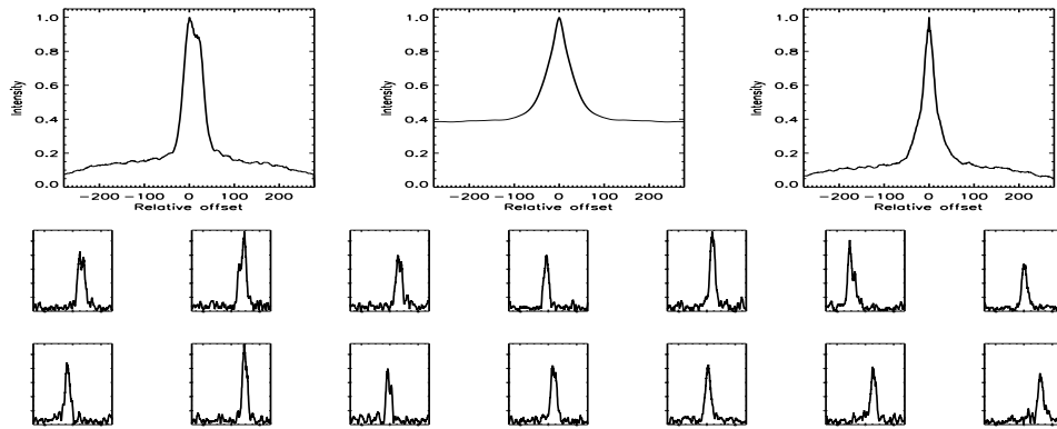
FIGURE B.420: SFP inspection for HD 145675 with S1-W1 on UT 2007/04/24, seq 001
