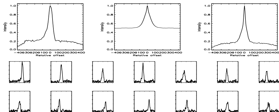
FIGURE B.615: SFP inspection for HD 216520 with S1-W1 on UT 2007/09/16, seq 001
