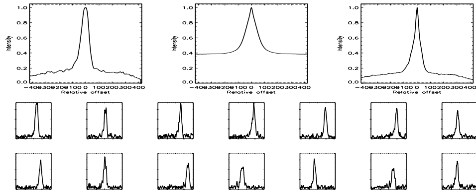
FIGURE B.41: SFP inspection for HD 007924 with S1-W1 on UT 2007/09/16, seq 001
