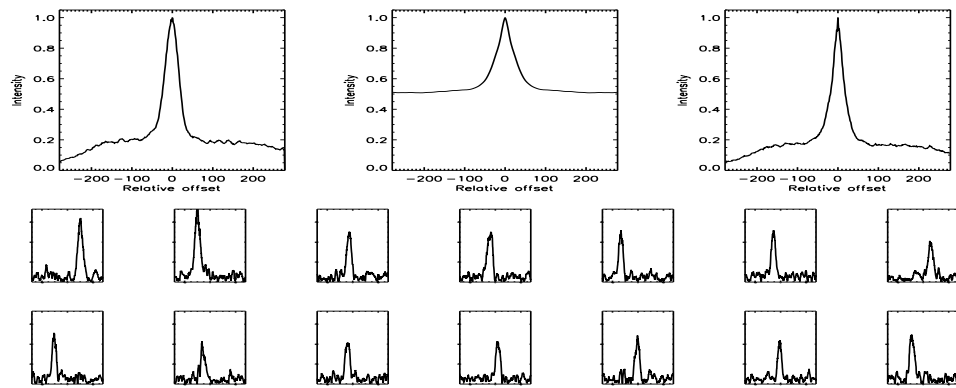
FIGURE B.177: SFP inspection for HD 054371 with S1-E1 on UT 2007/02/04, seq 001
