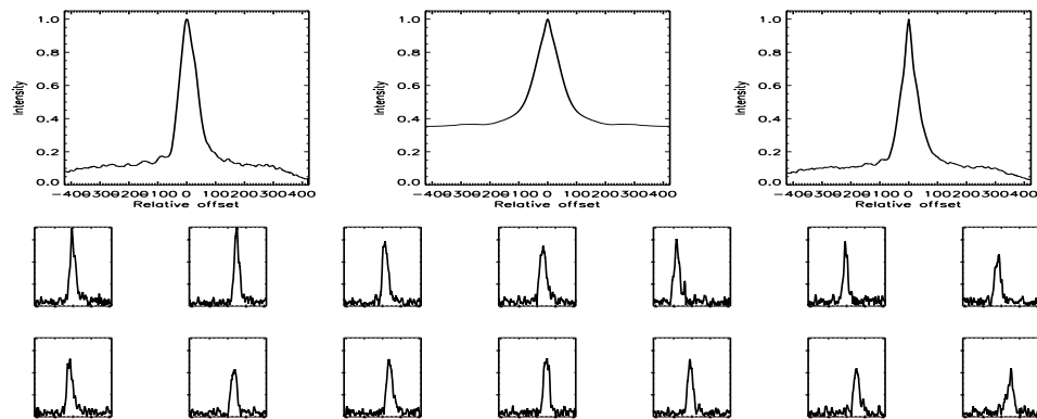
FIGURE B.108: SFP inspection for HD 024409 with S2-E1 on UT 2007/08/20, seq 001
