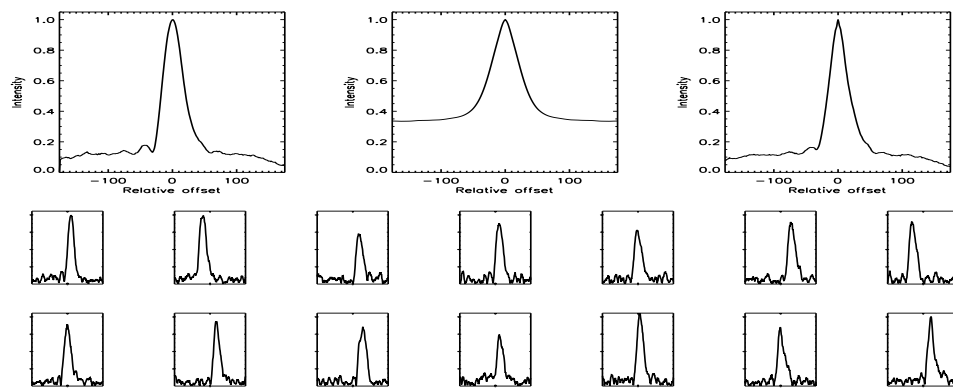
FIGURE B.624: SFP inspection for HD 218868 with S1-E1 on UT 2008/07/21, seq 001
