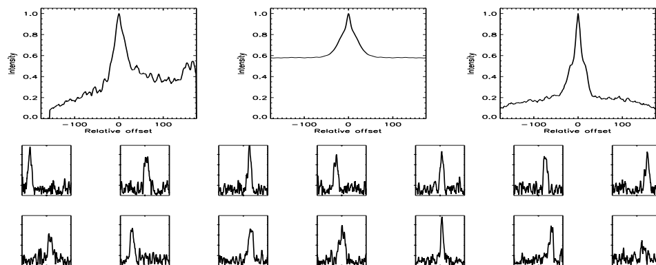
FIGURE B.459: SFP inspection for HD 159062 with S1-E1 on UT 2008/06/25, seq 001
