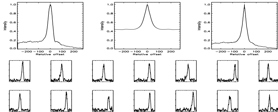
FIGURE B.170: SFP inspection for HD 051419 with S1-E1 on UT 2007/02/05, seq 002
