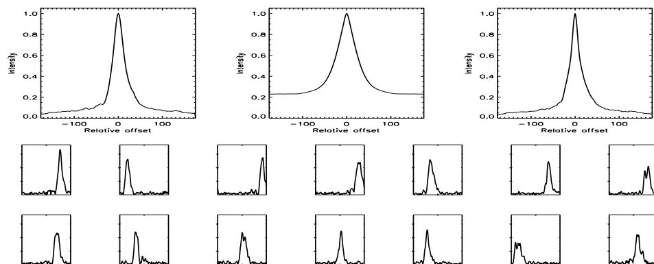
FIGURE B.423: SFP inspection for HD 146233 with S1-E1 on UT 2008/06/23, seq 001
