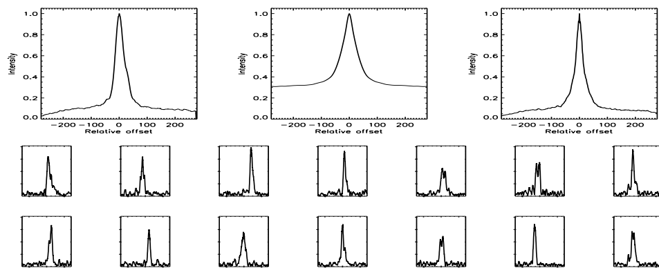
FIGURE B.201: SFP inspection for HD 068255 with S1-E1 on UT 2007/02/25, seq 002
