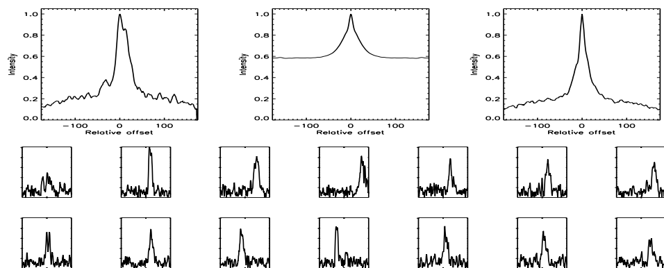
FIGURE B.490: SFP inspection for HD 175742 with S1-E1 on UT 2008/06/21, seq 001
