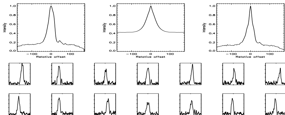
FIGURE B.504: SFP inspection for HD 176377 with S2-W1 on UT 2008/06/24, seq 001
