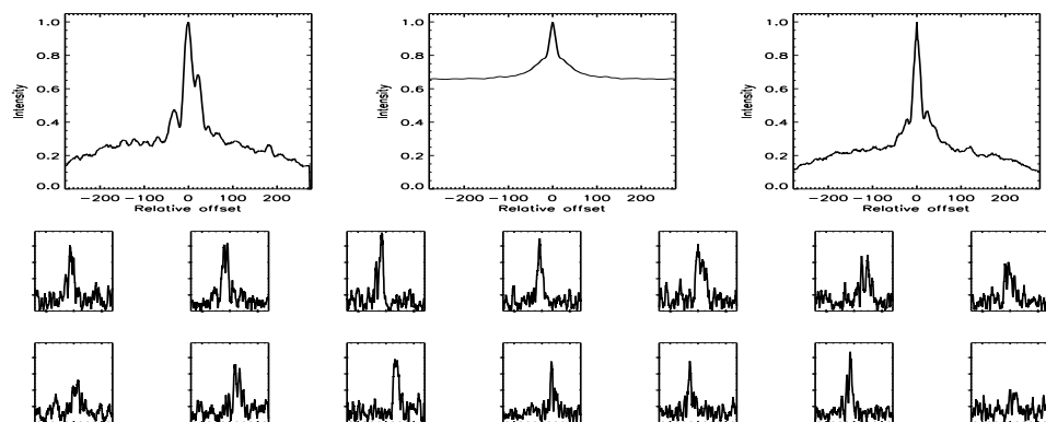
FIGURE B.145: SFP inspection for HD 037394 with S1-E1 on UT 2007/01/26, seq 002
