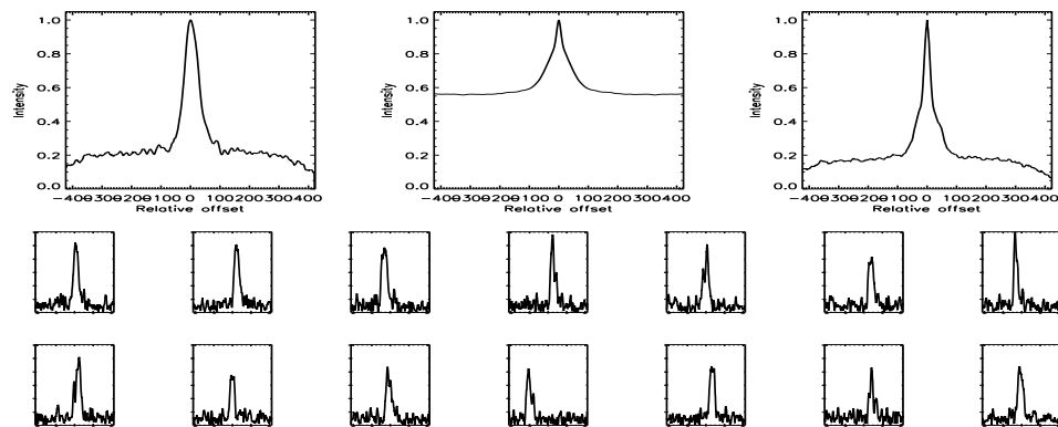
FIGURE B.118: SFP inspection for HD 025665 with S1-E1 on UT 2007/09/16, seq 002
