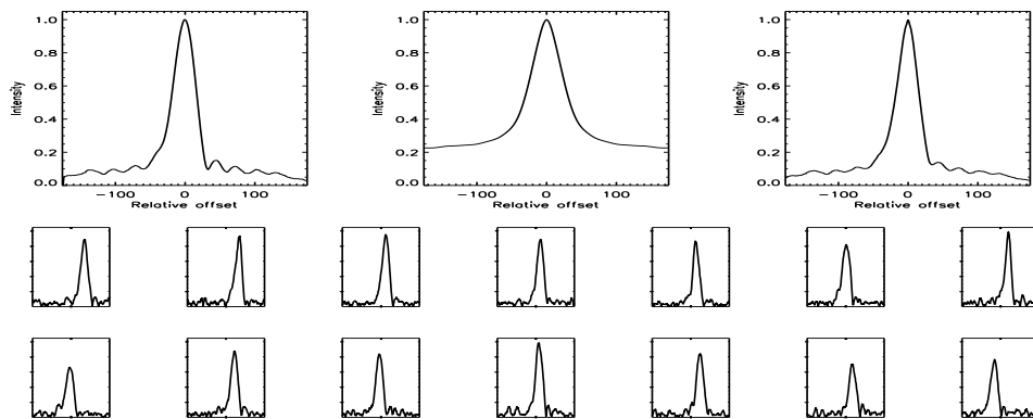
FIGURE B.484: SFP inspection for HD 165401 with S1-W1 on UT 2008/07/07, seq 001
