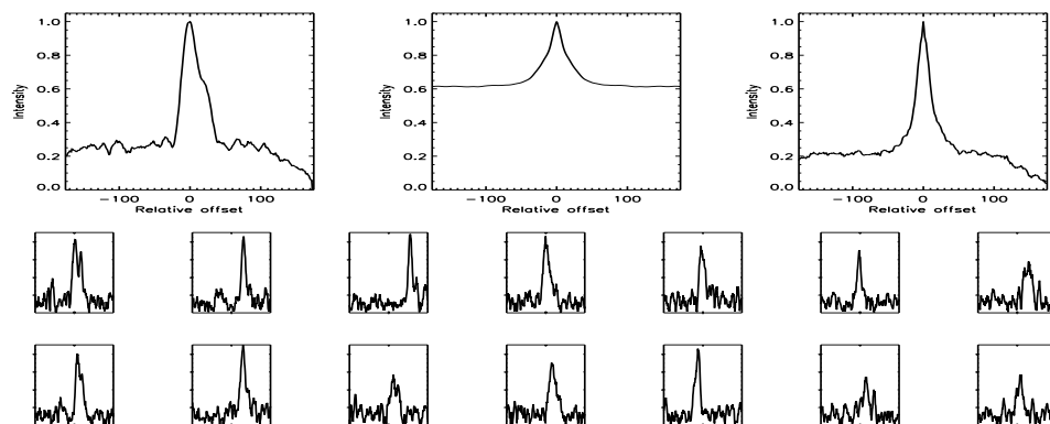
FIGURE B.198: SFP inspection for HD 068017 with S1-E1 on UT 2008/04/13, seq 001
