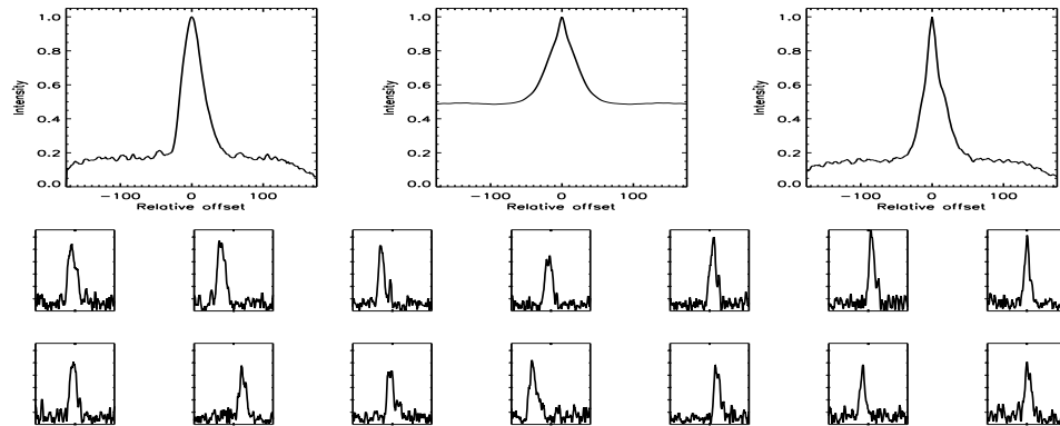
FIGURE B.308: SFP inspection for HD 116956 with S2-W1 on UT 2008/06/24, seq 001
