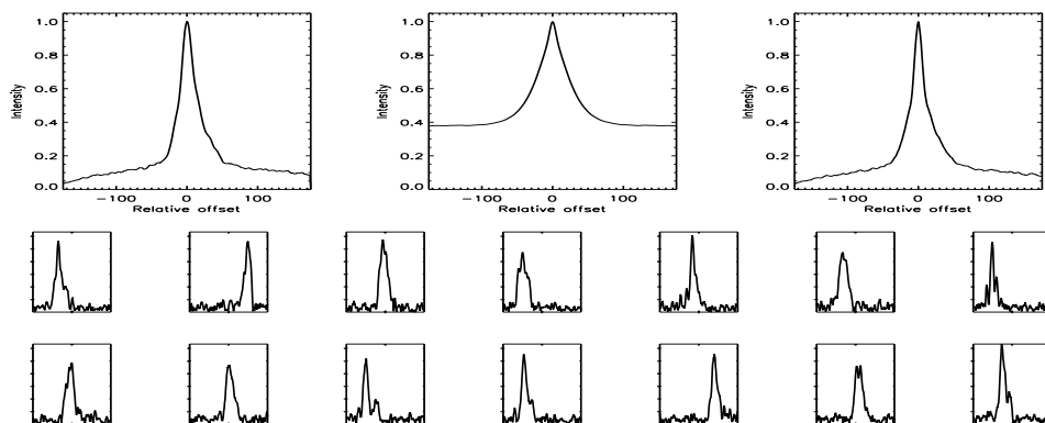
FIGURE B.405: SFP inspection for HD 139777 with S1-W1 on UT 2008/04/26, seq 001
