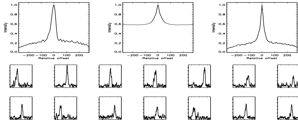
FIGURE B.398: SFP inspection for HD 139341 with E1-W1 on UT 2007/04/26, seq 002
