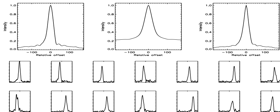
FIGURE B.266: SFP inspection for HD 099492 with S1-W1 on UT 2008/04/15, seq 001
