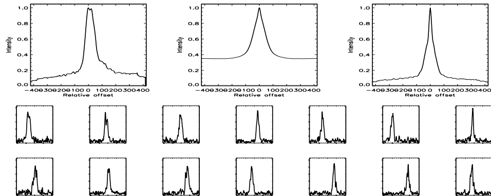
FIGURE B.113: SFP inspection for HD 025457 with S1-E1 on UT 2007/10/31, seq 001
