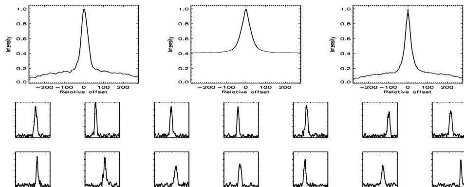
FIGURE B.440: SFP inspection for HD 154345 with E1-W1 on UT 2007/04/26, seq 001
