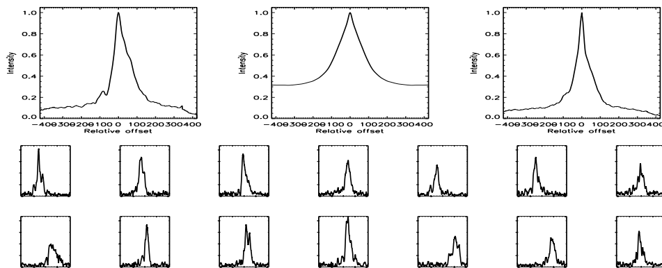
FIGURE B.136: SFP inspection for HD 032923 with S2-E2 on UT 2007/09/27, seq 001
