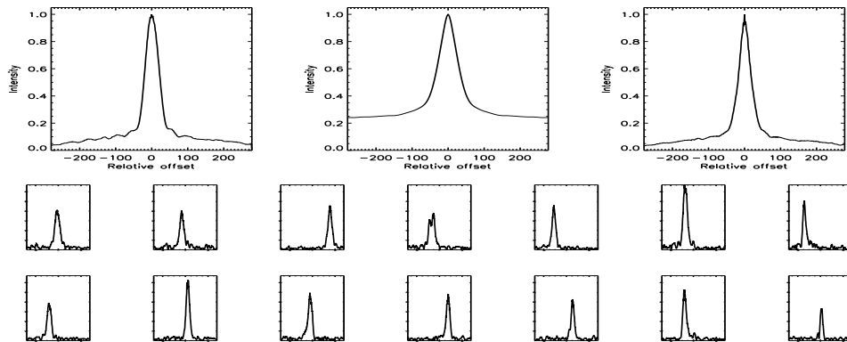
FIGURE B.361: SFP inspection for HD 132254 with S1-W1 on UT 2007/04/24, seq 001
