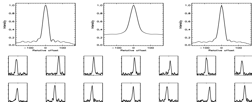
FIGURE B.381: SFP inspection for HD 136713 with S1-W1 on UT 2008/04/14, seq 001
