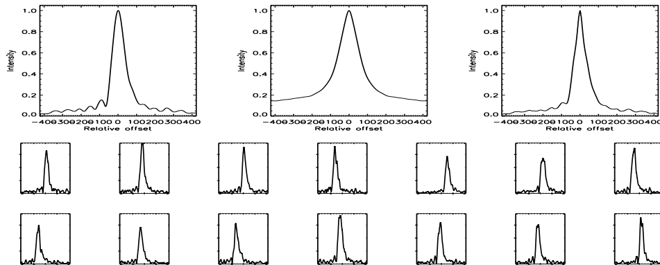
FIGURE B.134: SFP inspection for HD 032923 with S1-W1 on UT 2007/10/31, seq 002
