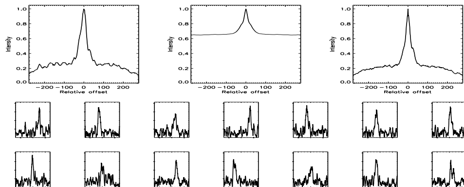
FIGURE B.608: SFP inspection for HD 211472 with S1-E1 on UT 2007/07/28, seq 001
