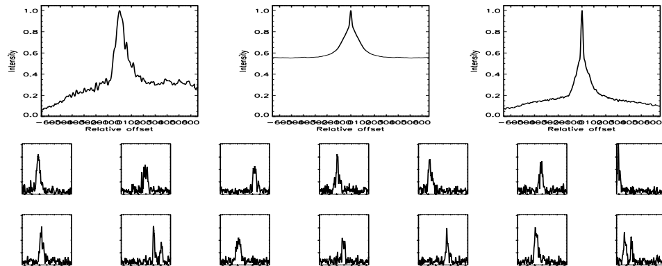
FIGURE B.47: SFP inspection for HD 010008 with S2-W1 on UT 2007/09/17, seq 001
