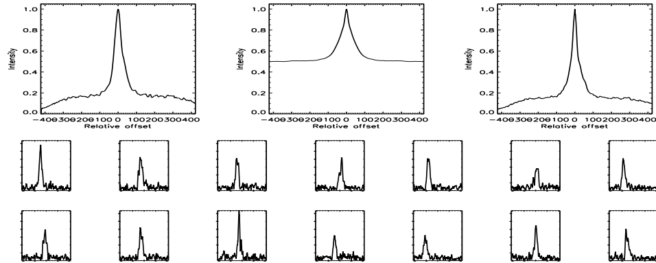
FIGURE B.89: SFP inspection for HD 018803 with S2-W1 on UT 2007/09/17, seq 001
