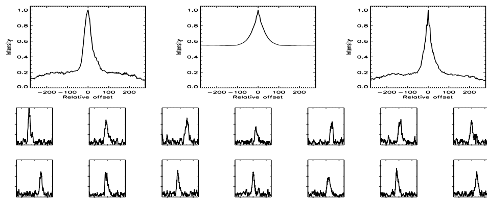
FIGURE B.648: SFP inspection for HD 222404 with S1-E1 on UT 2007/09/16, seq 003
