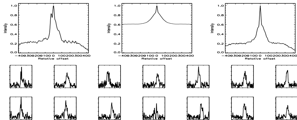
FIGURE B.112: SFP inspection for HD 024496 with S2-E2 on UT 2007/09/27, seq 001
