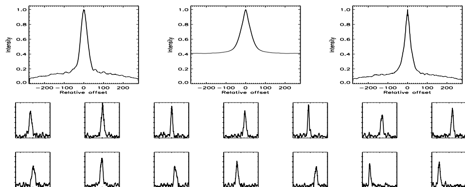
FIGURE B.531: SFP inspection for HD 185414 with S1-E1 on UT 2007/04/14, seq 001
