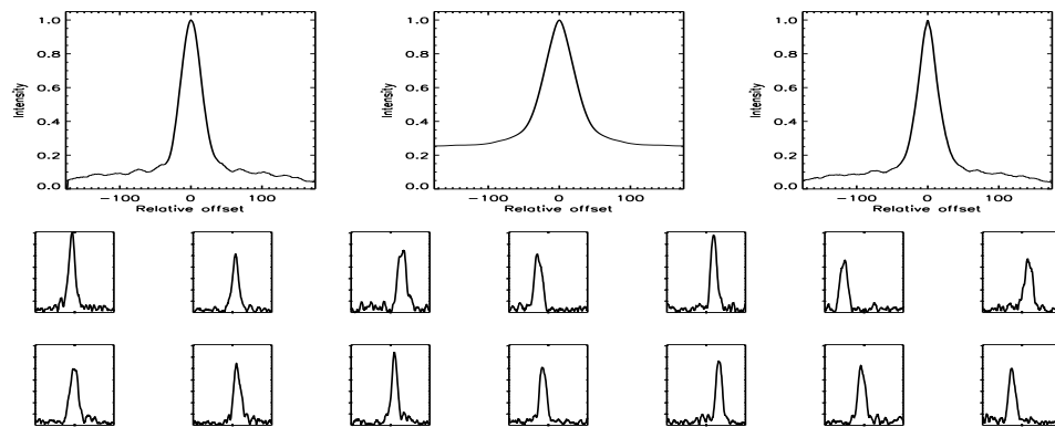
FIGURE B.571: SFP inspection for HD 192263 with S1-W1 on UT 2008/07/07, seq 002
