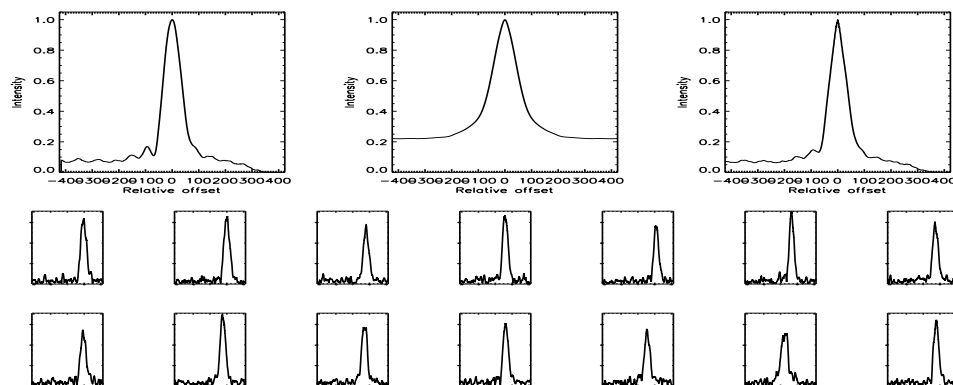
FIGURE B.618: SFP inspection for HD 217813 with S1-E1 on UT 2007/07/22, seq 001
