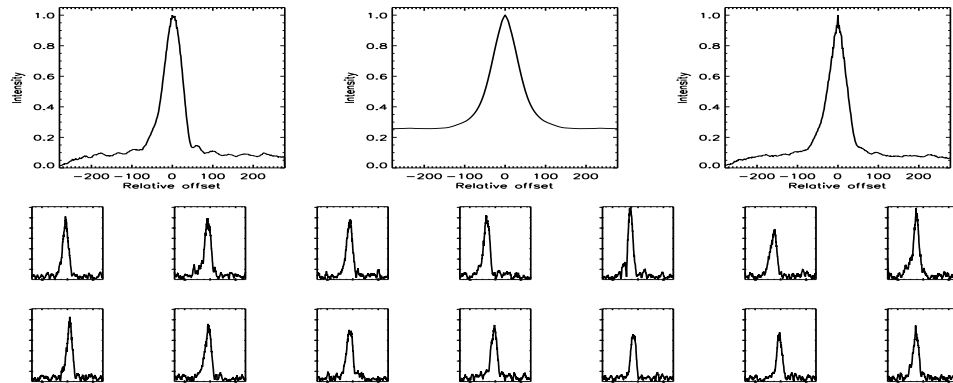
FIGURE B.650: SFP inspection for HD 222404 with S1-W1 on UT 2007/09/16, seq 002
