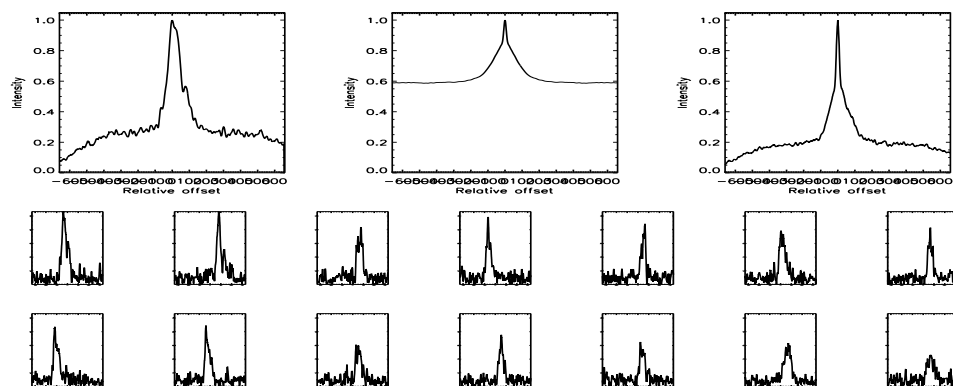
FIGURE B.127: SFP inspection for HD 029883 with S2-W1 on UT 2007/09/17, seq 001
