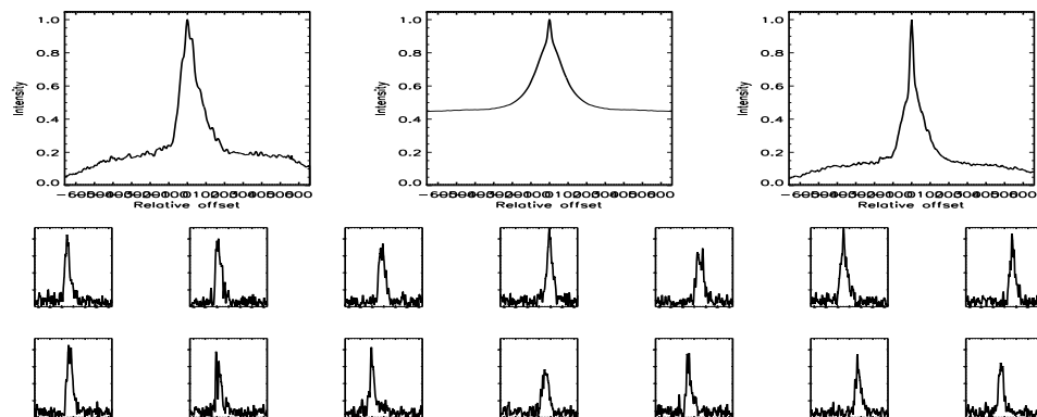
FIGURE B.82: SFP inspection for HD 018143 with S2-W1 on UT 2007/09/17, seq 001
