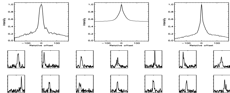
FIGURE B.178: SFP inspection for HD 054371 with S1-E1 on UT 2008/04/25, seq 001
