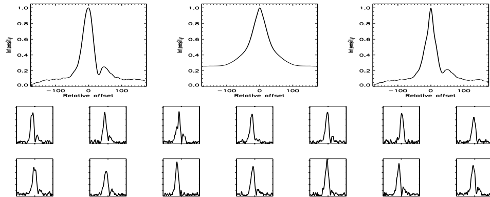
FIGURE B.347: SFP inspection for HD 128642 with S2-W1 on UT 2008/06/24, seq 001
