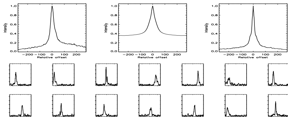
FIGURE B.321: SFP inspection for HD 124850 with S1-E1 on UT 2007/03/23, seq 001
