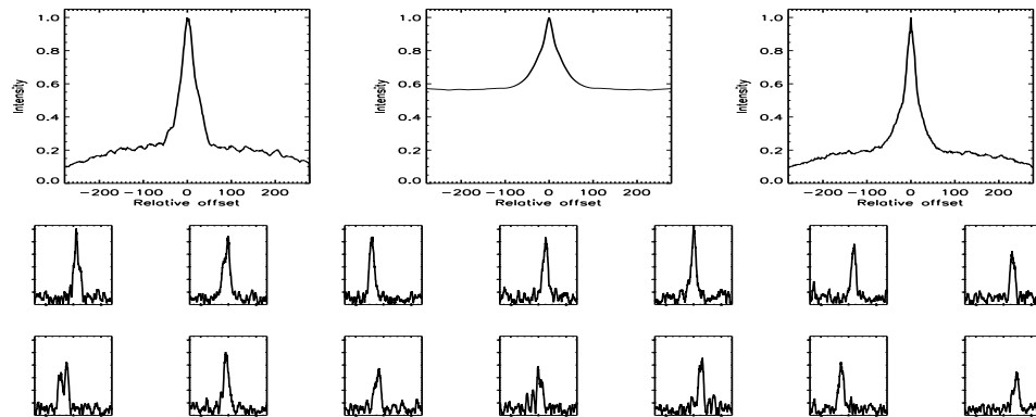
FIGURE B.184: SFP inspection for HD 055575 with S2-E2 on UT 2007/11/20, seq 001
