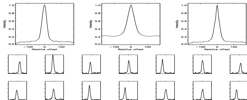
FIGURE B.652: SFP inspection for HD 222404 with S2-W1 on UT 2008/06/24, seq 001
