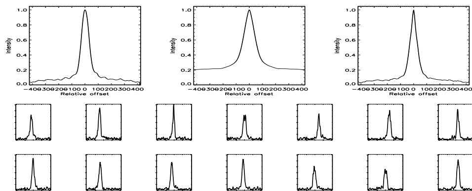
FIGURE B.55: SFP inspection for HD 010780 with S2-E1 on UT 2007/08/20, seq 002
