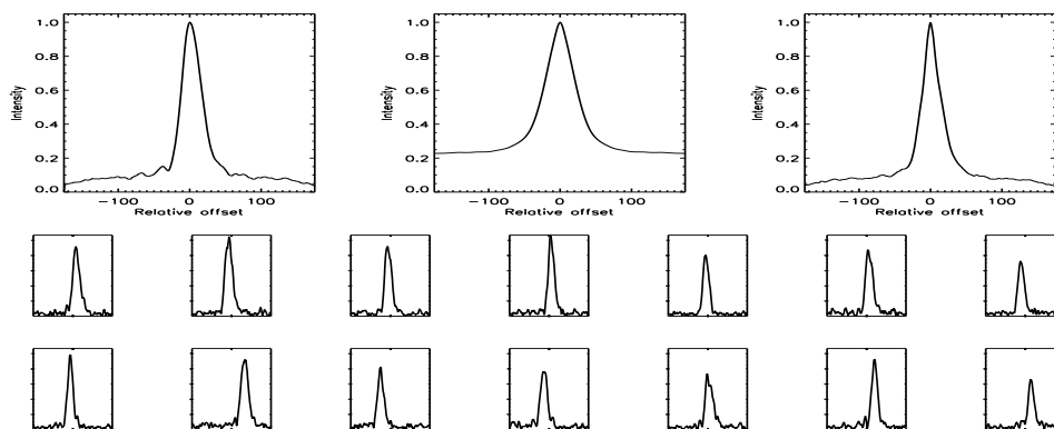
FIGURE B.430: SFP inspection for HD 149806 with S1-W1 on UT 2008/04/13, seq 001
