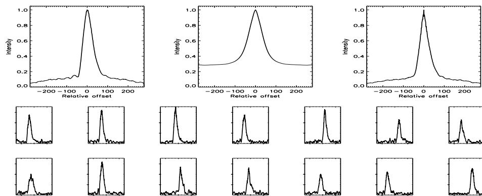
FIGURE B.246: SFP inspection for HD 098230 with S1-E1 on UT 2007/02/06, seq 001
