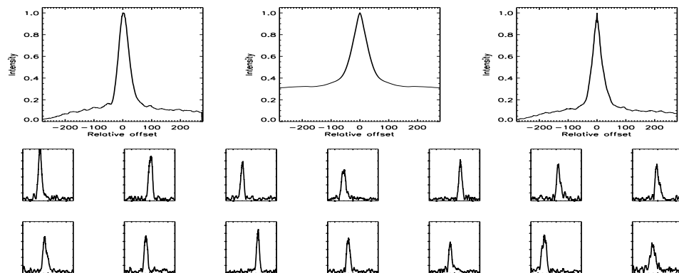
FIGURE B.443: SFP inspection for HD 154345 with S1-W1 on UT 2007/04/17, seq 002
