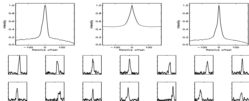
FIGURE B.433: SFP inspection for HD 151541 with S1-W1 on UT 2008/04/26, seq 001
