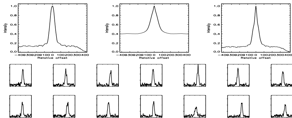
FIGURE B.138: SFP inspection for HD 035112 with S1-W1 on UT 2007/10/31, seq 002
