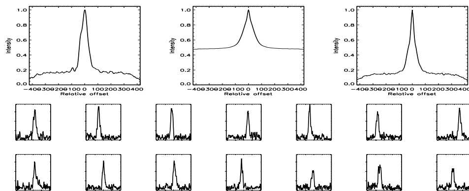
FIGURE B.175: SFP inspection for HD 051866 with S2-E2 on UT 2007/11/19, seq 001
