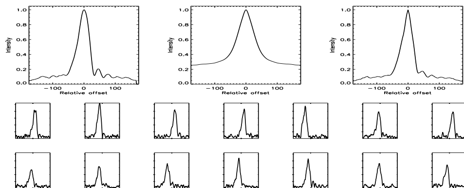
FIGURE B.394: SFP inspection for HD 137778 with S1-W1 on UT 2008/07/07, seq 001
