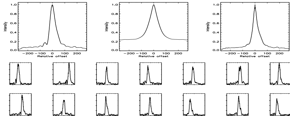
FIGURE B.248: SFP inspection for HD 098230 with S1-E1 on UT 2007/03/08, seq 002
