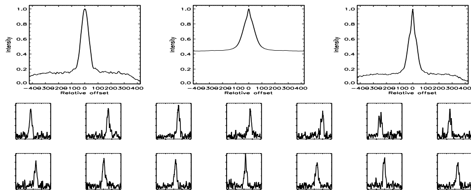
FIGURE B.109: SFP inspection for HD 024496 with S1-E1 on UT 2007/10/31, seq 001
