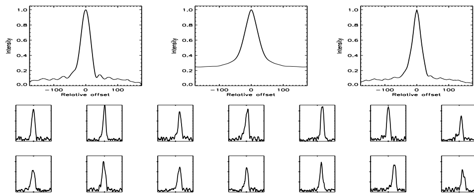
FIGURE B.264: SFP inspection for HD 099491 with S1-E1 on UT 2008/04/14, seq 002
