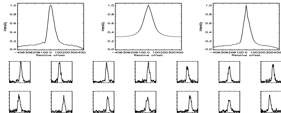
FIGURE B.100: SFP inspection for HD 022049 with S2-E2 on UT 2007/09/27, seq 002
