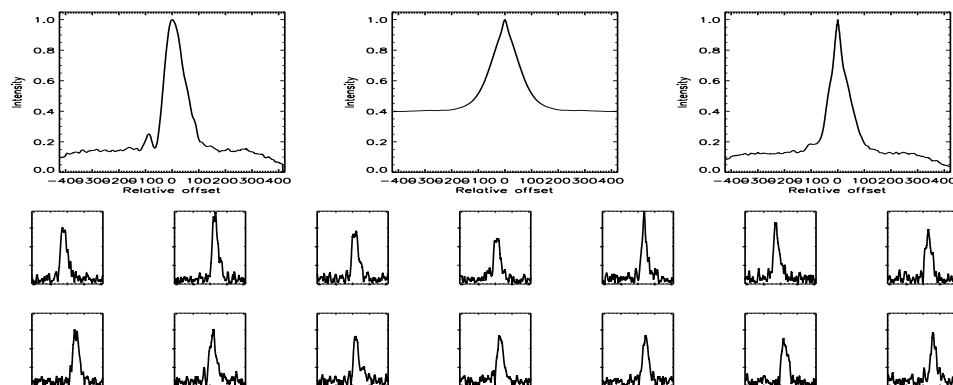
FIGURE B.102: SFP inspection for HD 022879 with S2-E2 on UT 2007/09/27, seq 002
