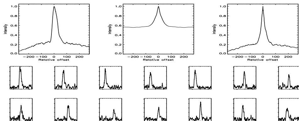
FIGURE B.313: SFP inspection for HD 121560 with S1-E1 on UT 2007/02/05, seq 002
