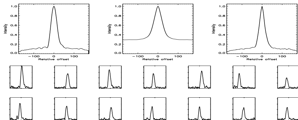
FIGURE B.601: SFP inspection for HD 210277 with S1-W1 on UT 2008/07/07, seq 001
