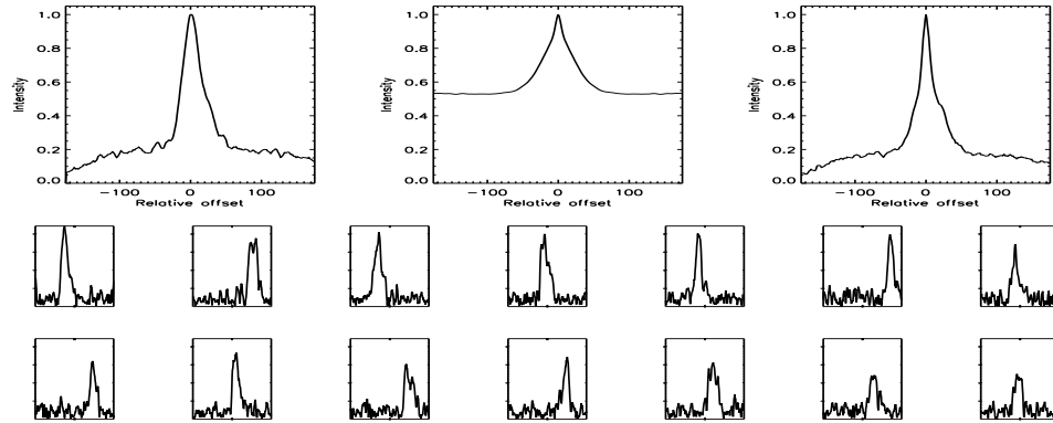
FIGURE B.236: SFP inspection for HD 090343 with S1-E1 on UT 2008/06/25, seq 001
