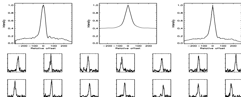
FIGURE B.545: SFP inspection for HD 190404 with S1-E1 on UT 2007/07/24, seq 001
