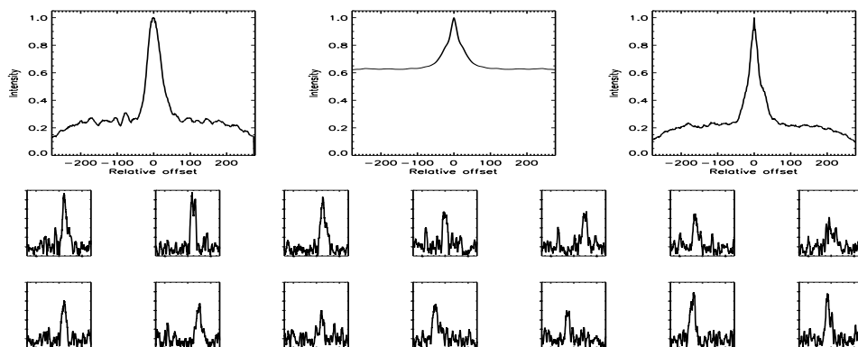
FIGURE B.594: SFP inspection for HD 208313 with S1-E1 on UT 2007/07/25, seq 001
