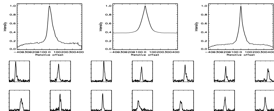
FIGURE B.64: SFP inspection for HD 016160 with S2-E2 on UT 2007/09/18, seq 001
