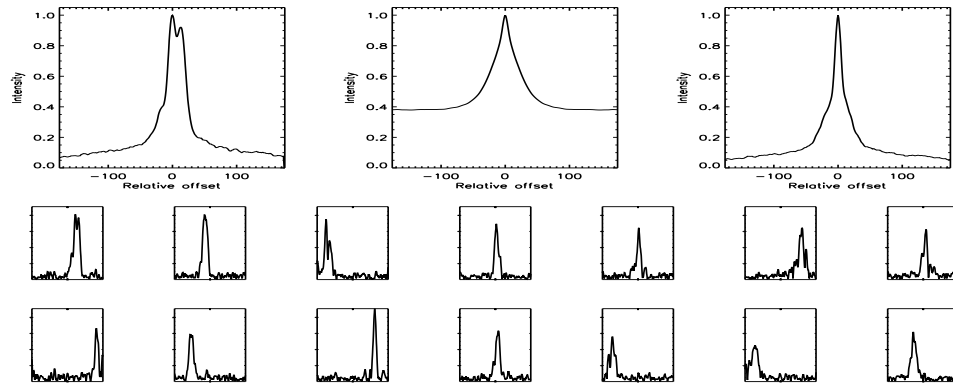
FIGURE B.221: SFP inspection for HD 080715 with S1-W1 on UT 2008/04/26, seq 001
