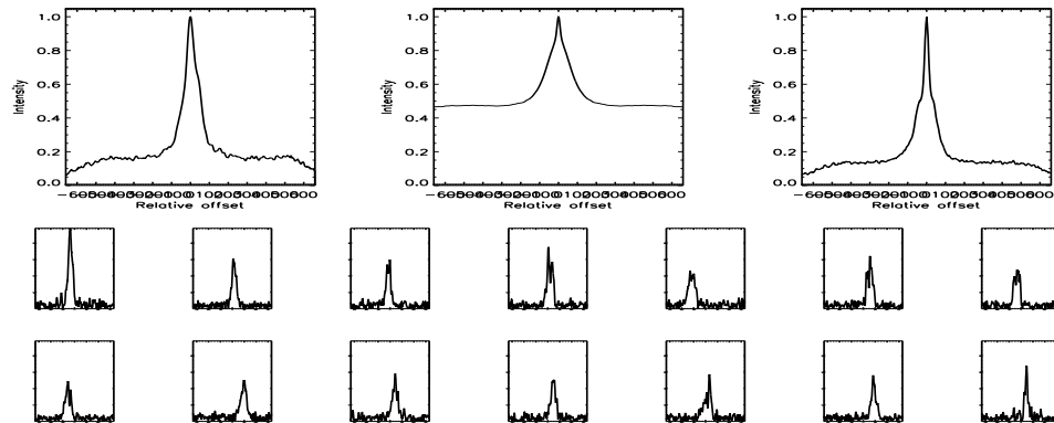
FIGURE B.641: SFP inspection for HD 221354 with S2-E1 on UT 2007/08/20, seq 002
