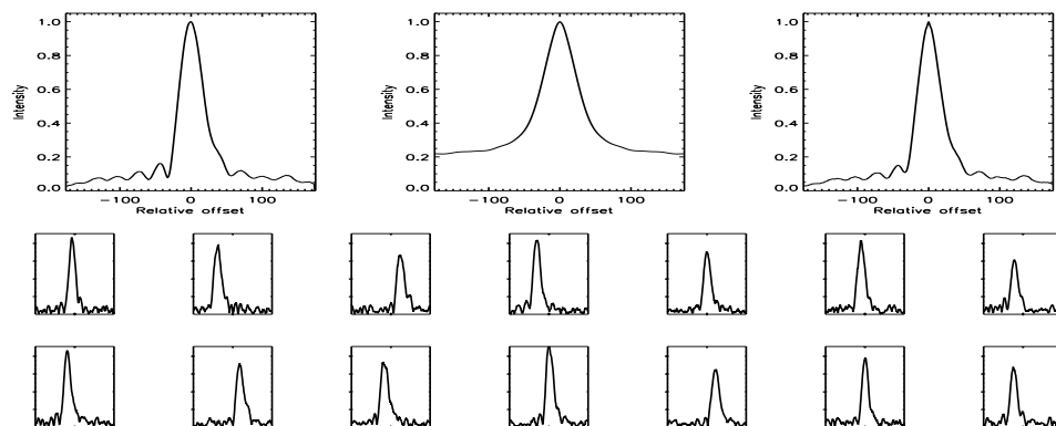
FIGURE B.411: SFP inspection for HD 141272 with S1-W1 on UT 2008/04/14, seq 001
