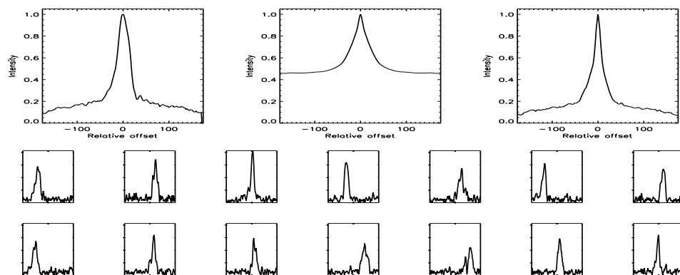
FIGURE B.469: SFP inspection for HD 161198 with S1-E1 on UT 2008/04/25, seq 001
