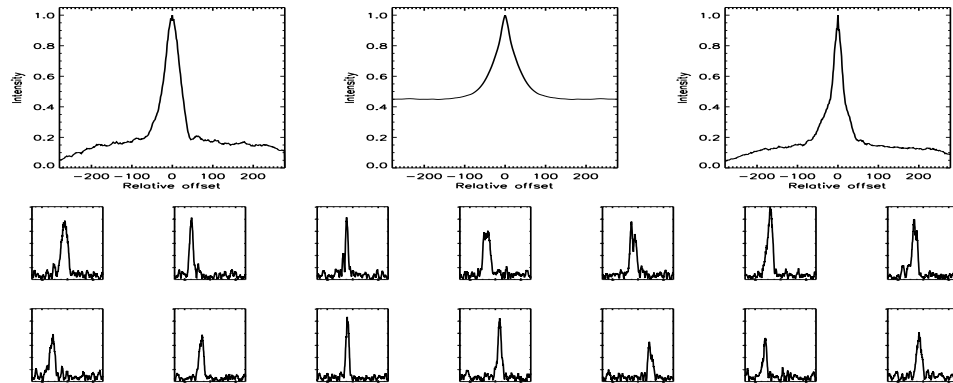
FIGURE B.281: SFP inspection for HD 108954 with S1-E1 on UT 2007/04/11, seq 002
