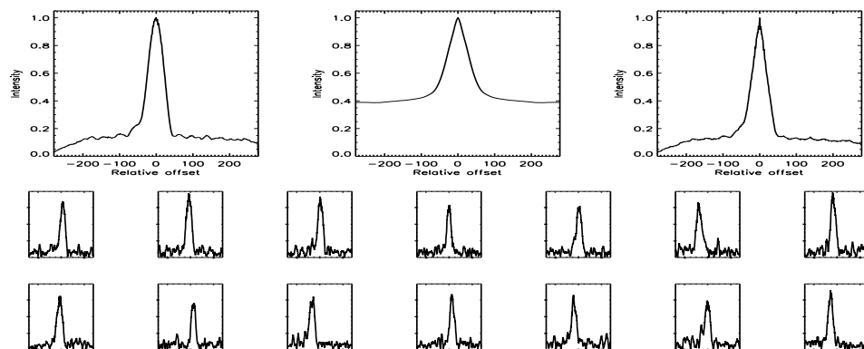
FIGURE B.621: SFP inspection for HD 218868 with S1-E1 on UT 2007/07/26, seq 001
