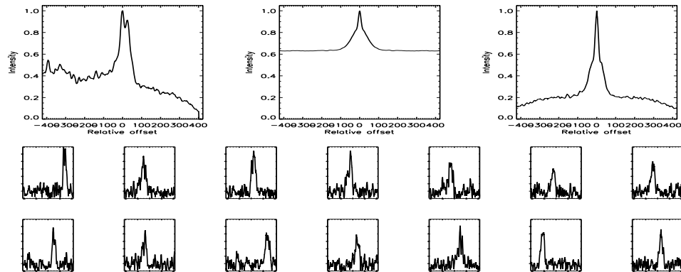
FIGURE B.137: SFP inspection for HD 035112 with S1-E1 on UT 2007/10/31, seq 001
