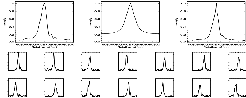
FIGURE B.92: SFP inspection for HD 019994 with S2-E2 on UT 2007/09/27, seq 001
