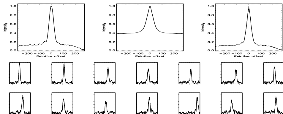
FIGURE B.463: SFP inspection for HD 159222 with S1-E1 on UT 2007/05/17, seq 002
