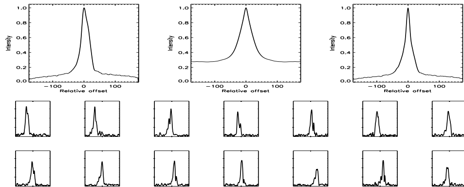
FIGURE B.448: SFP inspection for HD 157347 with S1-E1 on UT 2008/04/25, seq 001
