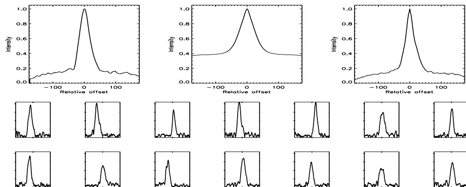
FIGURE B.599: SFP inspection for HD 210277 with S1-E1 on UT 2008/07/06, seq 002
