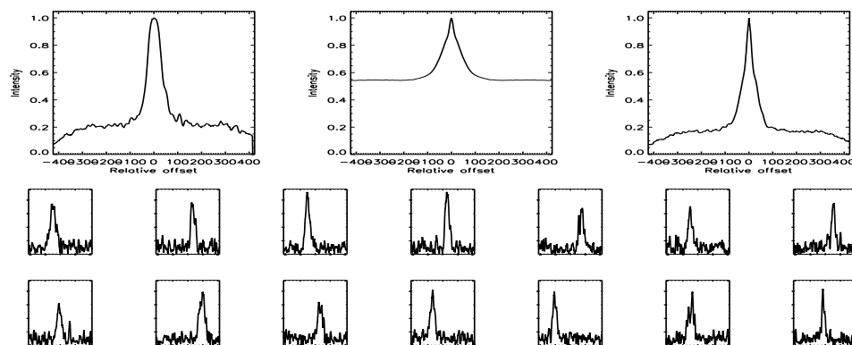
FIGURE B.622: SFP inspection for HD 218868 with S1-E1 on UT 2007/07/28, seq 002
