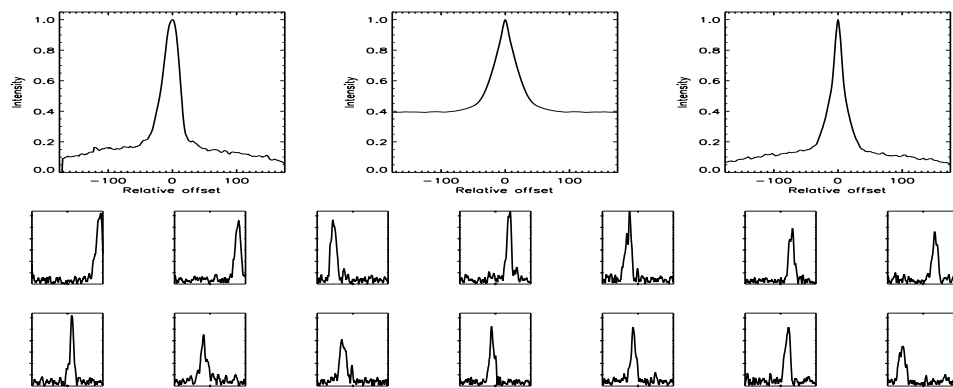
FIGURE B.243: SFP inspection for HD 097334 with S1-W1 on UT 2008/04/12, seq 001
