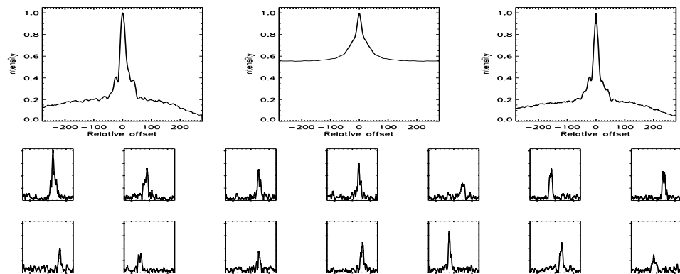
FIGURE B.181: SFP inspection for HD 055575 with S1-E1 on UT 2007/01/26, seq 001
