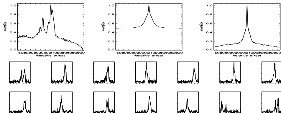
FIGURE B.101: SFP inspection for HD 022879 with S1-E1 on UT 2007/11/01, seq 001
