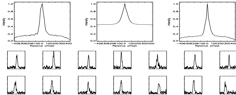
FIGURE B.123: SFP inspection for HD 026923 with S1-E1 on UT 2007/10/31, seq 001
