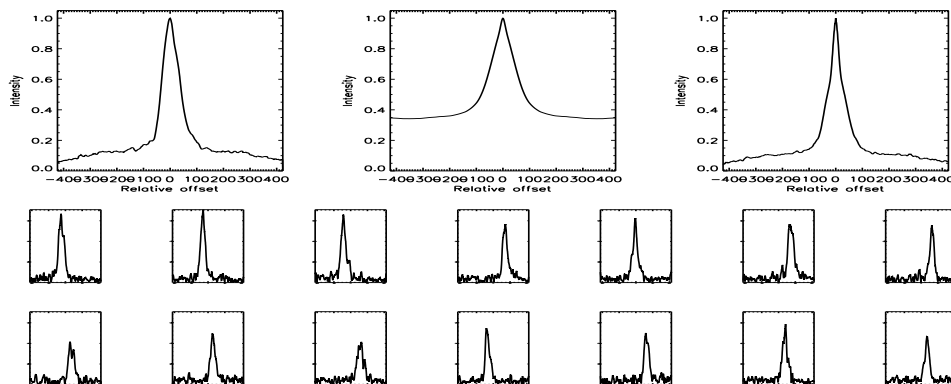
FIGURE B.527: SFP inspection for HD 185144 with S1-E1 on UT 2007/09/16, seq 002
