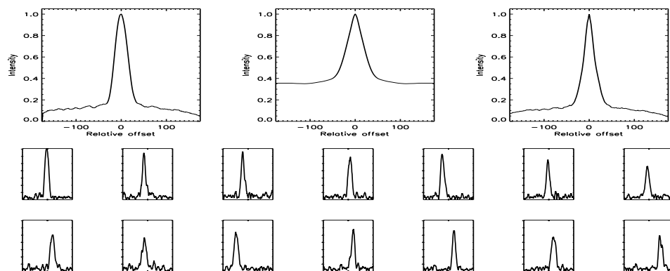
FIGURE B.289: SFP inspection for HD 112758 with S1-W1 on UT 2008/04/15, seq 001
