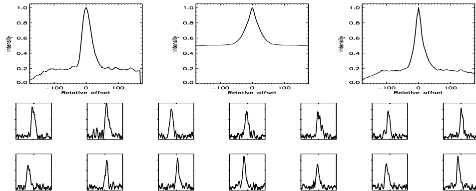
FIGURE B.245: SFP inspection for HD 097658 with S1-E1 on UT 2008/04/14, seq 001
