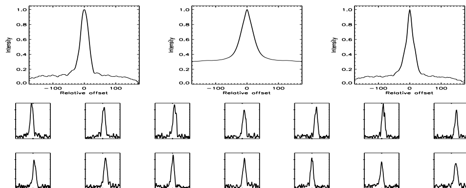
FIGURE B.294: SFP inspection for HD 114783 with S1-W1 on UT 2008/04/13, seq 002
