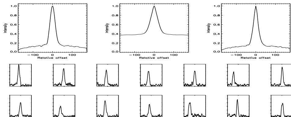
FIGURE B.465: SFP inspection for HD 159222 with S1-W1 on UT 2008/04/12, seq 001
