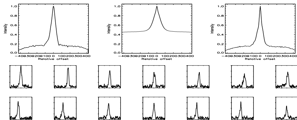
FIGURE B.634: SFP inspection for HD 220140 with S1-W1 on UT 2007/09/16, seq 001
