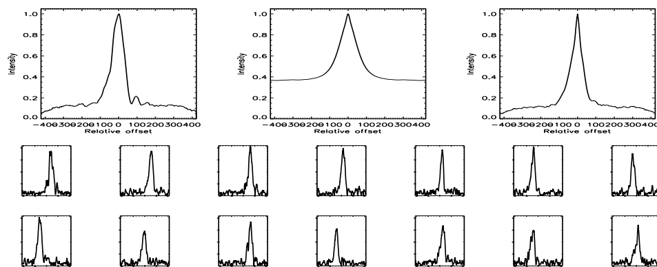
FIGURE B.154: SFP inspection for HD 038230 with S2-E2 on UT 2007/11/19, seq 002
