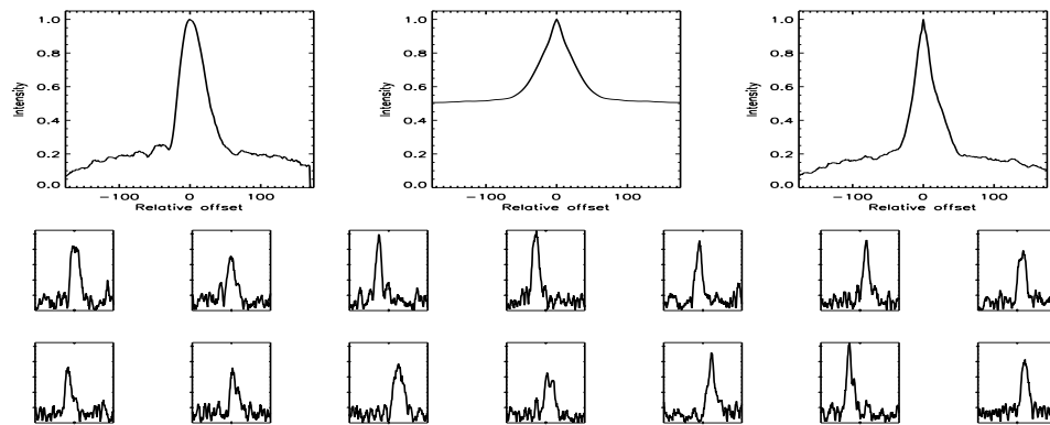
FIGURE B.75: SFP inspection for HD 017382 with S1-W1 on UT 2008/07/07, seq 001
