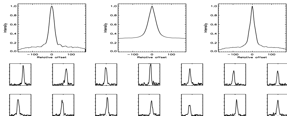
FIGURE B.502: SFP inspection for HD 176377 with S1-W1 on UT 2008/04/13, seq 001
