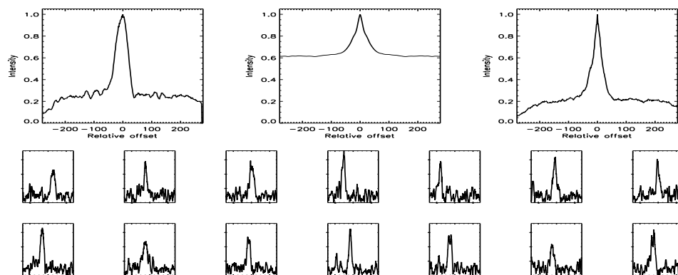
FIGURE B.460: SFP inspection for HD 159062 with S1-W1 on UT 2007/08/21, seq 002
