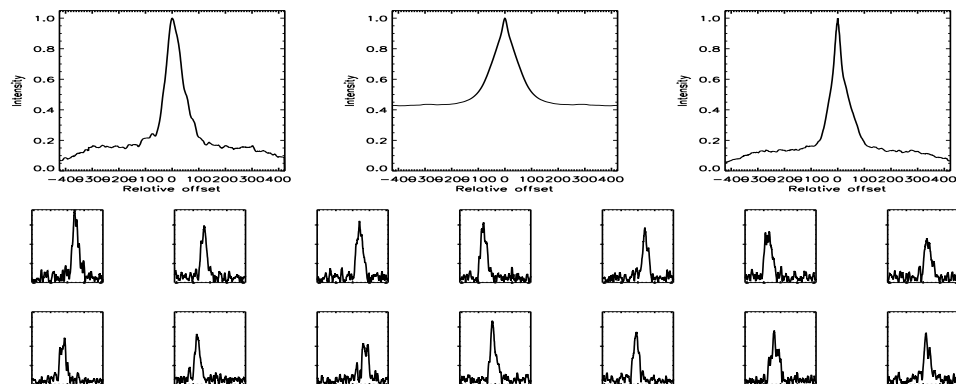
FIGURE B.614: SFP inspection for HD 216520 with S1-E1 on UT 2007/09/16, seq 002
