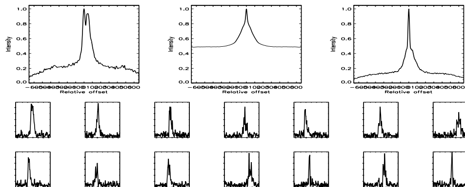
FIGURE B.590: SFP inspection for HD 202751 with S2-W1 on UT 2007/09/17, seq 001
