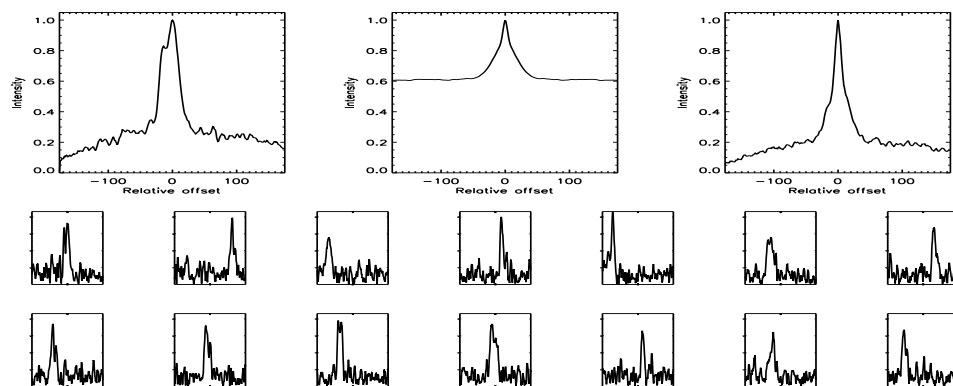
FIGURE B.37: SFP inspection for HD 007590 with S1-E1 on UT 2008/07/09, seq 001
