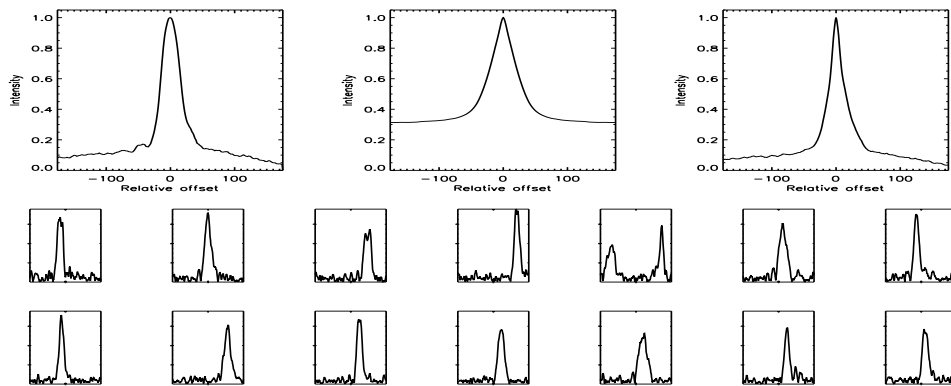
FIGURE B.363: SFP inspection for HD 135204 with S1-E1 on UT 2008/06/23, seq 001
