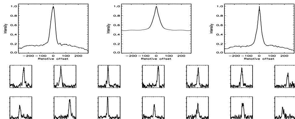
FIGURE B.316: SFP inspection for HD 124292 with S1-E1 on UT 2007/03/12, seq 002
