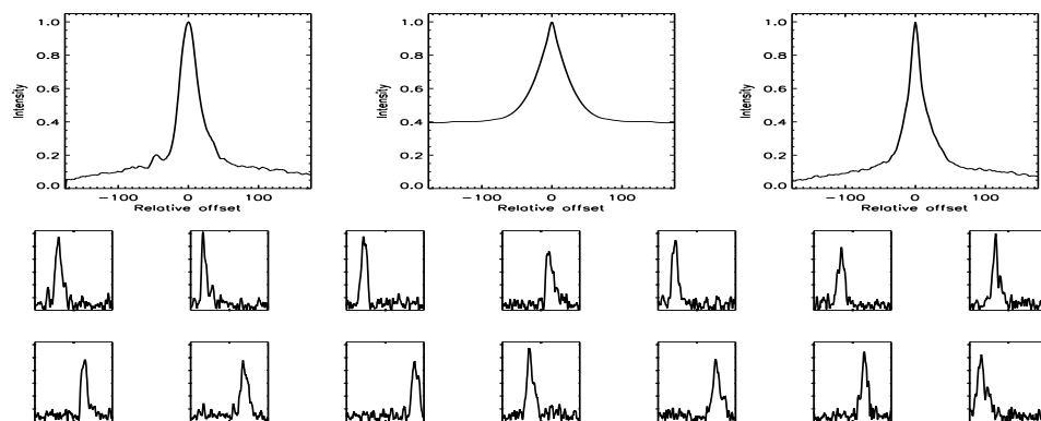
FIGURE B.499: SFP inspection for HD 176377 with S1-E1 on UT 2008/06/21, seq 001
