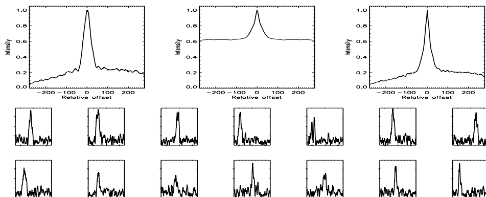
FIGURE B.402: SFP inspection for HD 139341 with S1-W1 on UT 2007/04/17, seq 004
