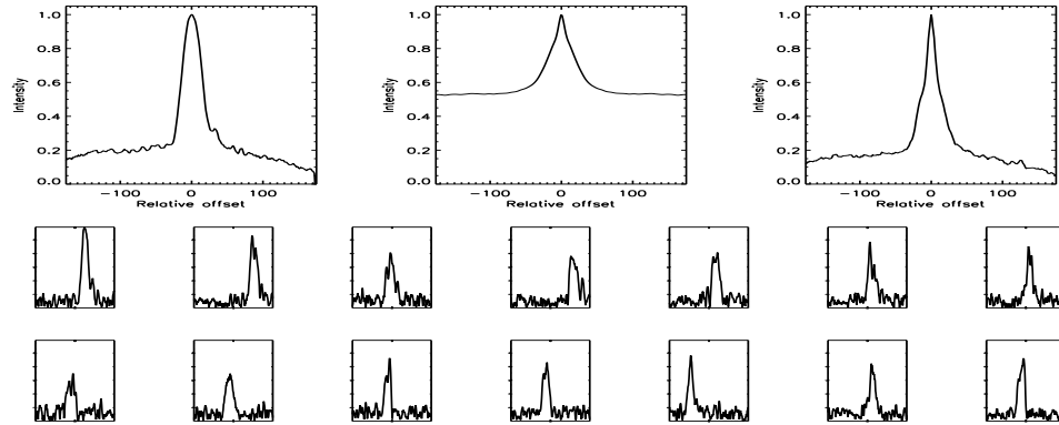
FIGURE B.356: SFP inspection for HD 132142 with S1-E1 on UT 2008/06/25, seq 001
