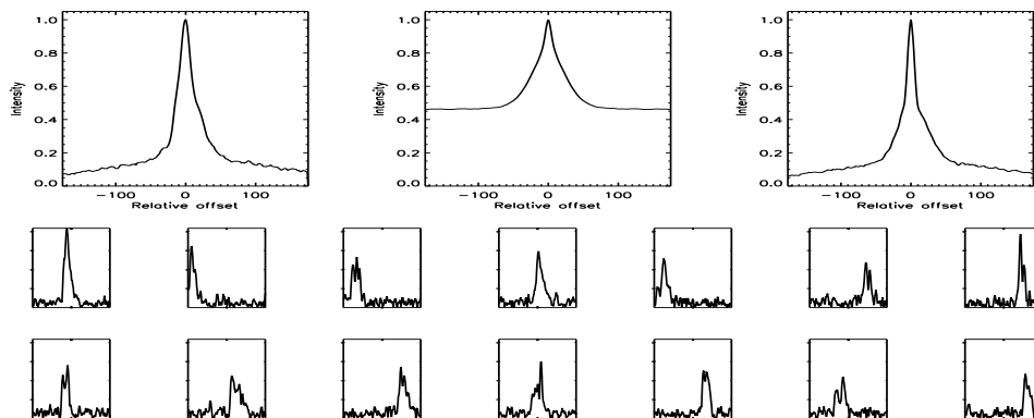
FIGURE B.533: SFP inspection for HD 189340 with S1-E1 on UT 2008/06/21, seq 001
