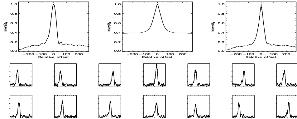
FIGURE B.194: SFP inspection for HD 067228 with S1-E1 on UT 2007/02/06, seq 002
