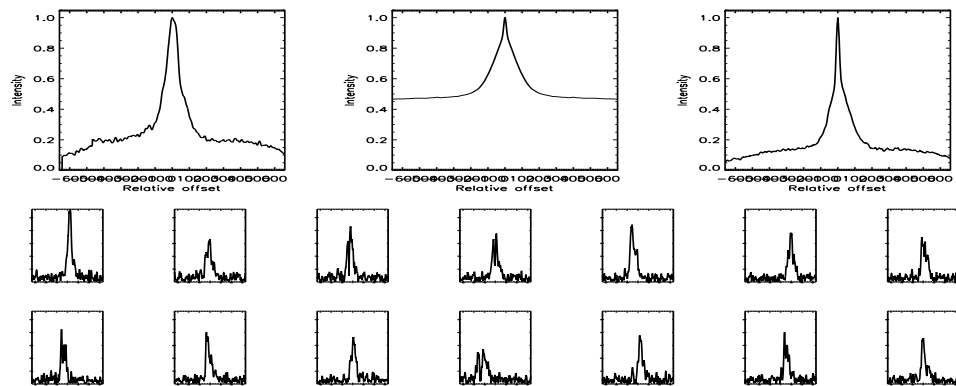
FIGURE B.78: SFP inspection for HD 017382 with S2-W1 on UT 2007/09/17, seq 001
