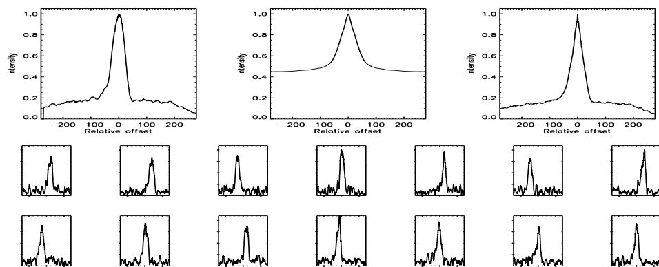
FIGURE B.562: SFP inspection for HD 191785 with S1-E1 on UT 2007/07/24, seq 001
