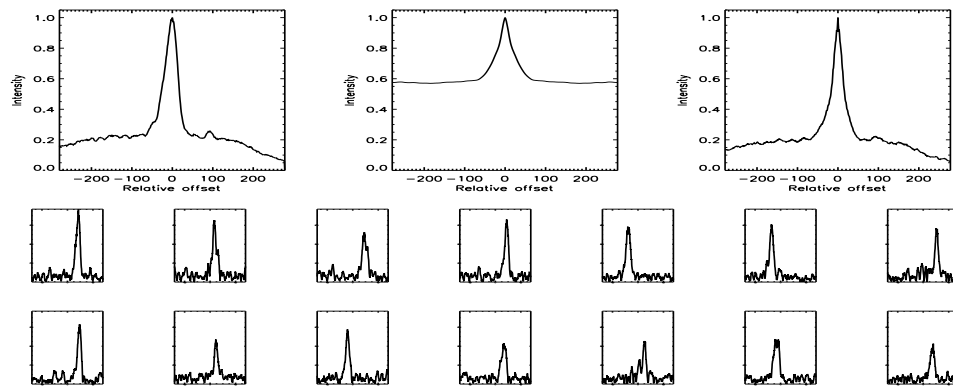
FIGURE B.309: SFP inspection for HD 119332 with S1-E1 on UT 2007/04/03, seq 002
