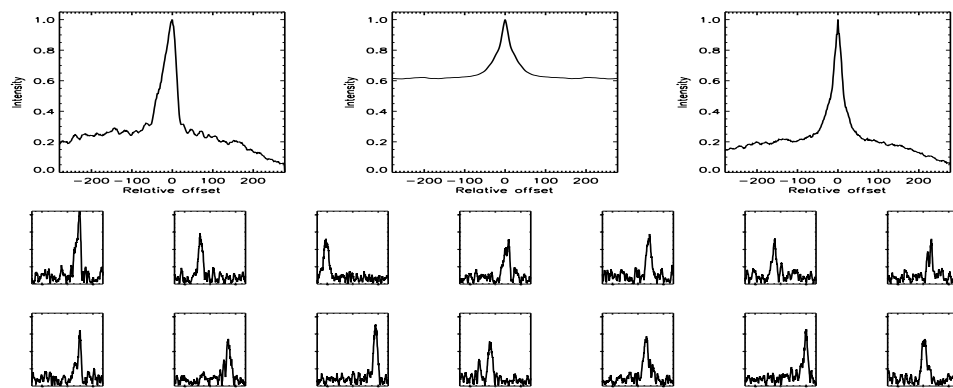
FIGURE B.300: SFP inspection for HD 116442 with S1-W1 on UT 2007/06/01, seq 001
