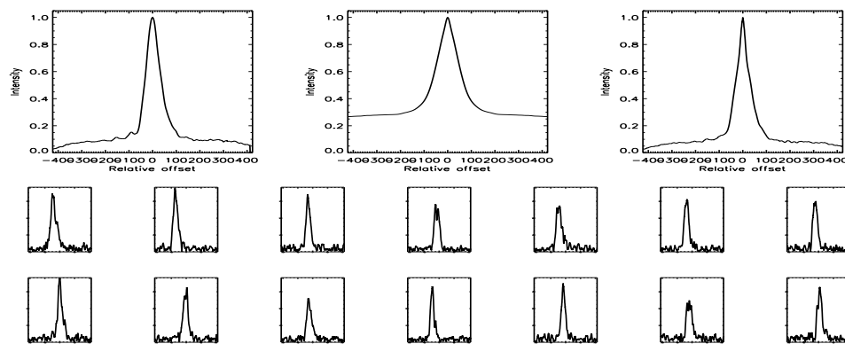
FIGURE B.603: SFP inspection for HD 210277 with S2-W1 on UT 2007/09/17, seq 001
