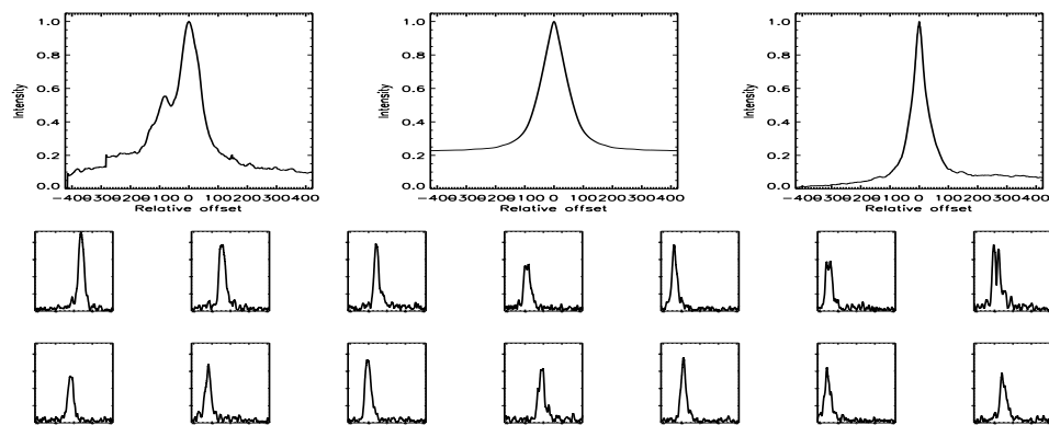
FIGURE B.54: SFP inspection for HD 010780 with S1-W1 on UT 2007/09/16, seq 001
