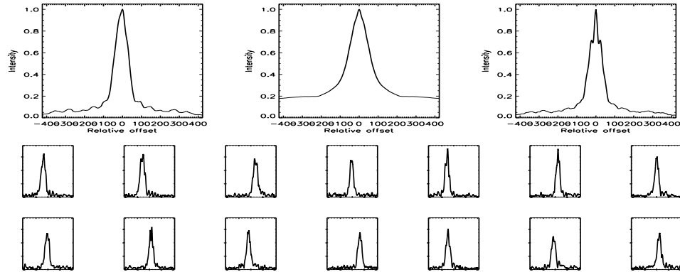
FIGURE B.68: SFP inspection for HD 016673 with S1-E1 on UT 2007/08/15, seq 001
