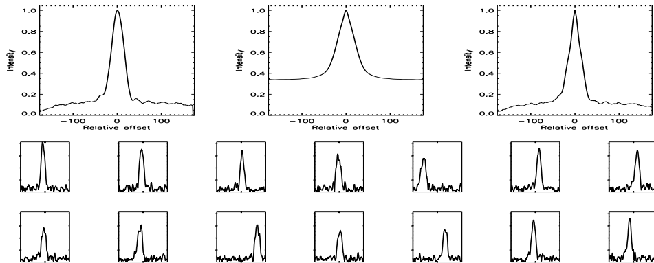
FIGURE B.434: SFP inspection for HD 151541 with S2-W1 on UT 2008/06/24, seq 001
