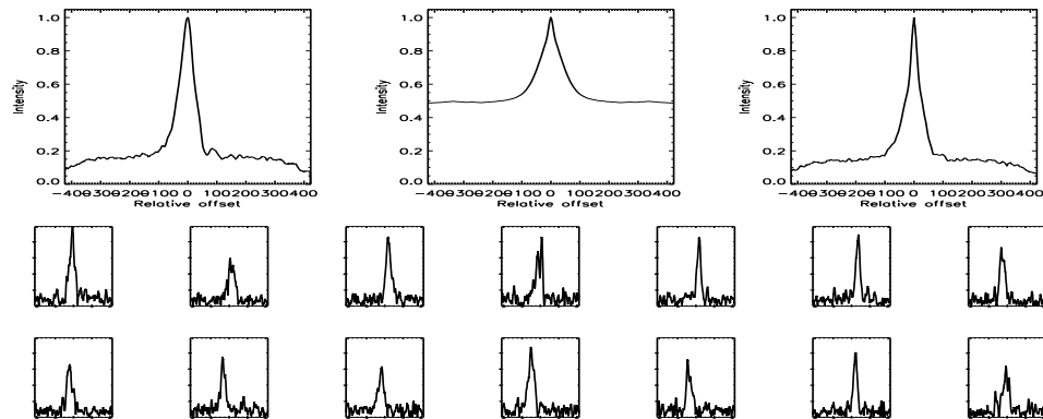
FIGURE B.142: SFP inspection for HD 037008 with S2-E2 on UT 2007/11/19, seq 002
