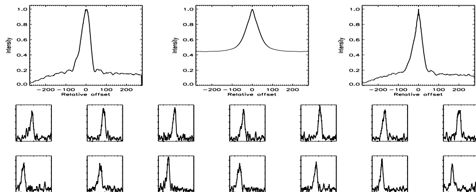
FIGURE B.578: SFP inspection for HD 197076 with S1-W1 on UT 2007/07/22, seq 001
