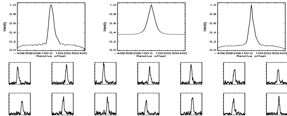
FIGURE B.121: SFP inspection for HD 026913 with S1-W1 on UT 2007/10/31, seq 002
