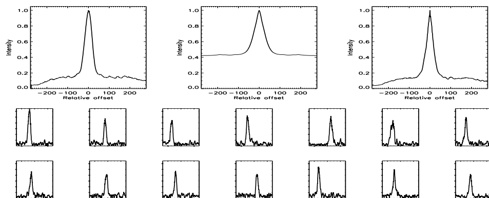
FIGURE B.301: SFP inspection for HD 116443 with S1-E1 on UT 2007/03/12, seq 001
