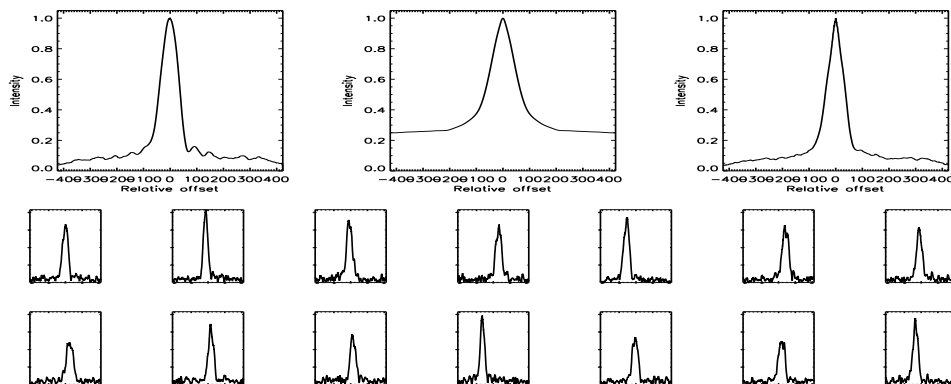
FIGURE B.554: SFP inspection for HD 190771 with S1-W1 on UT 2007/08/18, seq 001
