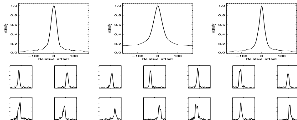
FIGURE B.275: SFP inspection for HD 104304 with S1-W1 on UT 2008/04/15, seq 001
