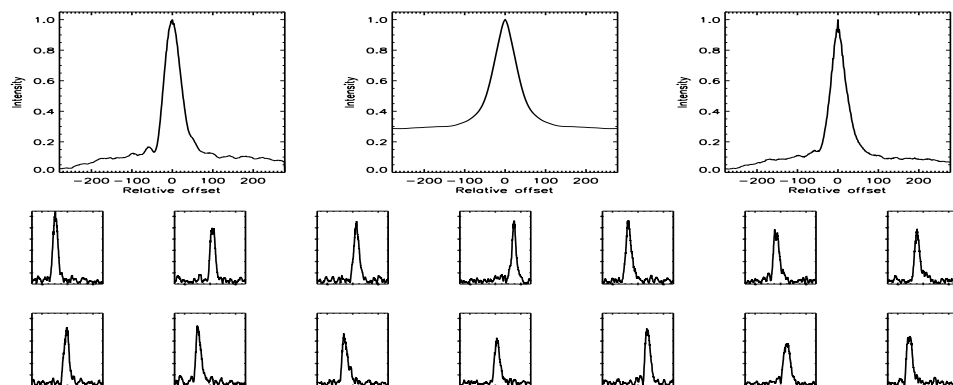
FIGURE B.441: SFP inspection for HD 154345 with S1-E1 on UT 2007/04/14, seq 001
