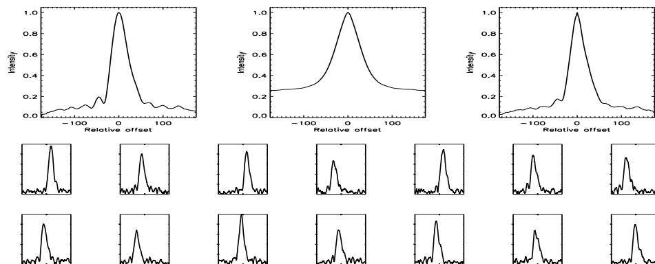
FIGURE B.395: SFP inspection for HD 137778 with S1-W1 on UT 2008/07/07, seq 002
