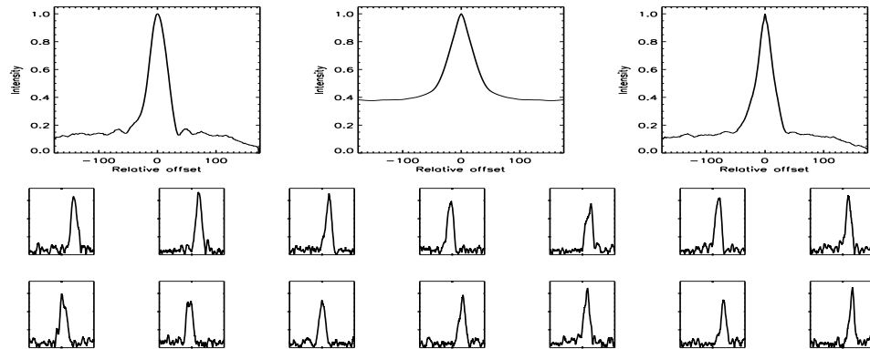
FIGURE B.263: SFP inspection for HD 099491 with S1-E1 on UT 2008/04/14, seq 001
