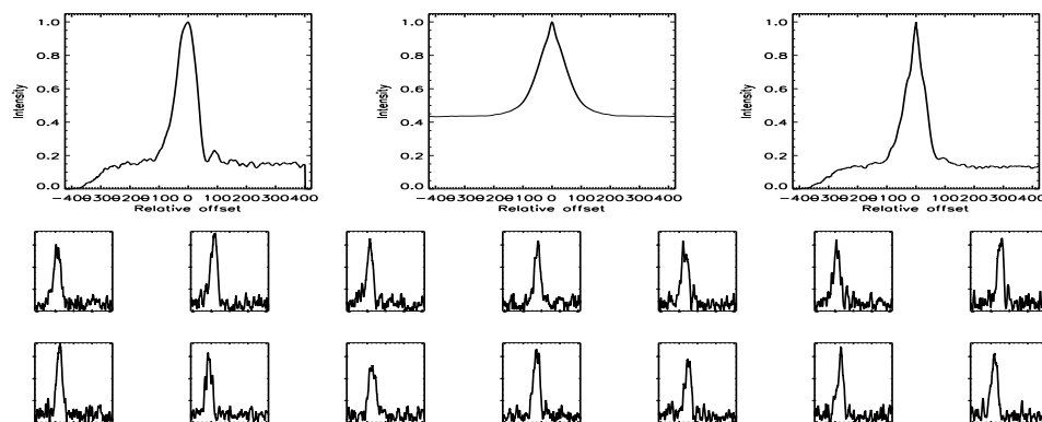
FIGURE B.559: SFP inspection for HD 191499 with S1-W1 on UT 2007/07/22, seq 001
