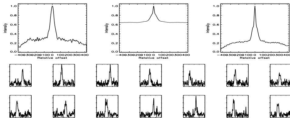
FIGURE B.126: SFP inspection for HD 029883 with S2-E2 on UT 2007/09/18, seq 001
