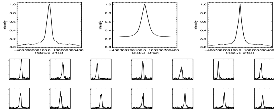
FIGURE B.53: SFP inspection for HD 010780 with S1-E1 on UT 2007/09/16, seq 002
