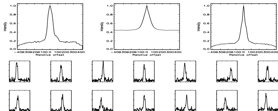
FIGURE B.165: SFP inspection for HD 042618 with S1-W1 on UT 2007/11/01, seq 001
