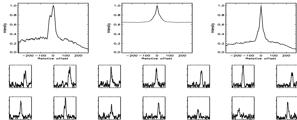
FIGURE B.255: SFP inspection for HD 098230 with S1-W1 on UT 2007/06/01, seq 001
