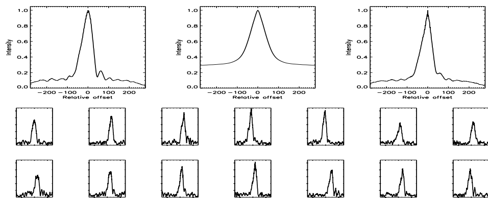
FIGURE B.115: SFP inspection for HD 025457 with S2-E2 on UT 2007/09/26, seq 001
