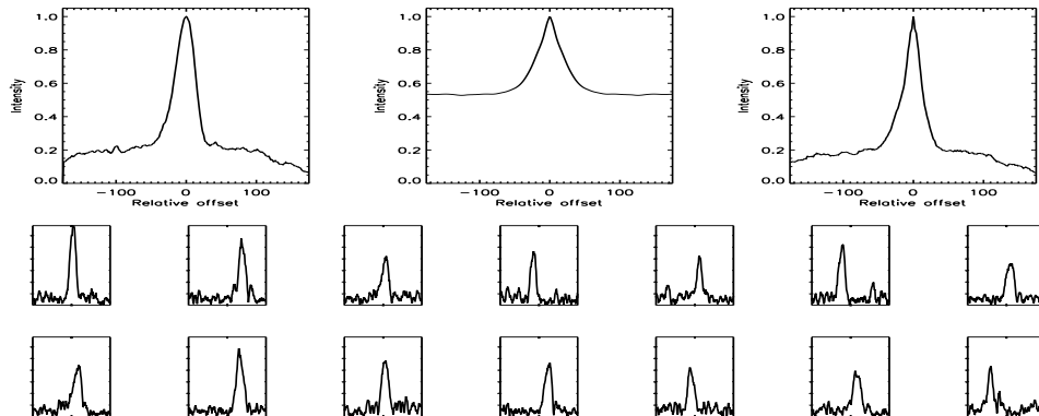
FIGURE B.23: SFP inspection for HD 003765 with S1-W1 on UT 2008/07/08, seq 001
