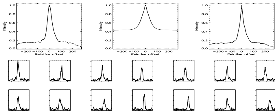
FIGURE B.505: SFP inspection for HD 178428 with S1-E2 on UT 2007/05/29, seq 001
