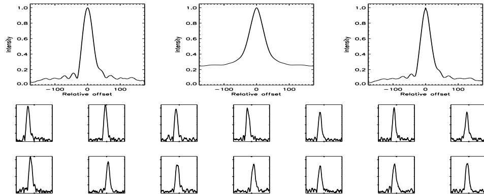
FIGURE B.392: SFP inspection for HD 137778 with S1-W1 on UT 2008/04/14, seq 001
