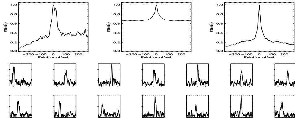
FIGURE B.278: SFP inspection for HD 105631 with S1-W1 on UT 2007/06/01, seq 001
