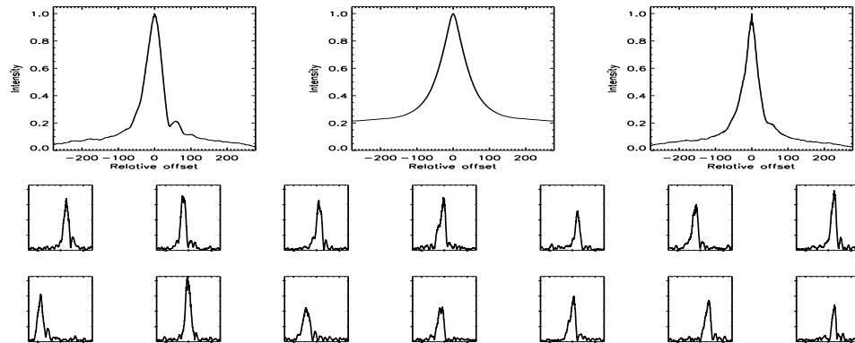
FIGURE B.257: SFP inspection for HD 098230 with S1-W1 on UT 2007/06/01, seq 003
