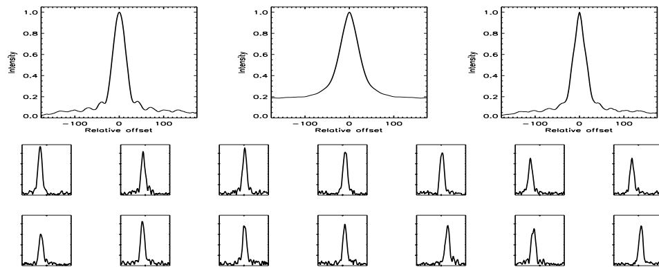
FIGURE B.342: SFP inspection for HD 128311 with S1-W1 on UT 2008/04/13, seq 002
