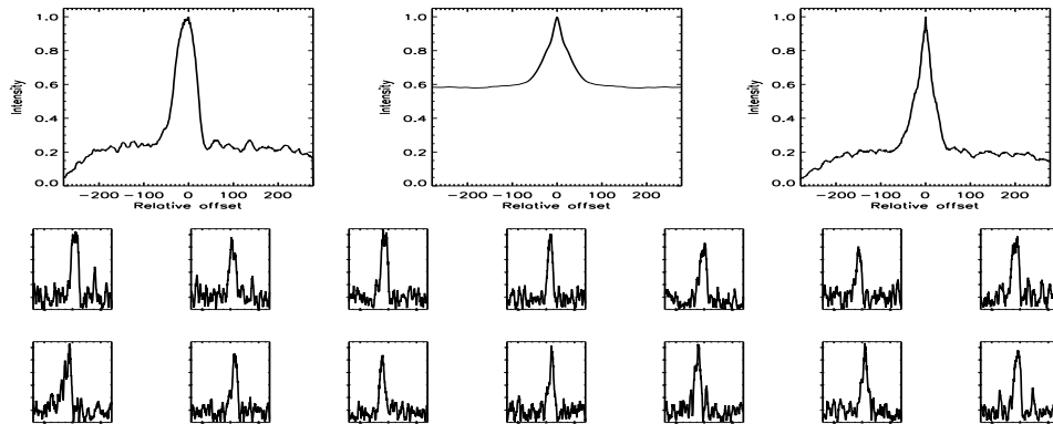
FIGURE B.437: SFP inspection for HD 153557 with S1-W1 on UT 2007/08/21, seq 001
