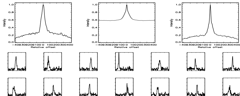
FIGURE B.143: SFP inspection for HD 037008 with S2-E2 on UT 2007/11/27, seq 001
