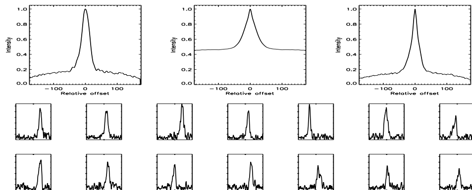
FIGURE B.218: SFP inspection for HD 079969 with S1-W1 on UT 2008/04/12, seq 001
