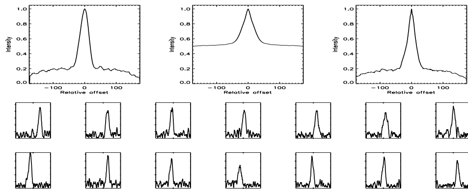
FIGURE B.76: SFP inspection for HD 017382 with S1-W1 on UT 2008/07/08, seq 001
