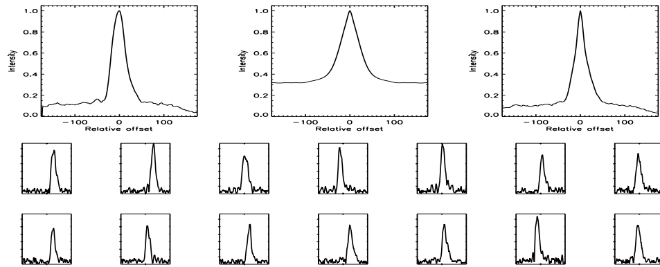
FIGURE B.237: SFP inspection for HD 090343 with S2-W1 on UT 2008/06/24, seq 001
