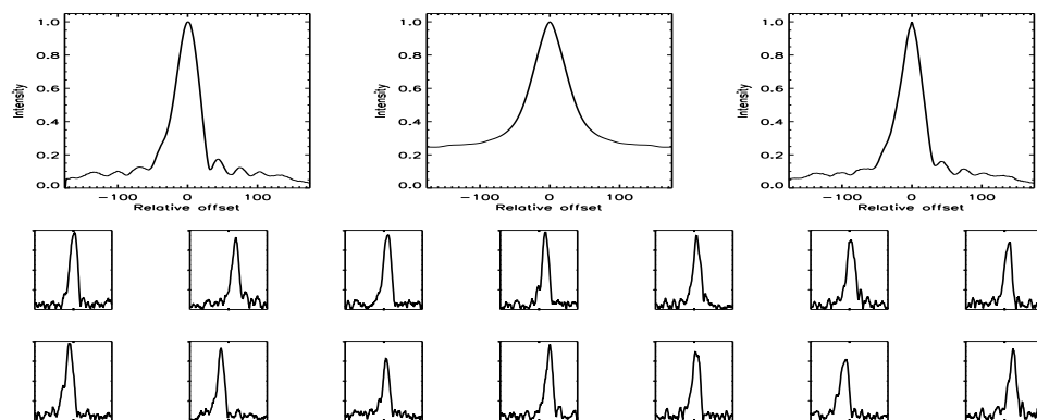
FIGURE B.331: SFP inspection for HD 125455 with S1-W1 on UT 2008/04/14, seq 002
