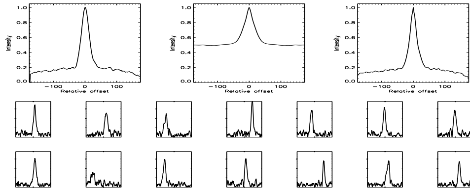
FIGURE B.242: SFP inspection for HD 097334 with S1-E1 on UT 2008/04/12, seq 002
