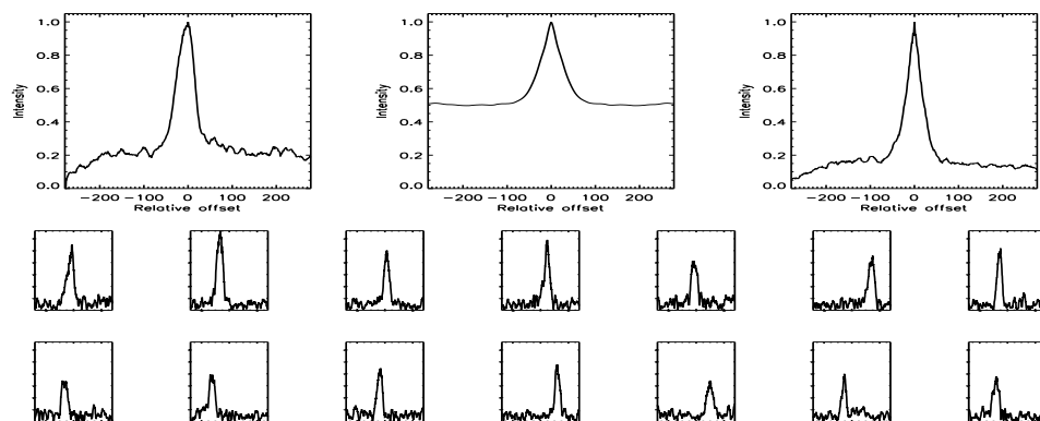
FIGURE B.625: SFP inspection for HD 218868 with S1-W1 on UT 2007/07/26, seq 002
