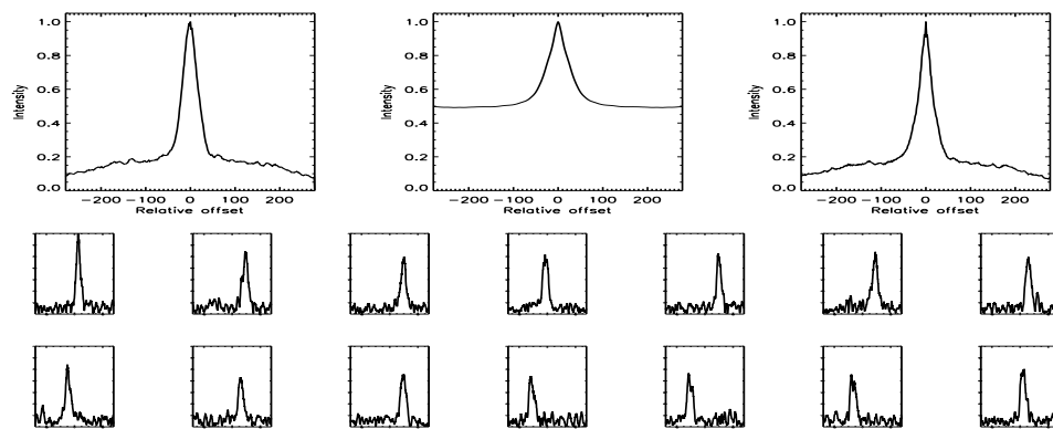
FIGURE B.540: SFP inspection for HD 189733 with S1-W1 on UT 2007/05/30, seq 001
