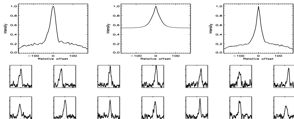
FIGURE B.190: SFP inspection for HD 063433 with S1-W1 on UT 2008/04/12, seq 001
