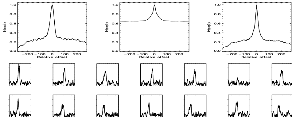
FIGURE B.509: SFP inspection for HD 179957 with S1-W1 on UT 2007/05/30, seq 001
