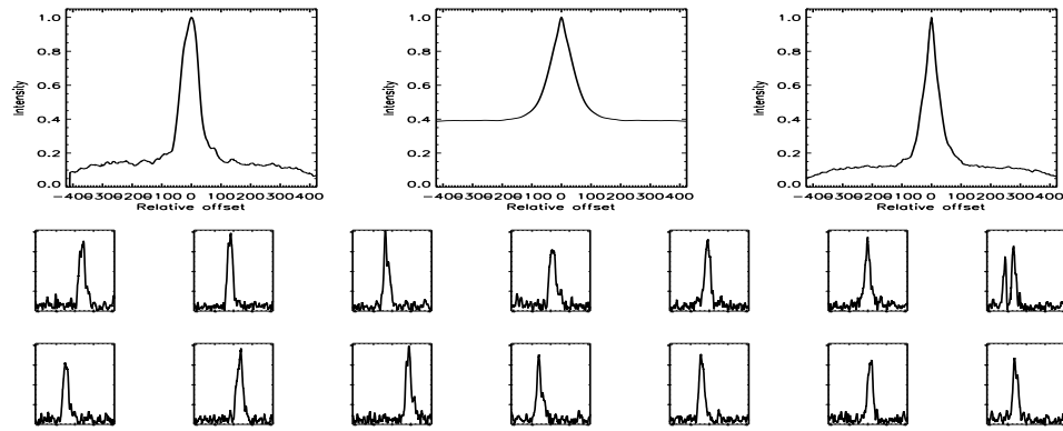
FIGURE B.87: SFP inspection for HD 018757 with S2-E1 on UT 2007/08/20, seq 001
