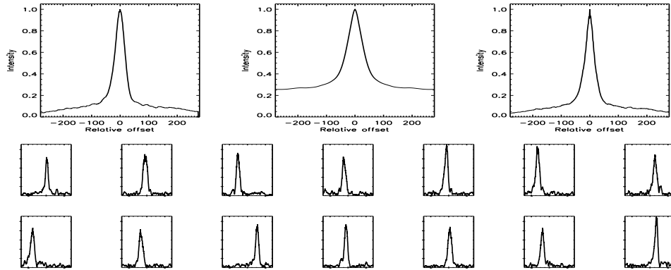
FIGURE B.359: SFP inspection for HD 132254 with E1-W1 on UT 2007/04/26, seq 001
