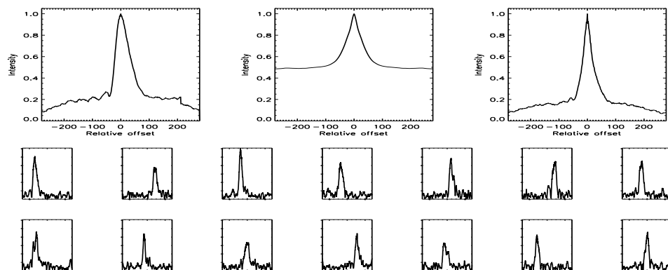
FIGURE B.498: SFP inspection for HD 176377 with S1-E1 on UT 2007/04/14, seq 001
