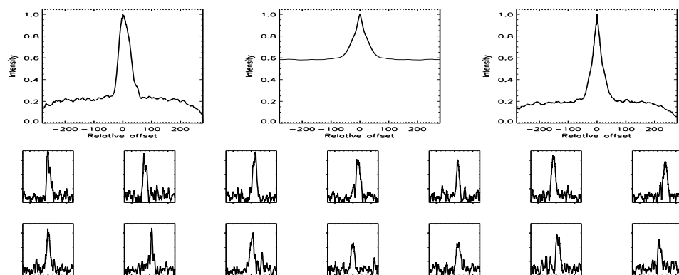
FIGURE B.592: SFP inspection for HD 208038 with S1-E1 on UT 2007/08/14, seq 001
