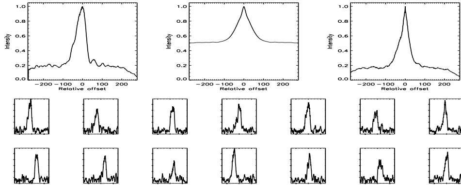
FIGURE B.122: SFP inspection for HD 026913 with S2-E2 on UT 2007/09/26, seq 001
