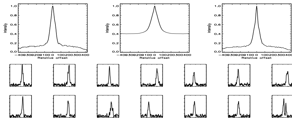
FIGURE B.153: SFP inspection for HD 038230 with S1-W1 on UT 2007/11/01, seq 001
