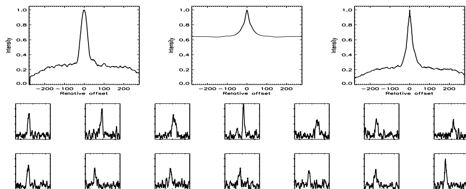
FIGURE B.400: SFP inspection for HD 139341 with S1-W1 on UT 2007/04/17, seq 001
