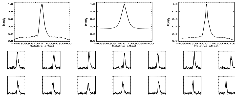
FIGURE B.124: SFP inspection for HD 026923 with S1-W1 on UT 2007/10/31, seq 002
