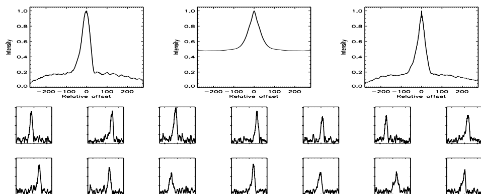
FIGURE B.339: SFP inspection for HD 128165 with S1-W1 on UT 2007/05/28, seq 001
