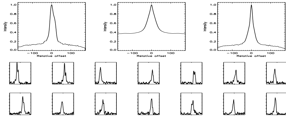
FIGURE B.477: SFP inspection for HD 165401 with S1-E1 on UT 2008/04/25, seq 001
