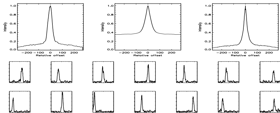
FIGURE B.285: SFP inspection for HD 110833 with S1-W1 on UT 2007/04/17, seq 001
