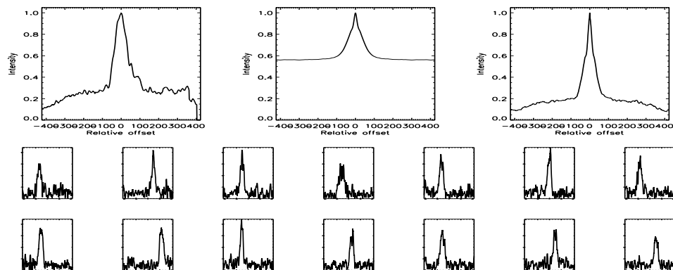
FIGURE B.605: SFP inspection for HD 210667 with S1-E1 on UT 2007/07/28, seq 001
