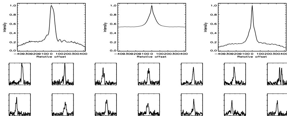
FIGURE B.556: SFP inspection for HD 190771 with S2-E1 on UT 2007/08/20, seq 001
