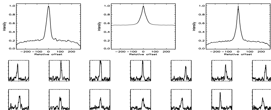
FIGURE B.328: SFP inspection for HD 125455 with S1-E1 on UT 2007/03/12, seq 001
