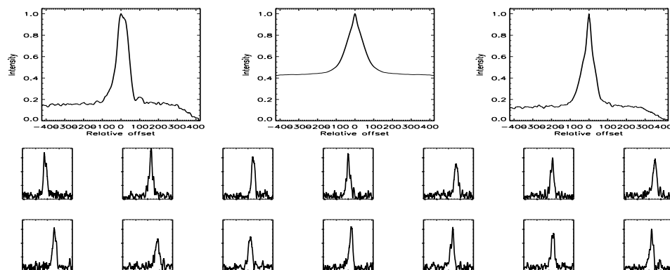
FIGURE B.159: SFP inspection for HD 040397 with S1-W1 on UT 2007/11/01, seq 001
