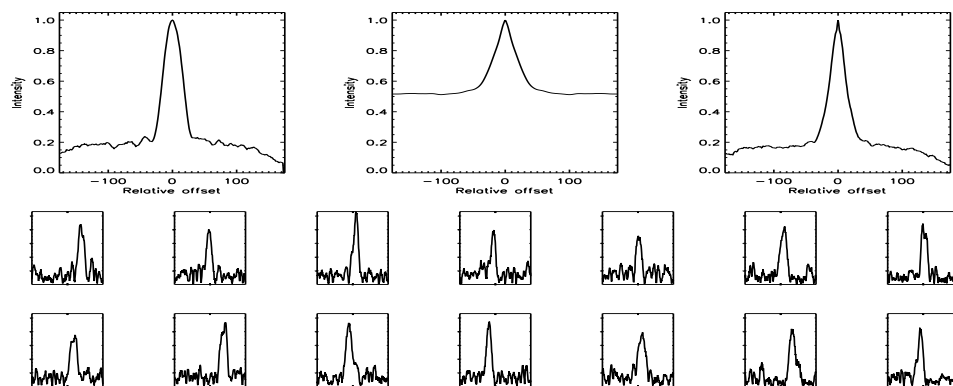
FIGURE B.244: SFP inspection for HD 097658 with S1-E1 on UT 2008/04/13, seq 001
