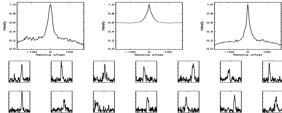
FIGURE B.8: SFP inspection for HD 001562 with S1-E1 on UT 2008/07/09, seq 001
