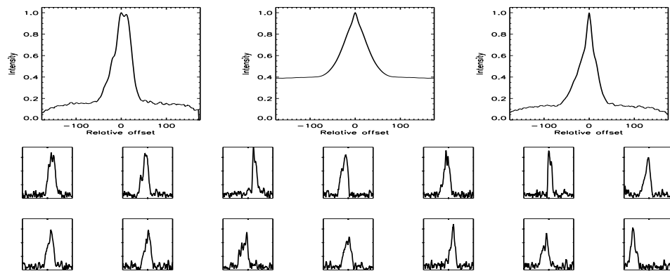
FIGURE B.538: SFP inspection for HD 189340 with S2-W2 on UT 2008/06/09, seq 002
