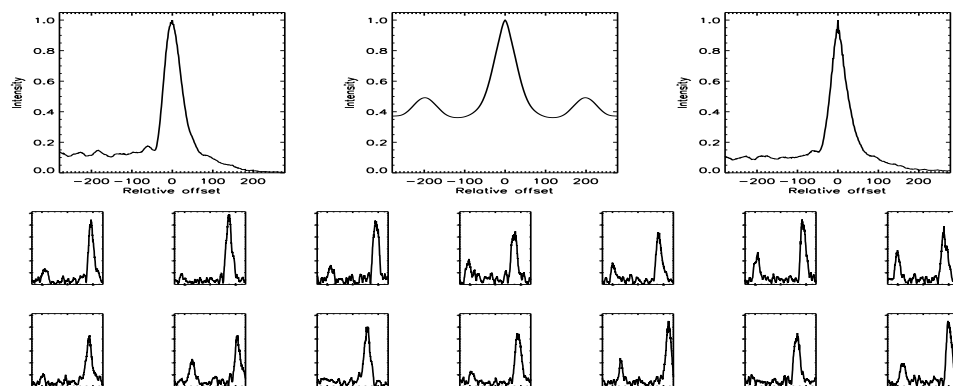
FIGURE B.13: SFP inspection for HD 003196 with S1-W1 on UT 2007/08/14, seq 004
