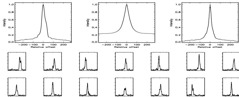
FIGURE B.195: SFP inspection for HD 067228 with S1-E1 on UT 2007/02/25, seq 001
