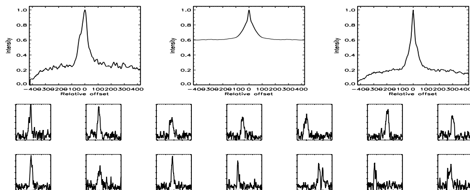
FIGURE B.412: SFP inspection for HD 142267 with S1-E1 on UT 2007/08/15, seq 001
