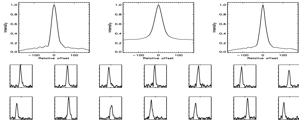
FIGURE B.260: SFP inspection for HD 098281 with S1-W1 on UT 2008/04/15, seq 001
