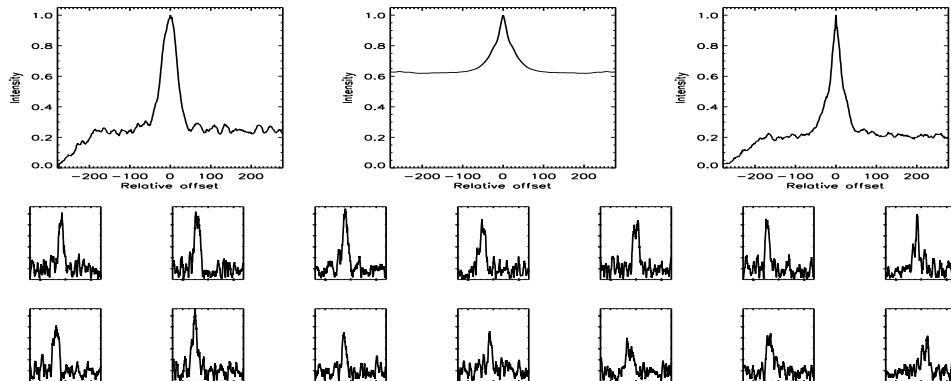
FIGURE B.593: SFP inspection for HD 208038 with S1-W1 on UT 2007/08/14, seq 002
