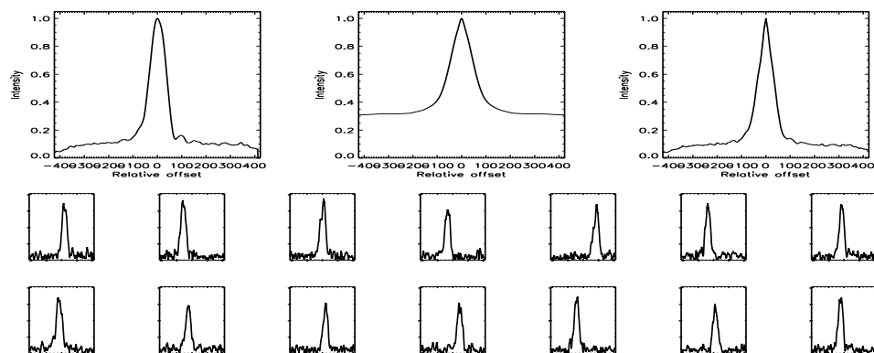
FIGURE B.646: SFP inspection for HD 222143 with S1-W1 on UT 2007/08/18, seq 001
