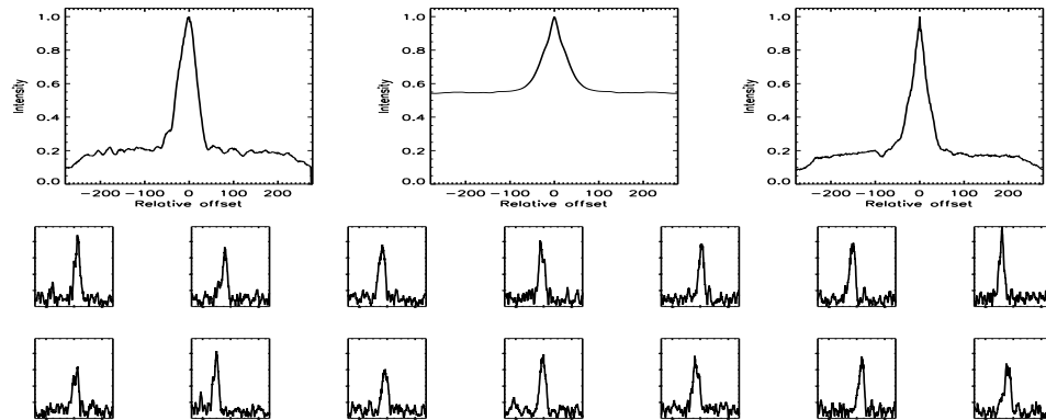
FIGURE B.539: SFP inspection for HD 189733 with S1-E1 on UT 2007/07/24, seq 001
