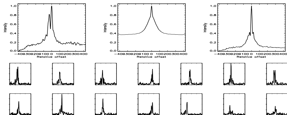
FIGURE B.489: SFP inspection for HD 166620 with S2-W1 on UT 2007/09/17, seq 001
