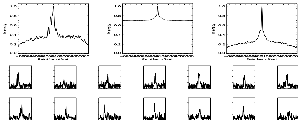
FIGURE B.495: SFP inspection for HD 175742 with S2-E2 on UT 2007/09/18, seq 003
