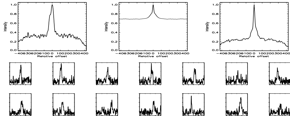
FIGURE B.587: SFP inspection for HD 200560 with S2-E1 on UT 2007/08/20, seq 001
