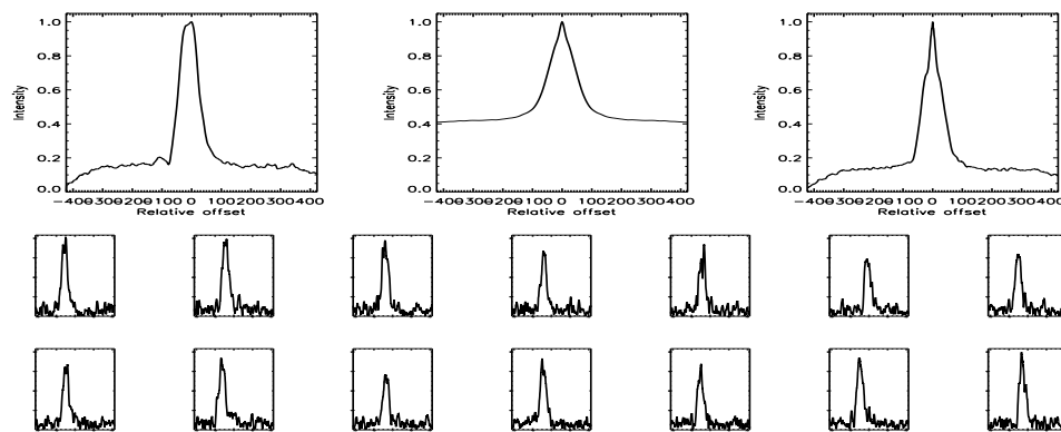
FIGURE B.36: SFP inspection for HD 007590 with S1-E1 on UT 2007/08/16, seq 002
