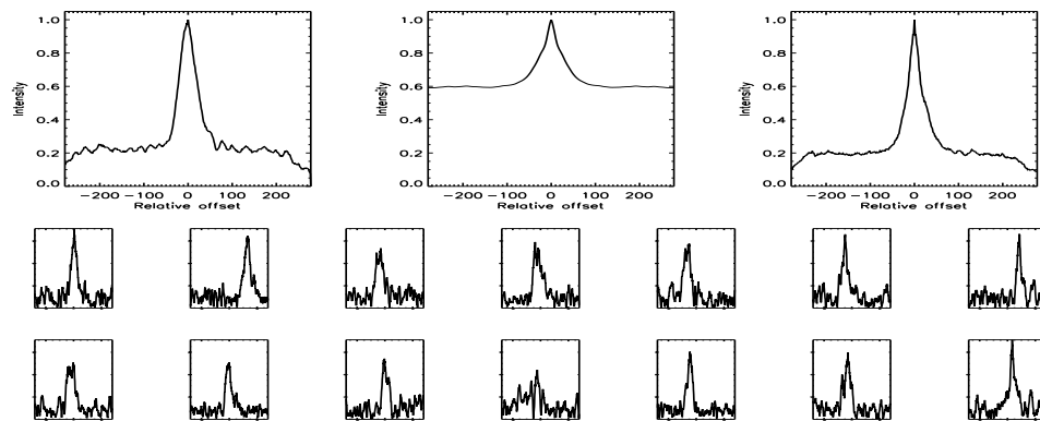
FIGURE B.628: SFP inspection for HD 219538 with S1-E1 on UT 2007/08/14, seq 001
