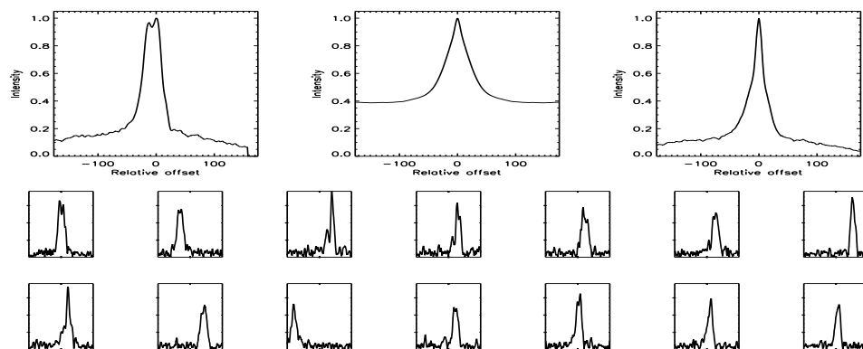
FIGURE B.307: SFP inspection for HD 116956 with S1-W1 on UT 2008/04/26, seq 001
