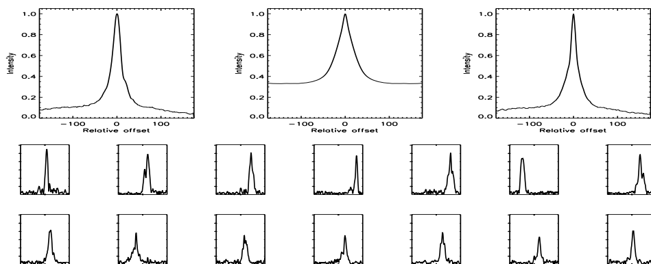
FIGURE B.325: SFP inspection for HD 124850 with S1-E2 on UT 2008/06/08, seq 002
