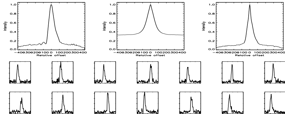
FIGURE B.653: SFP inspection for HD 224465 with S1-E1 on UT 2007/08/18, seq 002
