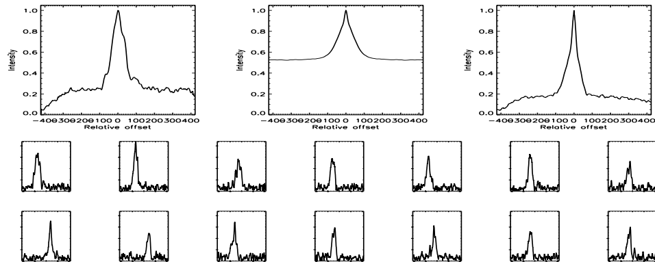
FIGURE B.560: SFP inspection for HD 191499 with S1-W1 on UT 2007/07/24, seq 002
