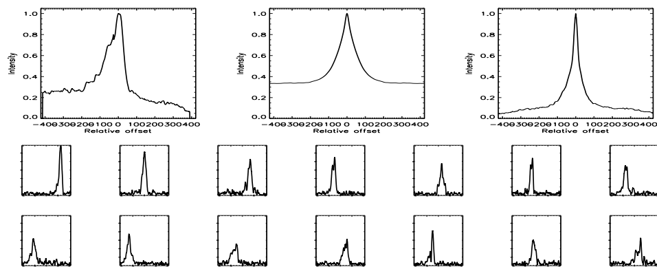
FIGURE B.522: SFP inspection for HD 182488 with S2-W1 on UT 2007/09/17, seq 001
