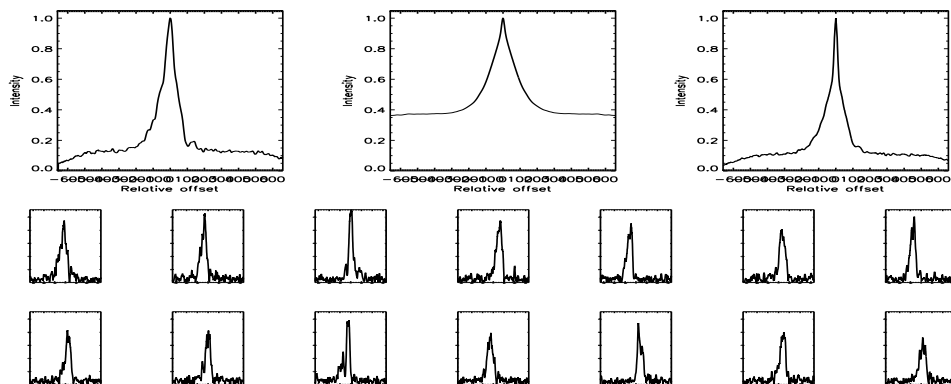
FIGURE B.503: SFP inspection for HD 176377 with S2-W1 on UT 2007/09/17, seq 001
