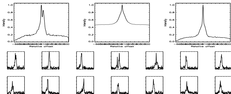
FIGURE B.496: SFP inspection for HD 175742 with S2-W1 on UT 2007/09/17, seq 001
