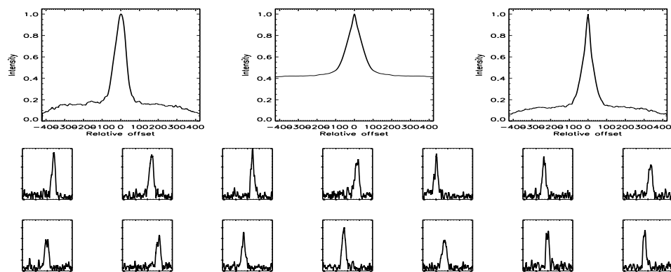
FIGURE B.553: SFP inspection for HD 190771 with S1-E1 on UT 2007/08/18, seq 002
