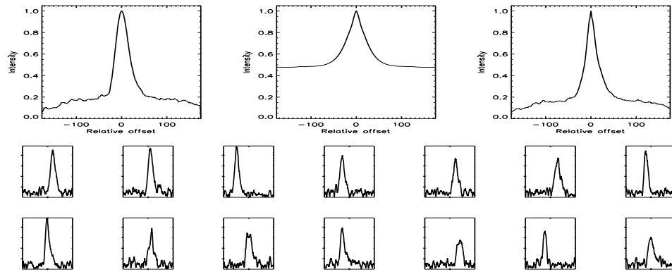
FIGURE B.357: SFP inspection for HD 132142 with S1-W1 on UT 2008/04/12, seq 001
