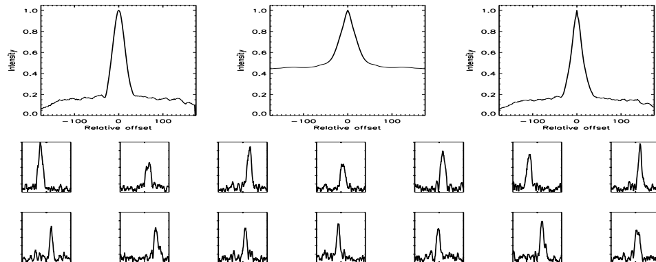
FIGURE B.371: SFP inspection for HD 135204 with S2-W2 on UT 2008/06/09, seq 001
