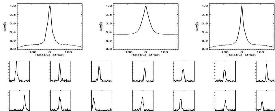
FIGURE B.451: SFP inspection for HD 158614 with S1-E1 on UT 2008/04/25, seq 001
