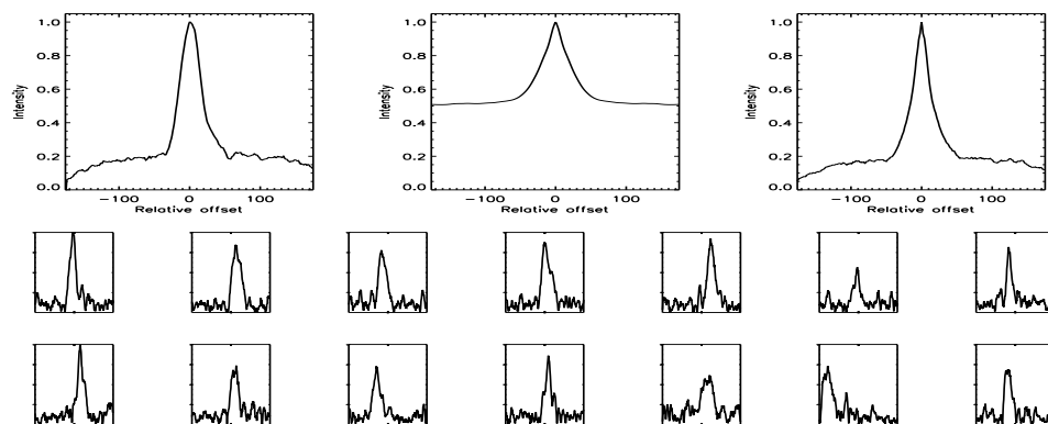
FIGURE B.610: SFP inspection for HD 215152 with S1-E1 on UT 2008/07/06, seq 001
