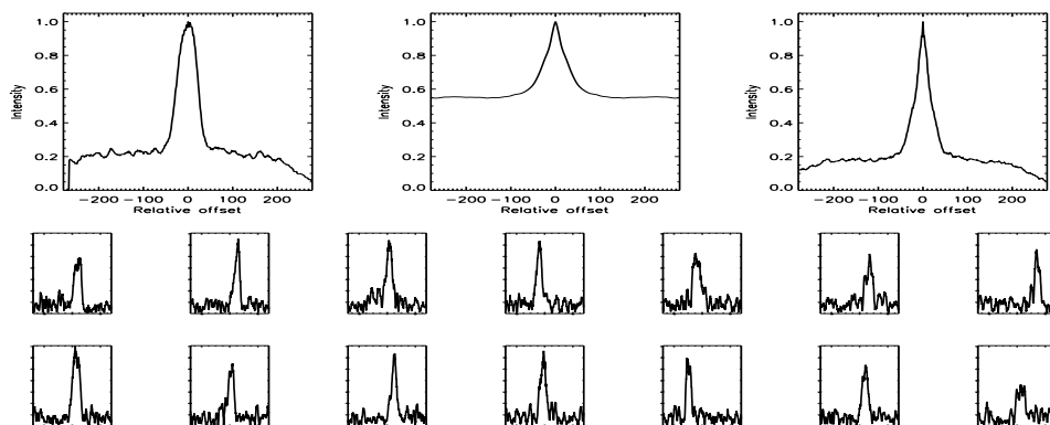
FIGURE B.24: SFP inspection for HD 004256 with S1-E1 on UT 2007/08/14, seq 001
