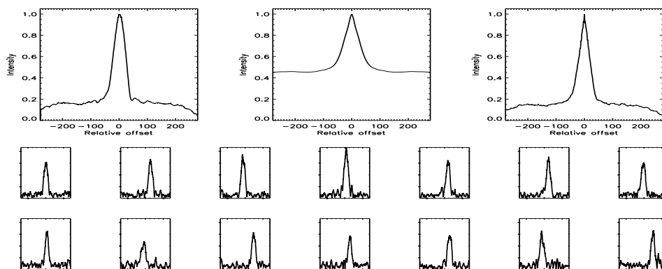
FIGURE B.577: SFP inspection for HD 197076 with S1-E1 on UT 2007/07/24, seq 001
