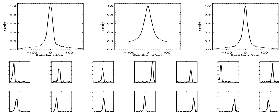
FIGURE B.258: SFP inspection for HD 098230 with S1-W1 on UT 2008/04/12, seq 001
