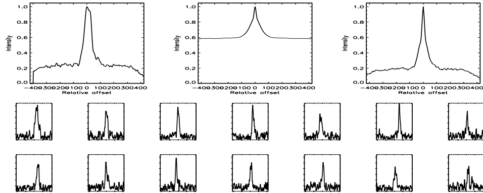
FIGURE B.176: SFP inspection for HD 051866 with S2-E2 on UT 2007/11/19, seq 002
