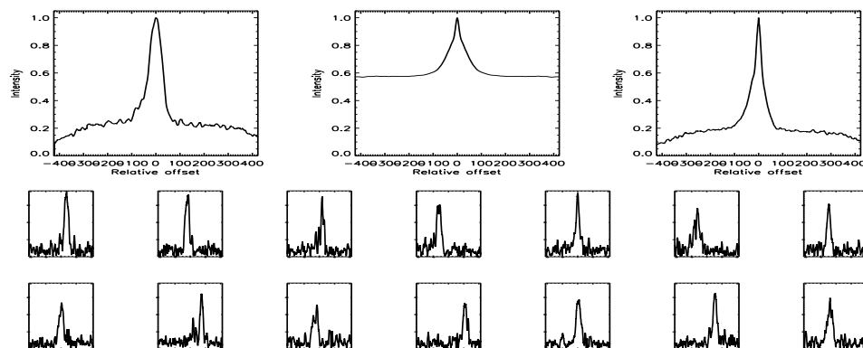
FIGURE B.219: SFP inspection for HD 079969 with S2-E2 on UT 2007/11/29, seq 001
