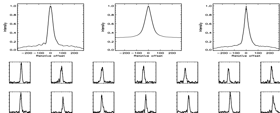
FIGURE B.442: SFP inspection for HD 154345 with S1-W1 on UT 2007/04/17, seq 001
