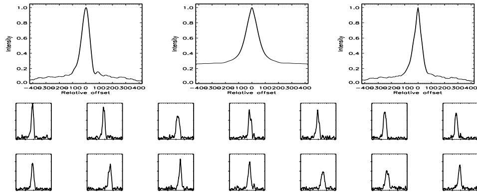
FIGURE B.50: SFP inspection for HD 010476 with S1-E1 on UT 2007/07/29, seq 001
