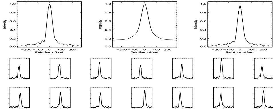
FIGURE B.626: SFP inspection for HD 219134 with S1-E1 on UT 2007/07/26, seq 002
