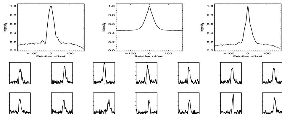
FIGURE B.349: SFP inspection for HD 130004 with S1-E1 on UT 2008/04/13, seq 001
