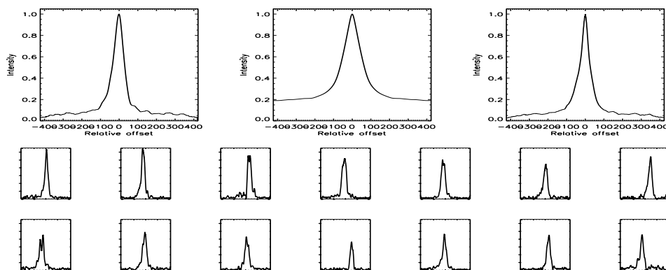
FIGURE B.529: SFP inspection for HD 185144 with S1-W1 on UT 2007/09/16, seq 001
