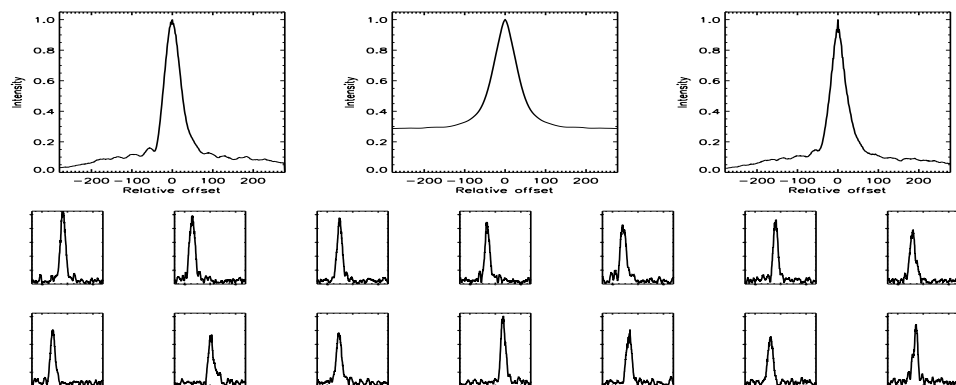
FIGURE B.519: SFP inspection for HD 182488 with S1-E1 on UT 2007/04/14, seq 001
