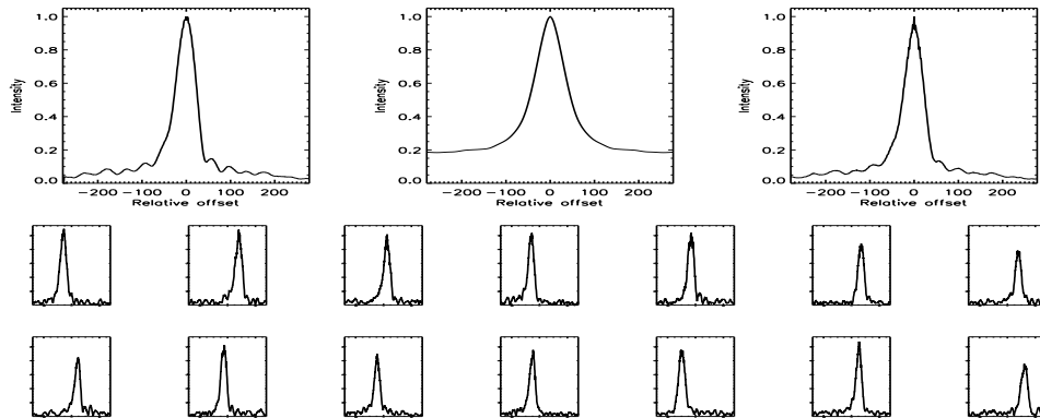
FIGURE B.254: SFP inspection for HD 098230 with S1-W1 on UT 2007/05/28, seq 001
