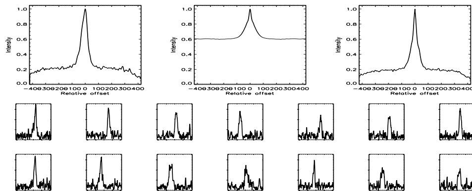
FIGURE B.58: SFP inspection for HD 012051 with S2-E2 on UT 2007/09/18, seq 001
