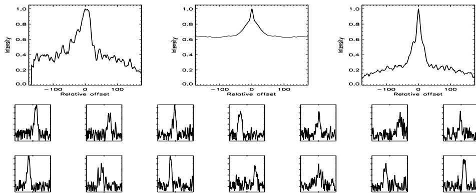
FIGURE B.435: SFP inspection for HD 153557 with S1-E1 on UT 2008/06/25, seq 001
