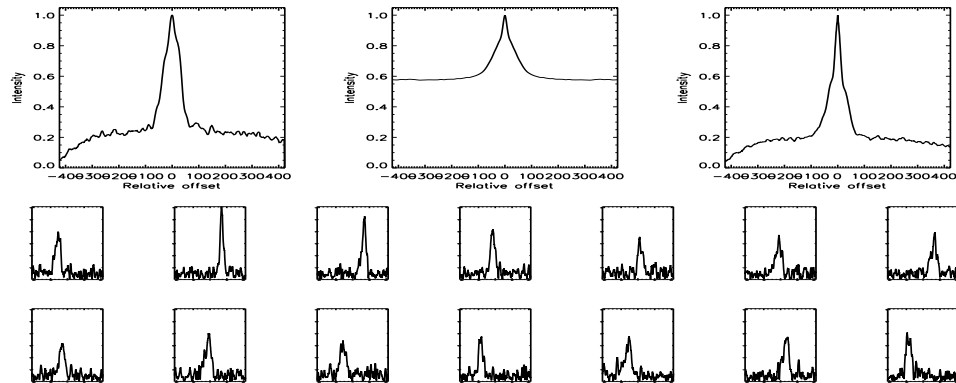
FIGURE B.632: SFP inspection for HD 219623 with S2-E1 on UT 2007/08/20, seq 001
