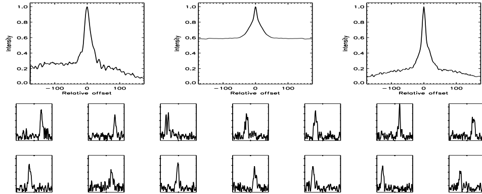
FIGURE B.566: SFP inspection for HD 192263 with S1-E1 on UT 2008/06/23, seq 001
