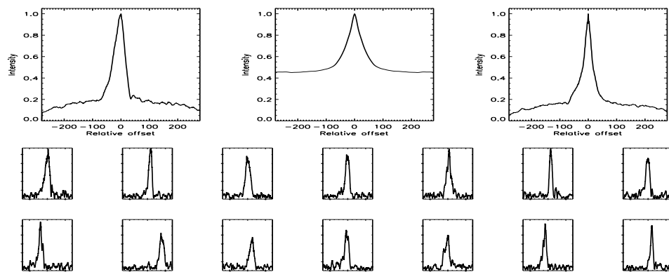
FIGURE B.282: SFP inspection for HD 108954 with S1-W1 on UT 2007/04/24, seq 001
