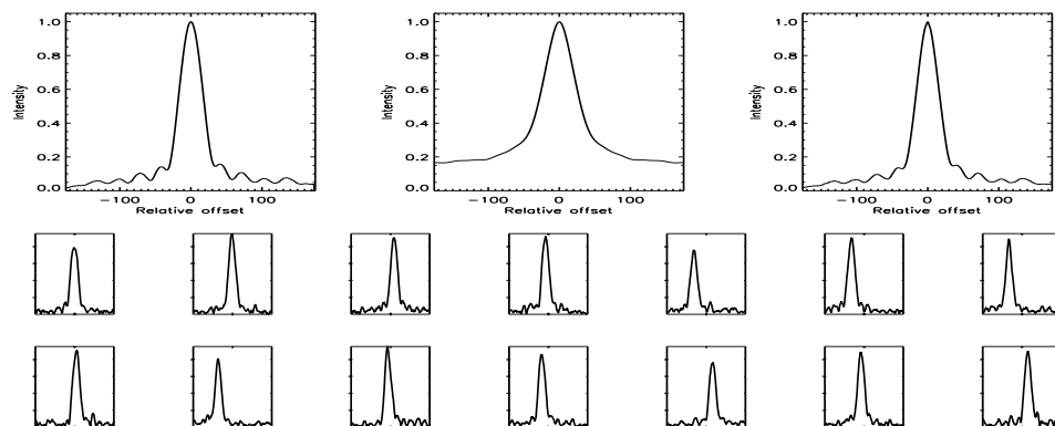
FIGURE B.453: SFP inspection for HD 158614 with S1-W1 on UT 2008/04/14, seq 001
