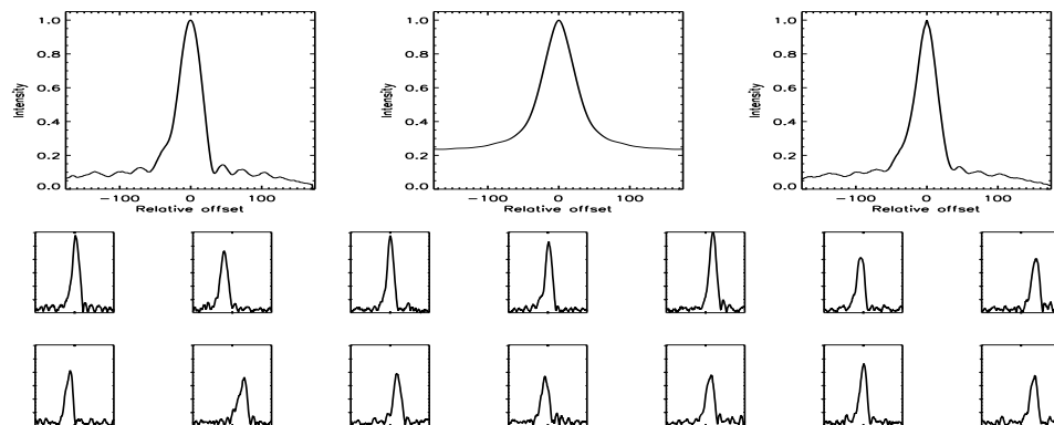
FIGURE B.485: SFP inspection for HD 165401 with S1-W1 on UT 2008/07/07, seq 002
