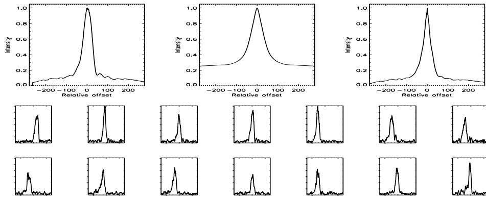
FIGURE B.360: SFP inspection for HD 132254 with S1-E1 on UT 2007/04/11, seq 001
