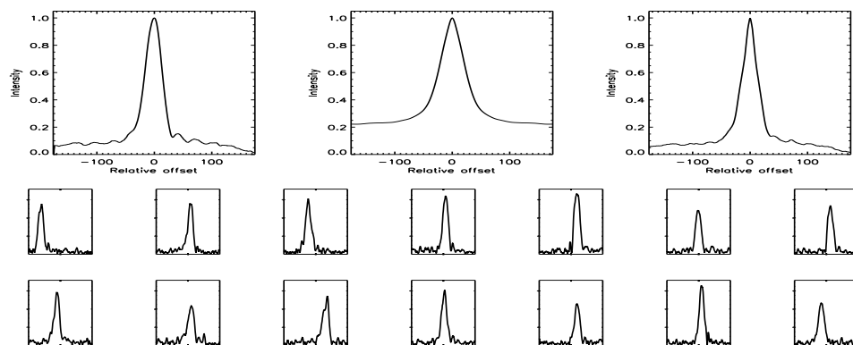
FIGURE B.466: SFP inspection for HD 159222 with S2-W1 on UT 2008/06/24, seq 001
