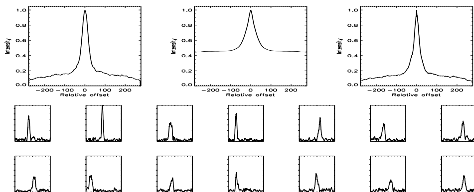
FIGURE B.418: SFP inspection for HD 145675 with E1-W1 on UT 2007/04/26, seq 001
