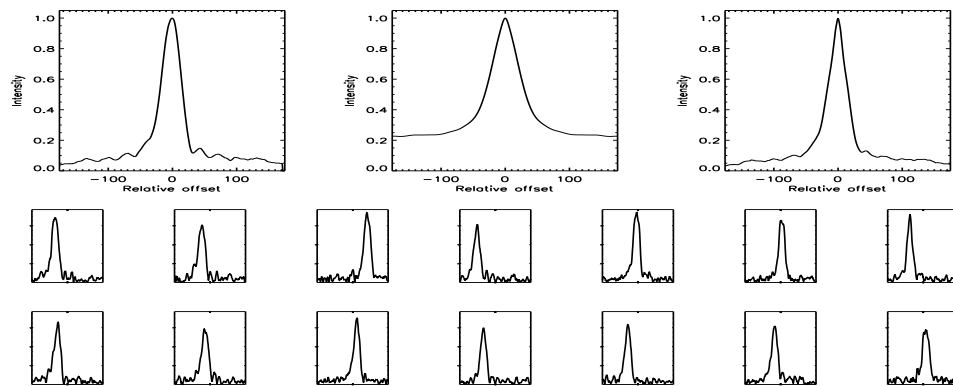
FIGURE B.319: SFP inspection for HD 124292 with S1-W1 on UT 2008/04/13, seq 002
