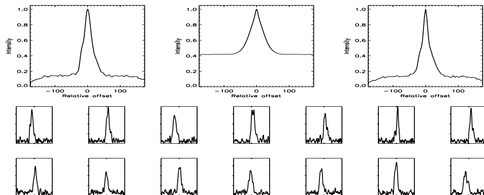
FIGURE B.344: SFP inspection for HD 128642 with S1-E1 on UT 2008/06/25, seq 002
