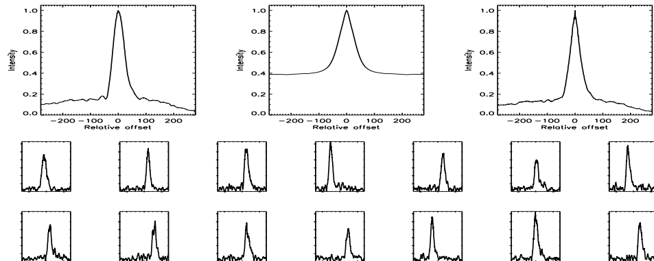
FIGURE B.146: SFP inspection for HD 037394 with S1-E1 on UT 2007/04/14, seq 001
