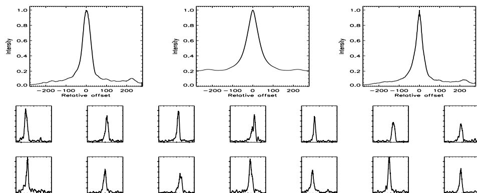
FIGURE B.253: SFP inspection for HD 098230 with S1-W1 on UT 2007/04/24, seq 001
