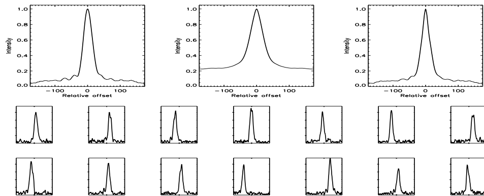
FIGURE B.354: SFP inspection for HD 130307 with S1-W1 on UT 2008/04/13, seq 002
