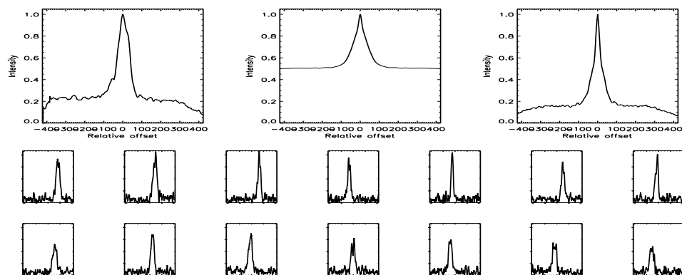
FIGURE B.106: SFP inspection for HD 024409 with S1-E1 on UT 2007/09/16, seq 002
