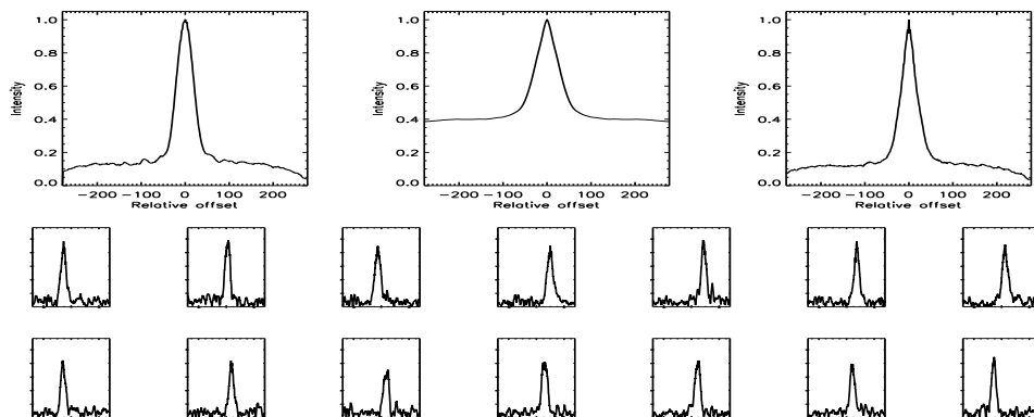
FIGURE B.524: SFP inspection for HD 184385 with S1-W1 on UT 2007/05/30, seq 001
