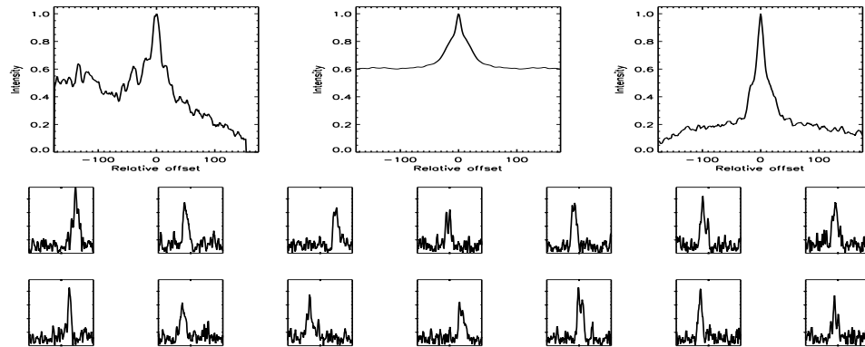
FIGURE B.317: SFP inspection for HD 124292 with S1-E1 on UT 2008/04/13, seq 001
