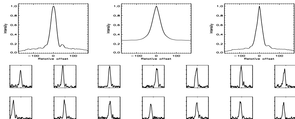
FIGURE B.471: SFP inspection for HD 161198 with S1-W1 on UT 2008/04/13, seq 001
