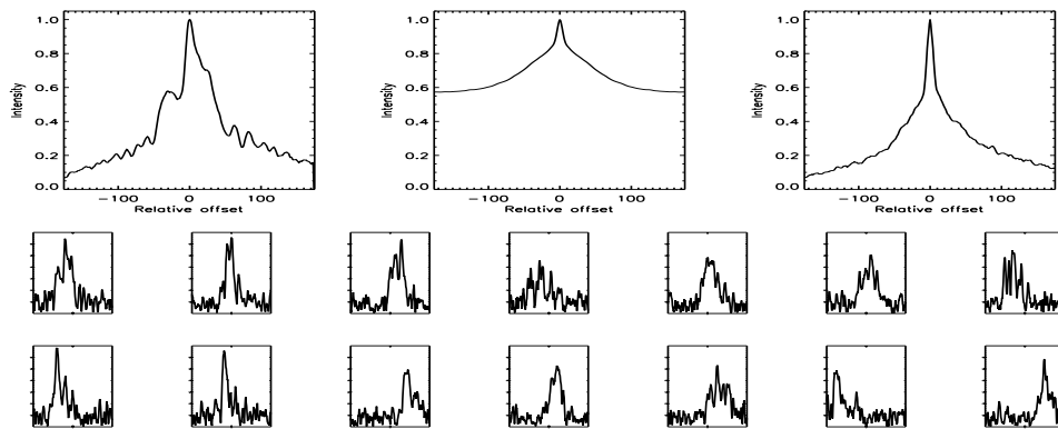
FIGURE B.483: SFP inspection for HD 165401 with S1-W1 on UT 2008/06/22, seq 001
