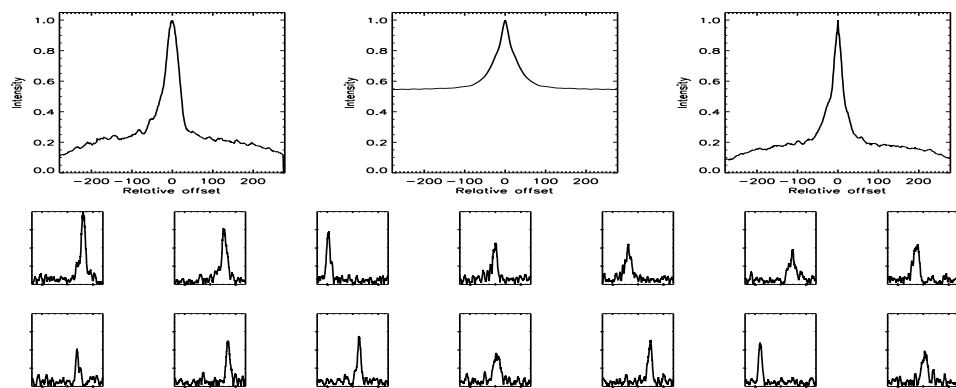
FIGURE B.235: SFP inspection for HD 089269 with S1-W1 on UT 2007/04/24, seq 001
