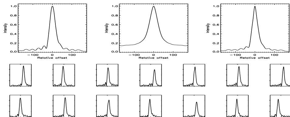
FIGURE B.379: SFP inspection for HD 136202 with S1-W1 on UT 2008/04/13, seq 002
