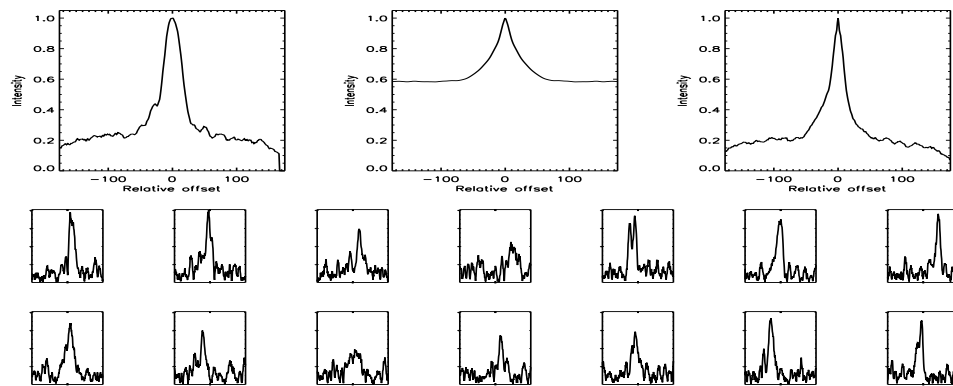
FIGURE B.355: SFP inspection for HD 132142 with S1-E1 on UT 2008/04/12, seq 002
