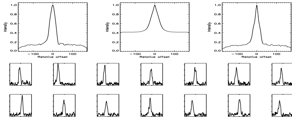
FIGURE B.358: SFP inspection for HD 132142 with S2-W1 on UT 2008/06/24, seq 001
