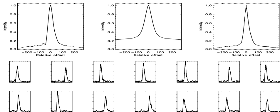
FIGURE B.377: SFP inspection for HD 136202 with S1-E2 on UT 2007/05/31, seq 001
