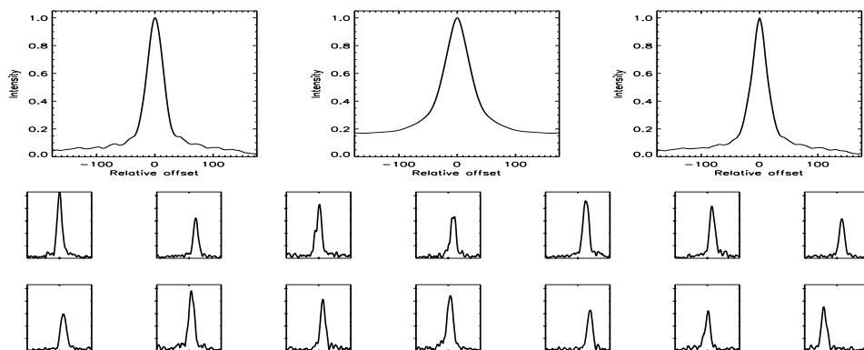
FIGURE B.327: SFP inspection for HD 124850 with S2-W2 on UT 2008/06/09, seq 001
