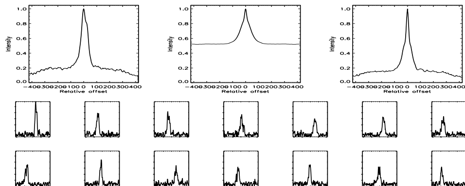
FIGURE B.155: SFP inspection for HD 038230 with S2-E2 on UT 2007/11/27, seq 001
