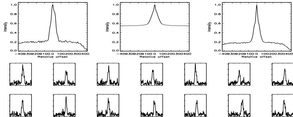
FIGURE B.20: SFP inspection for HD 003765 with S1-E1 on UT 2007/08/16, seq 002
