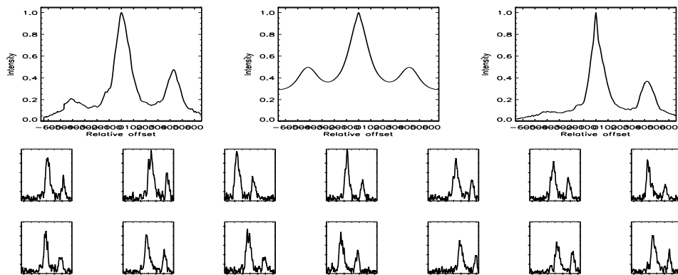
FIGURE B.15: SFP inspection for HD 003196 with S2-E2 on UT 2007/09/27, seq 001
