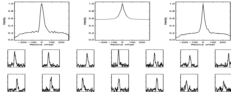
FIGURE B.173: SFP inspection for HD 051866 with S1-E1 on UT 2007/01/25, seq 001
