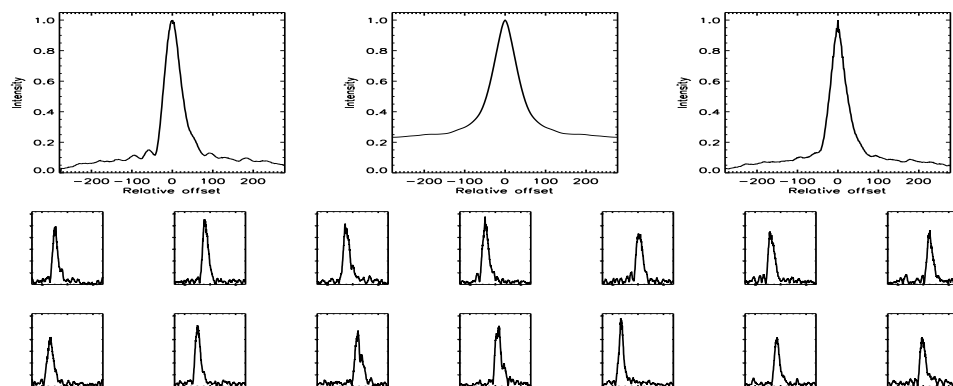
FIGURE B.454: SFP inspection for HD 158633 with S1-E1 on UT 2007/04/14, seq 001
