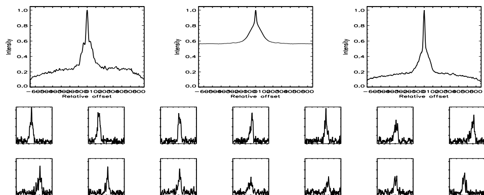
FIGURE B.97: SFP inspection for HD 020619 with S1-E1 on UT 2007/11/01, seq 001
