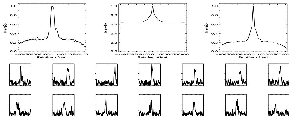
FIGURE B.96: SFP inspection for HD 020165 with S1-W1 on UT 2007/11/01, seq 002
