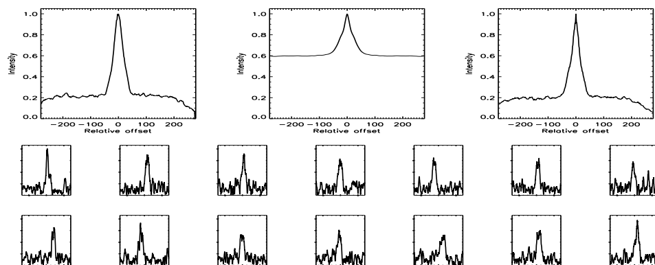
FIGURE B.580: SFP inspection for HD 198425 with S1-E1 on UT 2007/08/14, seq 001
