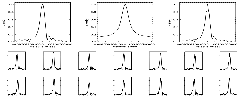
FIGURE B.51: SFP inspection for HD 010476 with S1-E1 on UT 2007/08/16, seq 001
