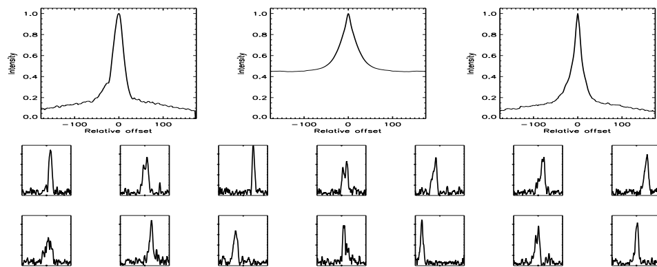
FIGURE B.273: SFP inspection for HD 101206 with S1-W1 on UT 2008/04/12, seq 001
