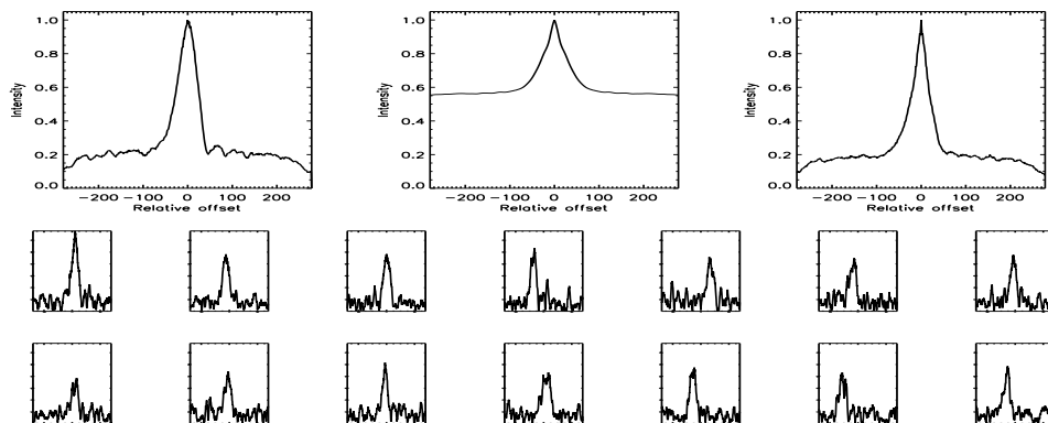
FIGURE B.596: SFP inspection for HD 208313 with S1-W1 on UT 2007/08/14, seq 002
