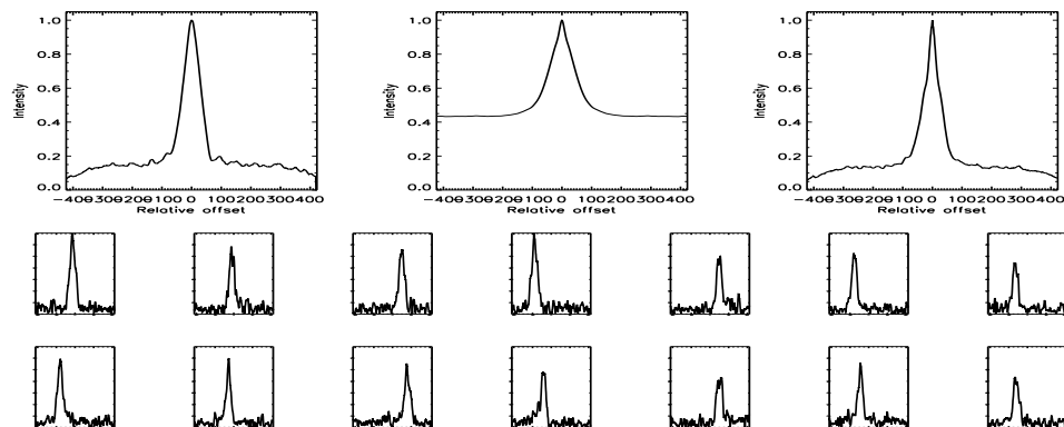
FIGURE B.515: SFP inspection for HD 180161 with S1-E1 on UT 2007/09/16, seq 002
