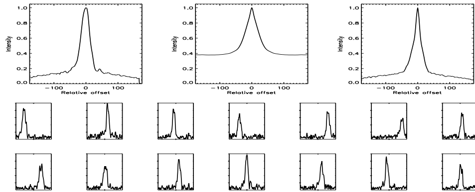
FIGURE B.225: SFP inspection for HD 082443 with S1-W1 on UT 2008/04/12, seq 001
