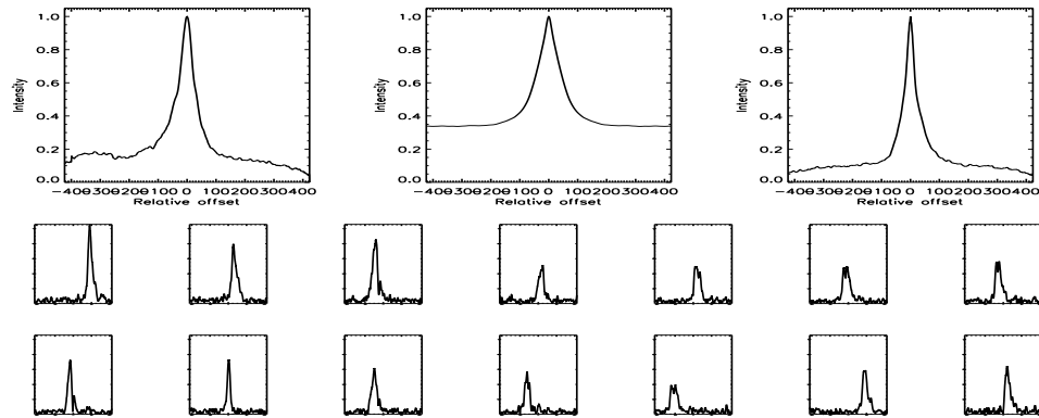
FIGURE B.185: SFP inspection for HD 055575 with S2-E2 on UT 2007/11/27, seq 002
