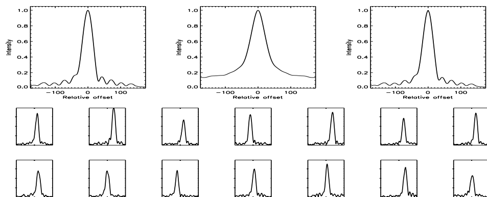
FIGURE B.424: SFP inspection for HD 146233 with S1-W1 on UT 2008/04/14, seq 001
