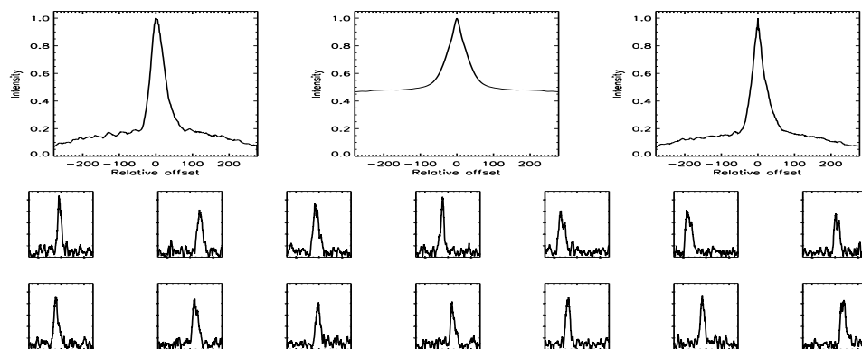
FIGURE B.373: SFP inspection for HD 135599 with S1-E2 on UT 2007/05/31, seq 001
