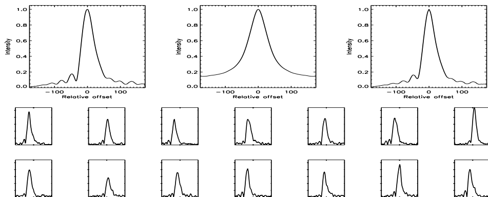
FIGURE B.326: SFP inspection for HD 124850 with S1-W1 on UT 2008/07/08, seq 001
