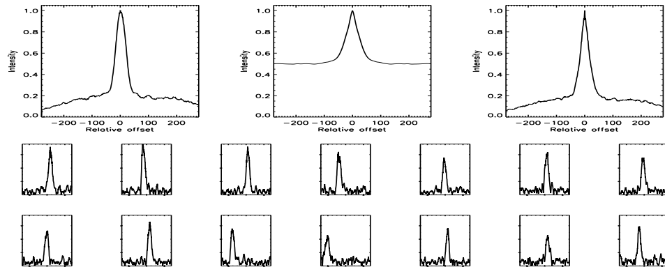
FIGURE B.35: SFP inspection for HD 007590 with S1-E1 on UT 2007/02/04, seq 002
