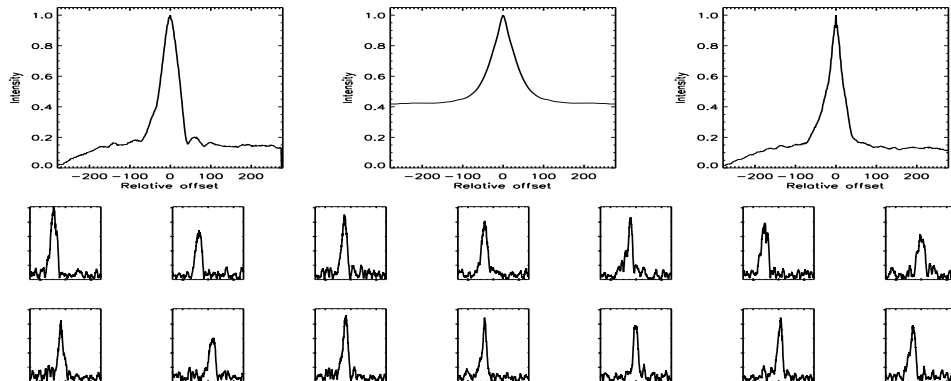
FIGURE B.296: SFP inspection for HD 115404 with S1-E1 on UT 2007/02/06, seq 002
