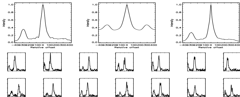
FIGURE B.16: SFP inspection for HD 003196 with S2-W1 on UT 2007/09/17, seq 001
