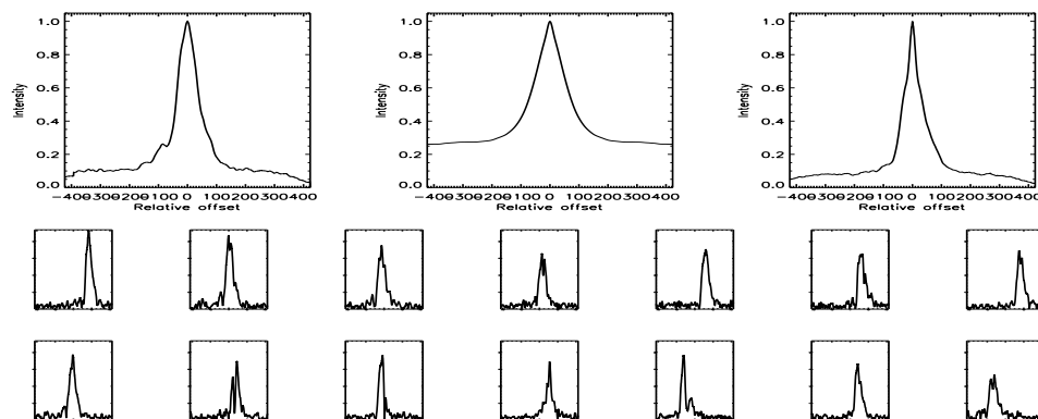
FIGURE B.147: SFP inspection for HD 037394 with S1-W1 on UT 2007/11/01, seq 001
