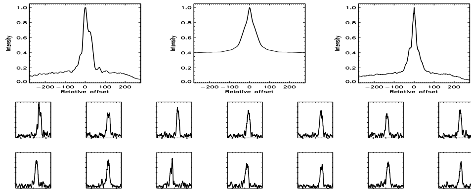
FIGURE B.152: SFP inspection for HD 038230 with S1-E1 on UT 2007/01/25, seq 001
