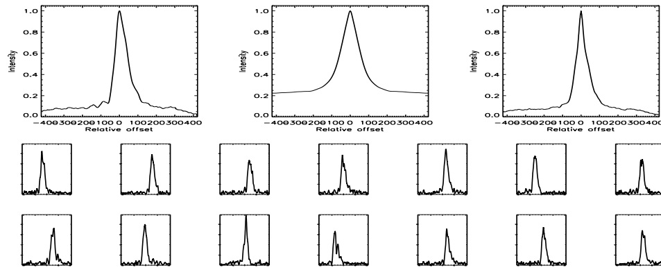
FIGURE B.183: SFP inspection for HD 055575 with S1-W1 on UT 2007/11/01, seq 001
