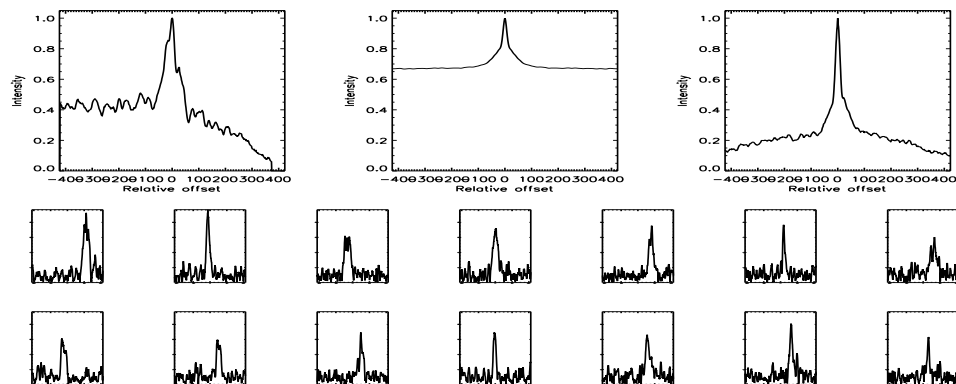
FIGURE B.95: SFP inspection for HD 020165 with S1-E1 on UT 2007/11/01, seq 001
