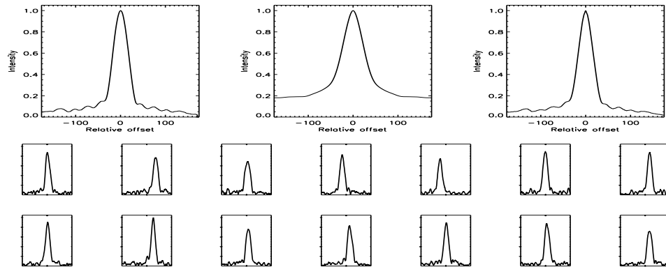
FIGURE B.5: SFP inspection for HD 001461 with S1-W1 on UT 2008/07/27, seq 001
