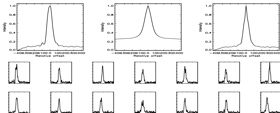
FIGURE B.555: SFP inspection for HD 190771 with S1-W1 on UT 2007/08/21, seq 001
