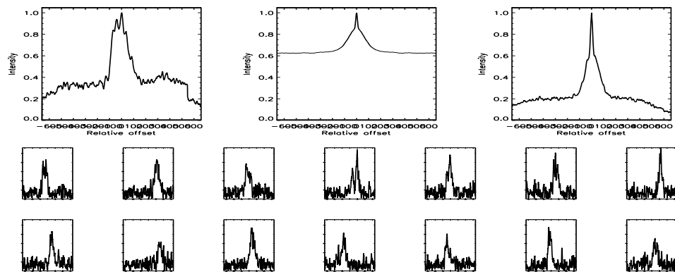
FIGURE B.46: SFP inspection for HD 010008 with S2-E2 on UT 2007/09/27, seq 001
