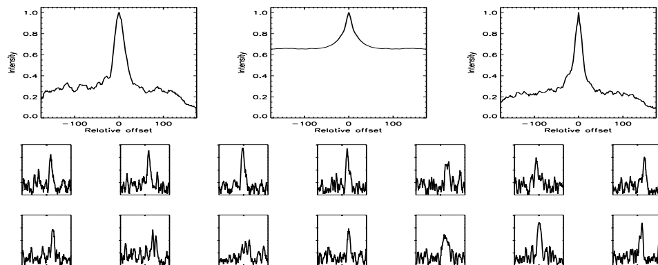
FIGURE B.329: SFP inspection for HD 125455 with S1-E1 on UT 2008/04/14, seq 001
