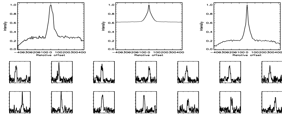
FIGURE B.61: SFP inspection for HD 012846 with S2-E2 on UT 2007/09/18, seq 001
