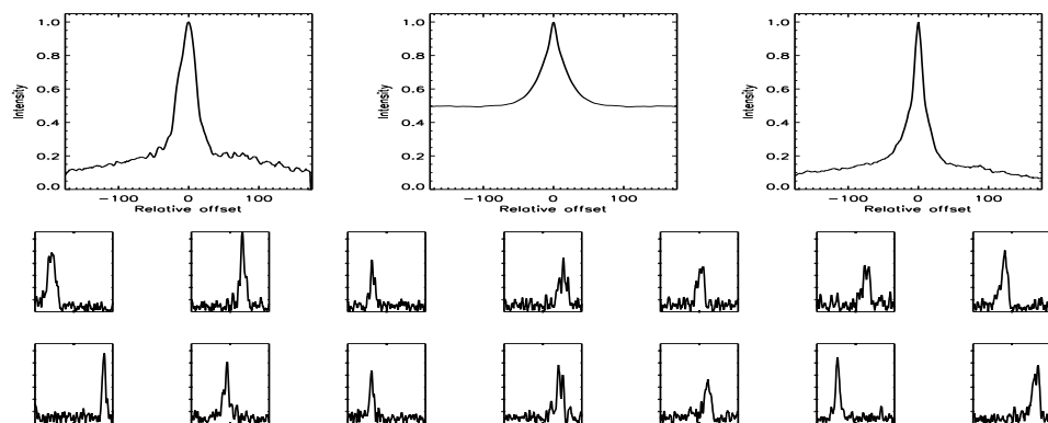
FIGURE B.565: SFP inspection for HD 192263 with S1-E1 on UT 2008/04/25, seq 001
