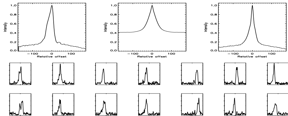
FIGURE B.180: SFP inspection for HD 054371 with S1-W1 on UT 2008/04/26, seq 001
