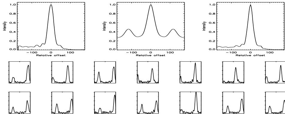
FIGURE B.14: SFP inspection for HD 003196 with S1-W1 on UT 2008/07/07, seq 001
