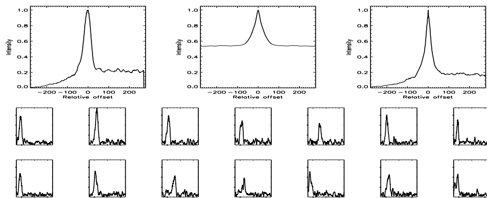
FIGURE B.171: SFP inspection for HD 051419 with S1-E1 on UT 2007/02/05, seq 003
