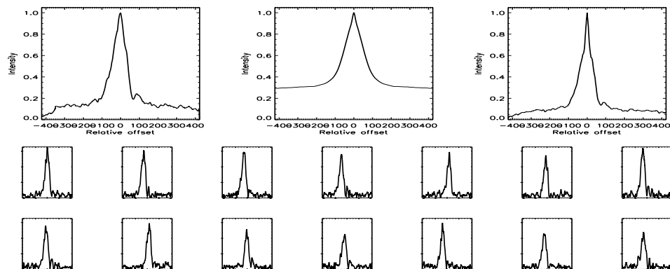
FIGURE B.644: SFP inspection for HD 222143 with S1-E1 on UT 2007/07/27, seq 001
