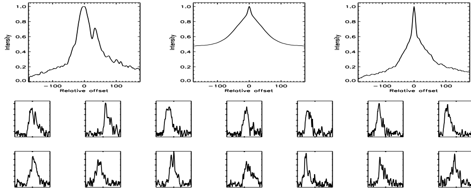
FIGURE B.368: SFP inspection for HD 135204 with S1-W1 on UT 2008/06/22, seq 002
