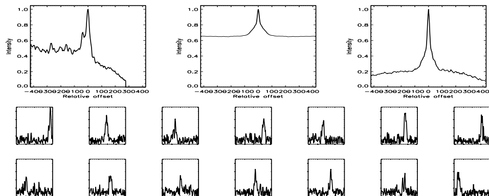
FIGURE B.164: SFP inspection for HD 042618 with S1-E1 on UT 2007/10/31, seq 001
