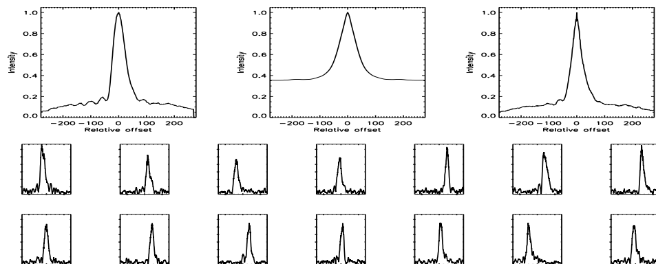
FIGURE B.167: SFP inspection for HD 046588 with S1-E1 on UT 2007/04/14, seq 001
