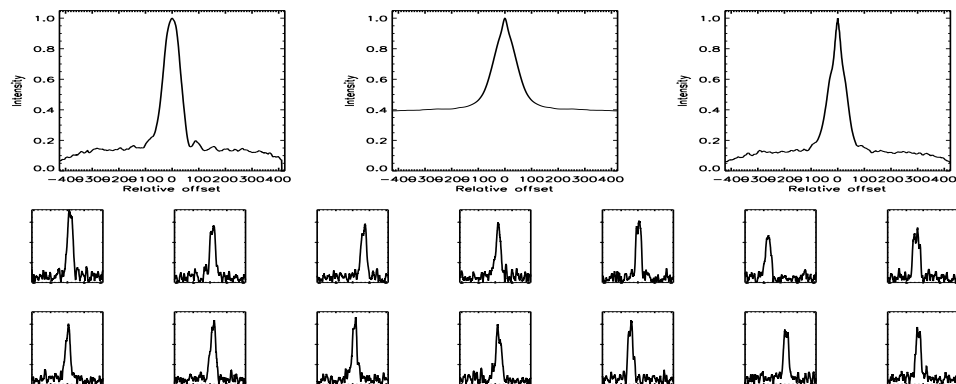
FIGURE B.518: SFP inspection for HD 180161 with S2-E1 on UT 2007/08/20, seq 001
