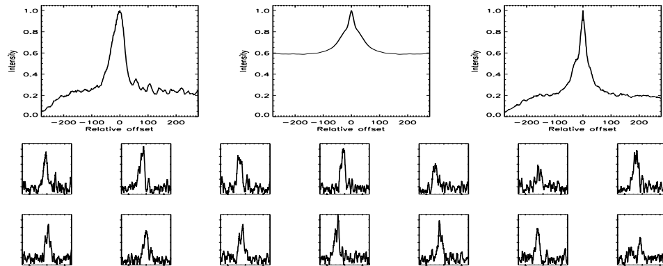
FIGURE B.125: SFP inspection for HD 026923 with S2-E2 on UT 2007/09/26, seq 001
