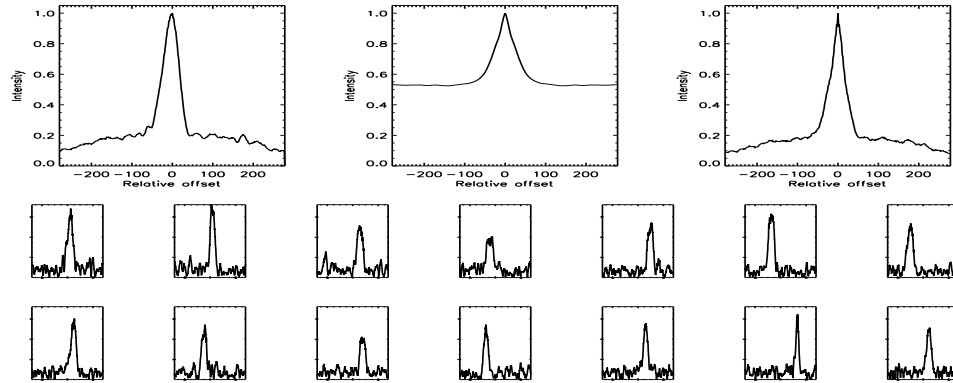
FIGURE B.476: SFP inspection for HD 165401 with S1-E1 on UT 2007/07/22, seq 002
