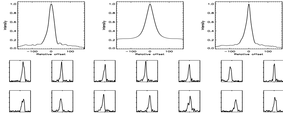
FIGURE B.56: SFP inspection for HD 010780 with S2-W1 on UT 2008/06/24, seq 001
