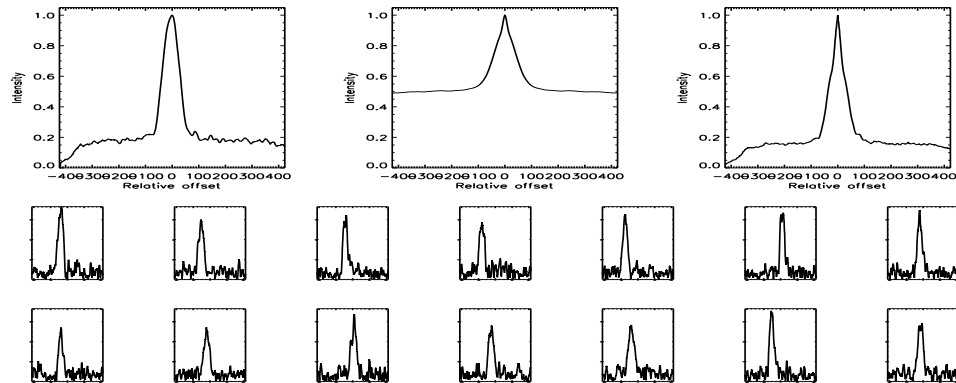
FIGURE B.551: SFP inspection for HD 190470 with S1-W1 on UT 2007/08/18, seq 001
