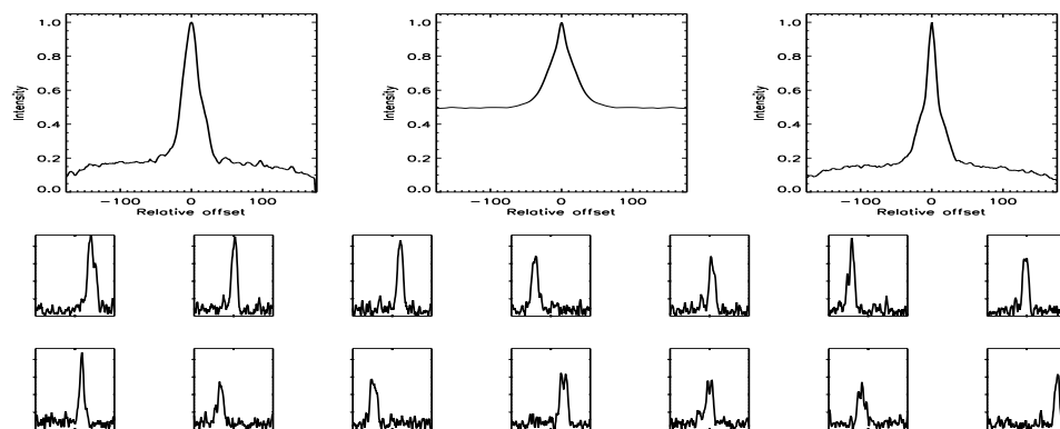
FIGURE B.481: SFP inspection for HD 165401 with S1-E1 on UT 2008/07/05, seq 002
