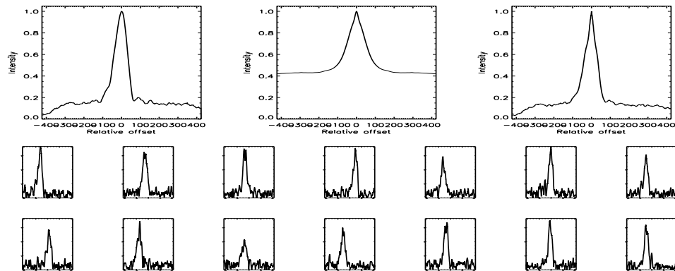
FIGURE B.586: SFP inspection for HD 200560 with S1-W1 on UT 2007/08/18, seq 001
