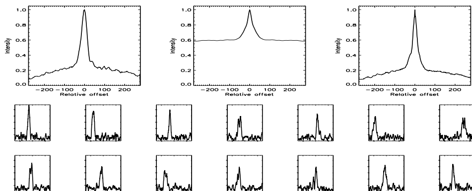
FIGURE B.414: SFP inspection for HD 142267 with S1-E2 on UT 2007/06/01, seq 001
