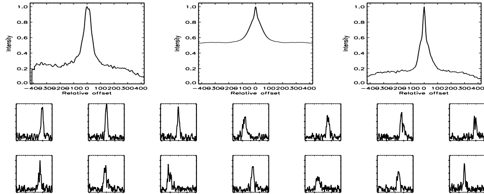
FIGURE B.140: SFP inspection for HD 037008 with S1-W1 on UT 2007/11/01, seq 002
