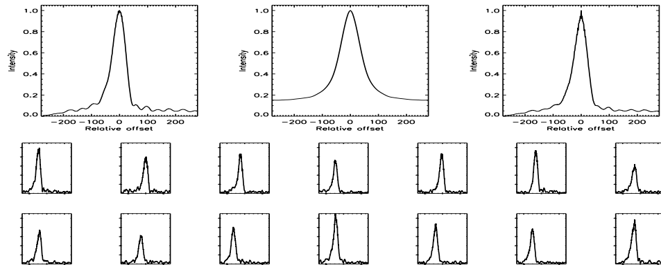
FIGURE B.251: SFP inspection for HD 098230 with S1-E1 on UT 2007/05/17, seq 003
