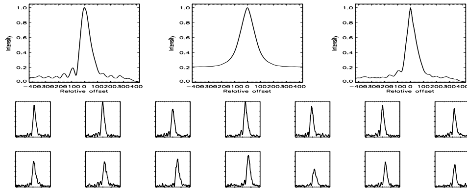
FIGURE B.93: SFP inspection for HD 019994 with S2-E2 on UT 2007/09/27, seq 002
