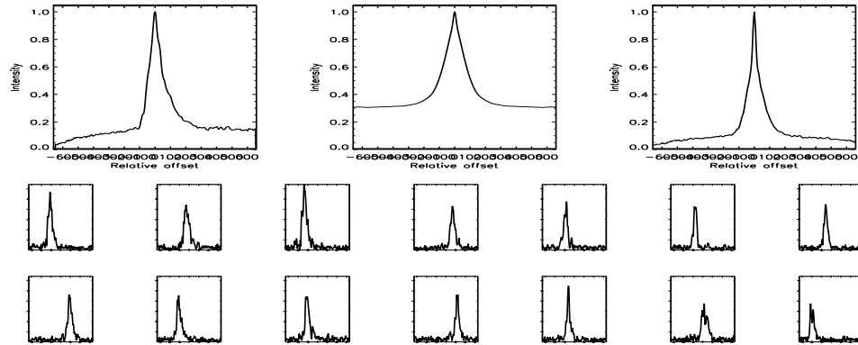
FIGURE B.74: SFP inspection for HD 016765 with S2-W1 on UT 2007/09/17, seq 001
