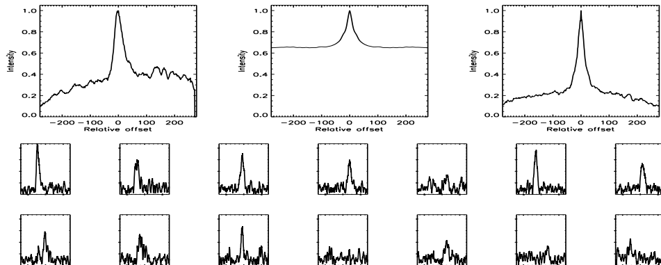
FIGURE B.401: SFP inspection for HD 139341 with S1-W1 on UT 2007/04/17, seq 002
