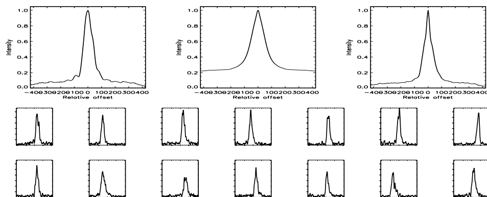
FIGURE B.133: SFP inspection for HD 032923 with S1-E1 on UT 2007/10/31, seq 001
