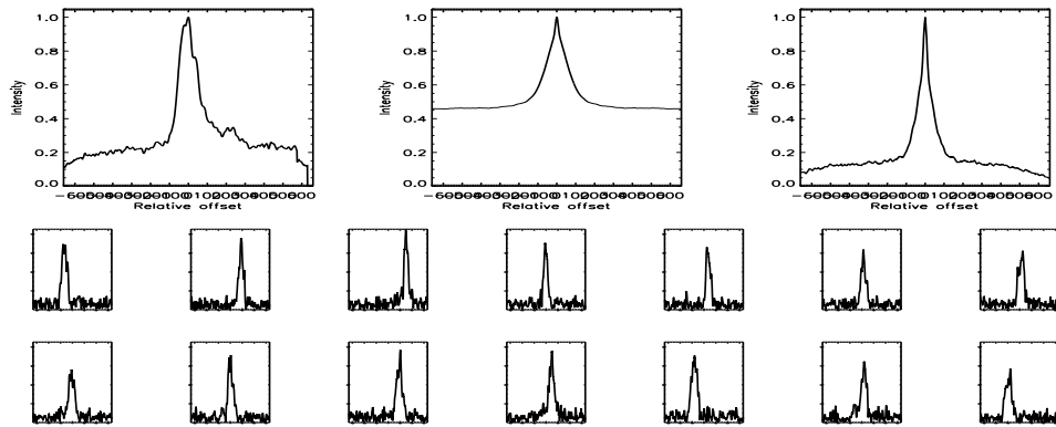
FIGURE B.30: SFP inspection for HD 004635 with S2-E1 on UT 2007/08/20, seq 001
