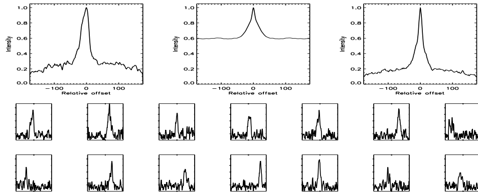
FIGURE B.623: SFP inspection for HD 218868 with S1-E1 on UT 2008/06/25, seq 001
