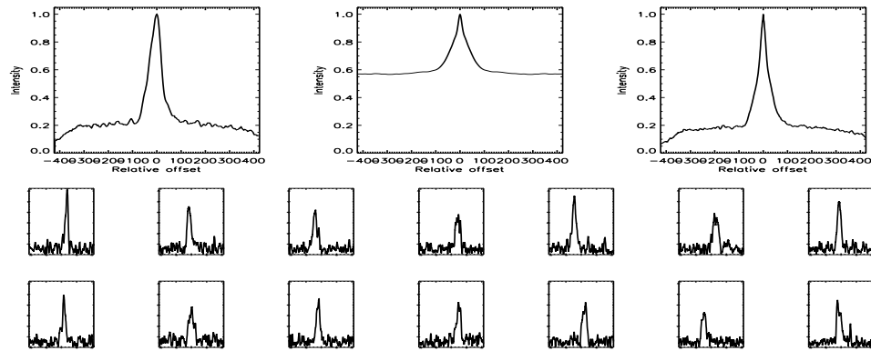
FIGURE B.585: SFP inspection for HD 200560 with S1-E1 on UT 2007/08/18, seq 002
