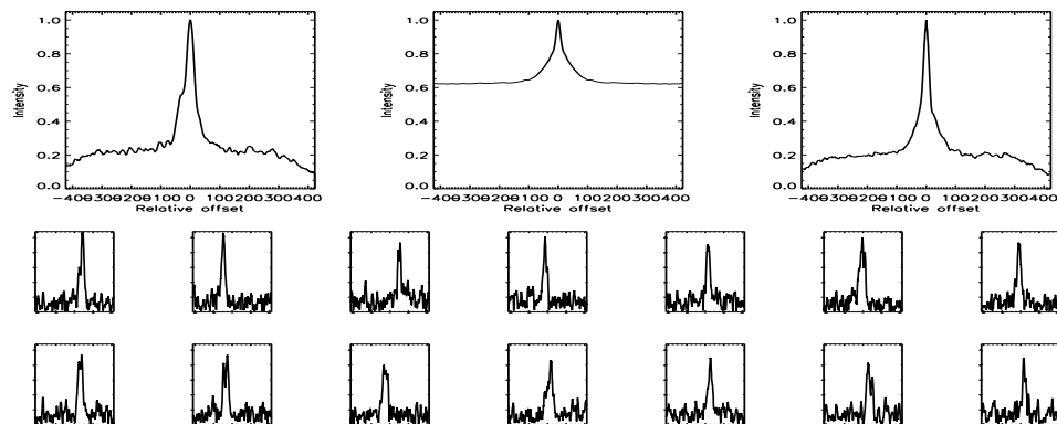
FIGURE B.104: SFP inspection for HD 024238 with S1-E1 on UT 2007/09/16, seq 002
