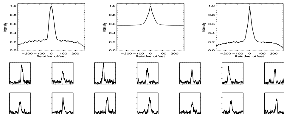
FIGURE B.609: SFP inspection for HD 211472 with S1-W1 on UT 2007/07/26, seq 002
