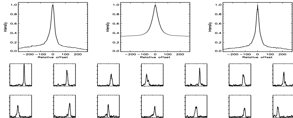
FIGURE B.320: SFP inspection for HD 124850 with S1-E1 on UT 2007/02/16, seq 001
