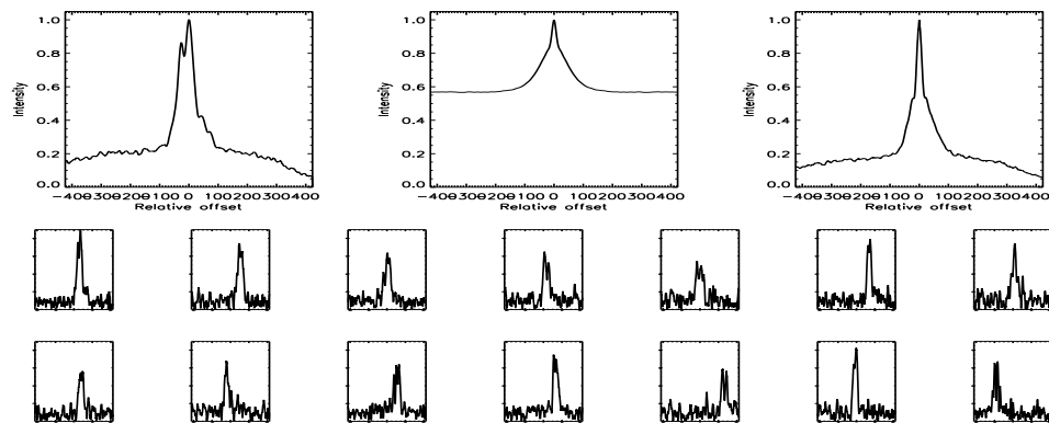
FIGURE B.79: SFP inspection for HD 018143 with S1-E1 on UT 2007/10/31, seq 001
