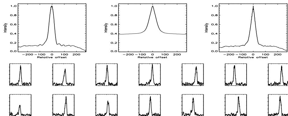
FIGURE B.474: SFP inspection for HD 164922 with S1-E1 on UT 2007/05/17, seq 001
