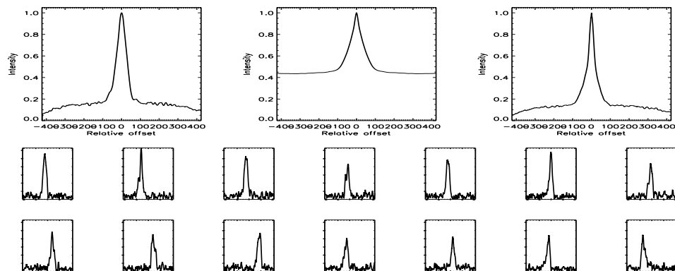
FIGURE B.488: SFP inspection for HD 166620 with S2-E2 on UT 2007/09/18, seq 001
