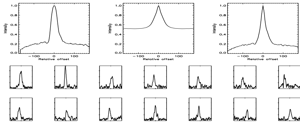
FIGURE B.39: SFP inspection for HD 007590 with S1-W1 on UT 2008/07/08, seq 001
