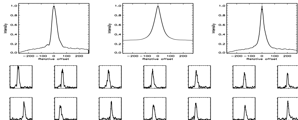
FIGURE B.335: SFP inspection for HD 127334 with S1-W1 on UT 2007/04/17, seq 002
