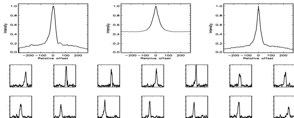
FIGURE B.336: SFP inspection for HD 128165 with E1-W1 on UT 2007/04/26, seq 001
