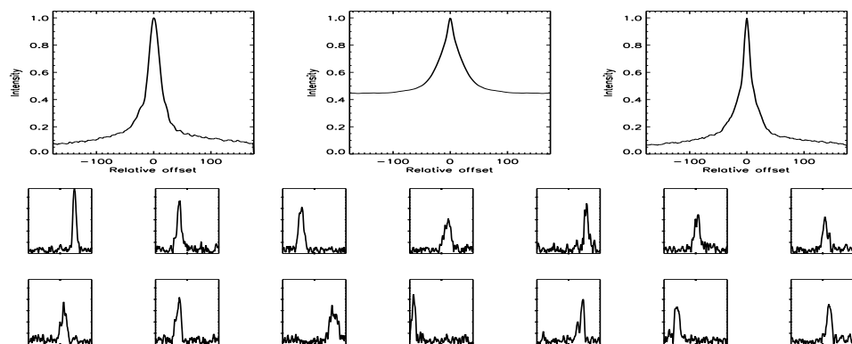
FIGURE B.232: SFP inspection for HD 087883 with S1-W1 on UT 2008/04/26, seq 001
