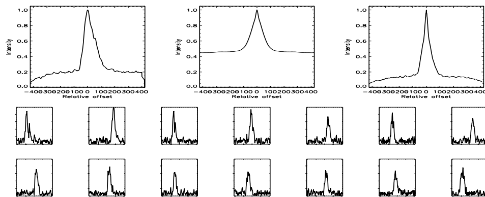
FIGURE B.612: SFP inspection for HD 215152 with S2-W1 on UT 2007/09/17, seq 001
