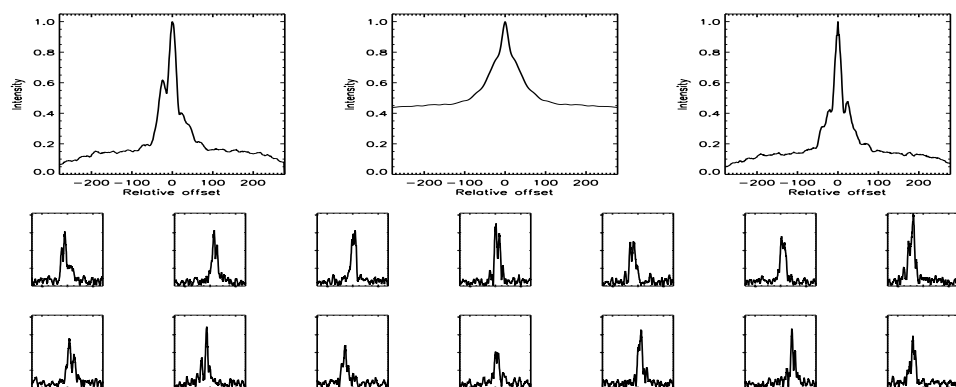
FIGURE B.144: SFP inspection for HD 037394 with S1-E1 on UT 2007/01/25, seq 001
