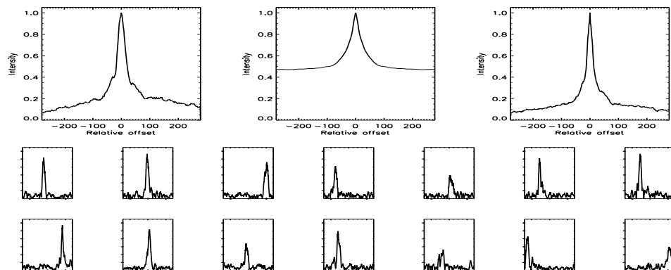
FIGURE B.374: SFP inspection for HD 136202 with S1-E1 on UT 2007/02/16, seq 001
