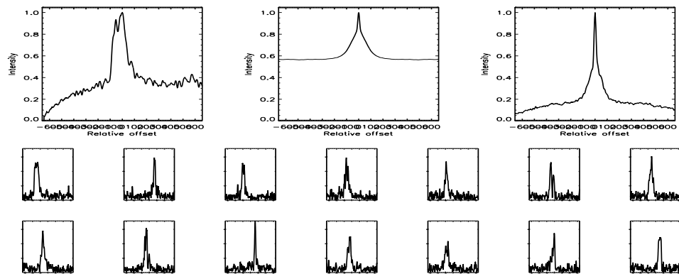
FIGURE B.45: SFP inspection for HD 008997 with S2-W1 on UT 2007/09/17, seq 001
