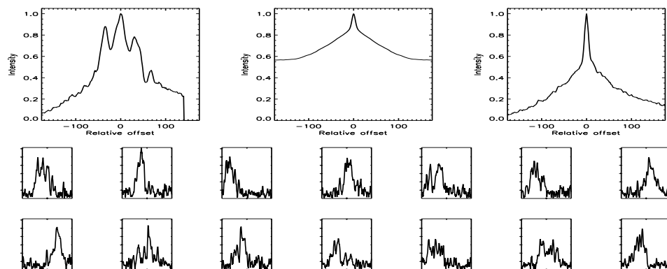
FIGURE B.600: SFP inspection for HD 210277 with S1-W1 on UT 2008/06/22, seq 001
