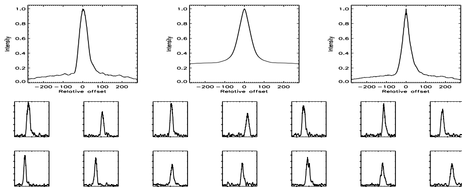
FIGURE B.256: SFP inspection for HD 098230 with S1-W1 on UT 2007/06/01, seq 002
