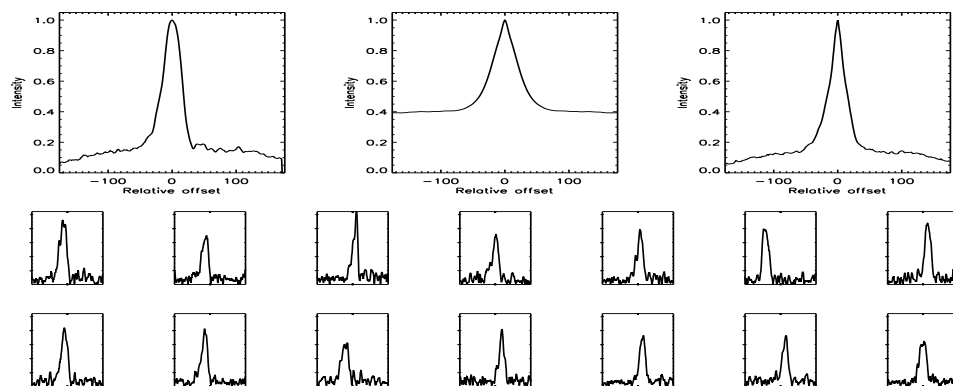
FIGURE B.493: SFP inspection for HD 175742 with S1-W1 on UT 2008/04/13, seq 001
