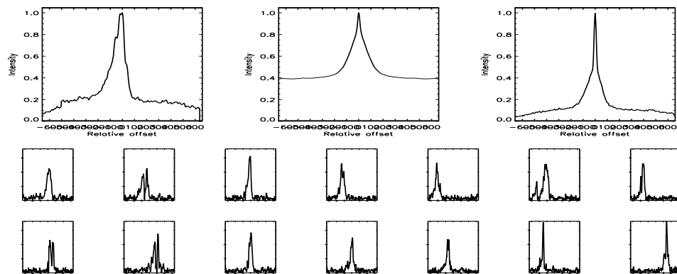
FIGURE B.541: SFP inspection for HD 189733 with S2-W1 on UT 2007/09/17, seq 001
