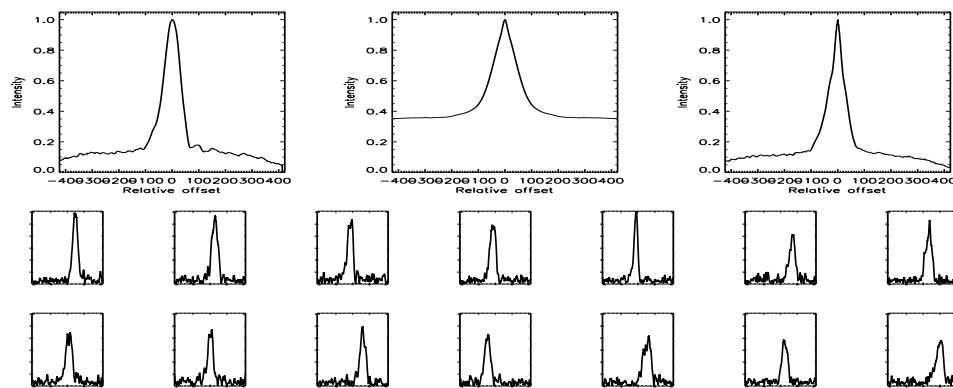
FIGURE B.189: SFP inspection for HD 063433 with S1-W1 on UT 2007/11/01, seq 001
