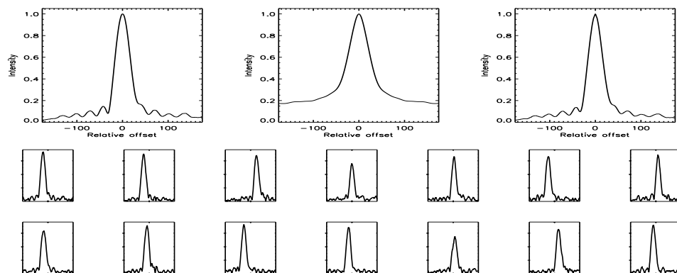
FIGURE B.450: SFP inspection for HD 157347 with S1-W1 on UT 2008/04/14, seq 001
