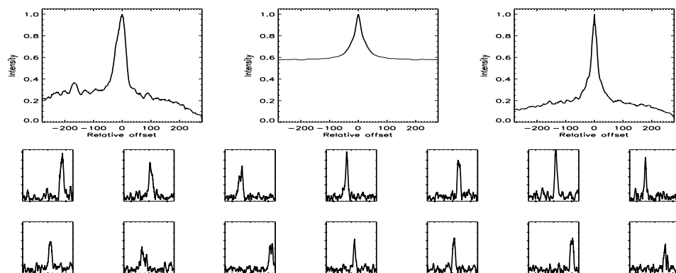
FIGURE B.262: SFP inspection for HD 099491 with S1-E1 on UT 2007/03/08, seq 001
