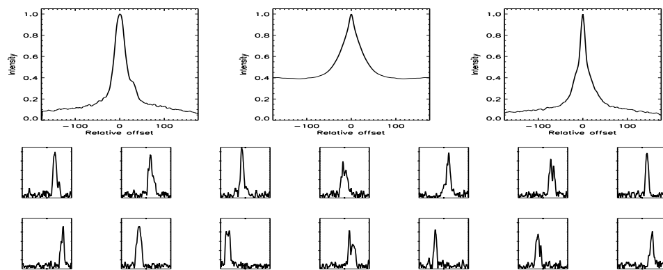
FIGURE B.172: SFP inspection for HD 051419 with S1-W1 on UT 2008/04/26, seq 001
