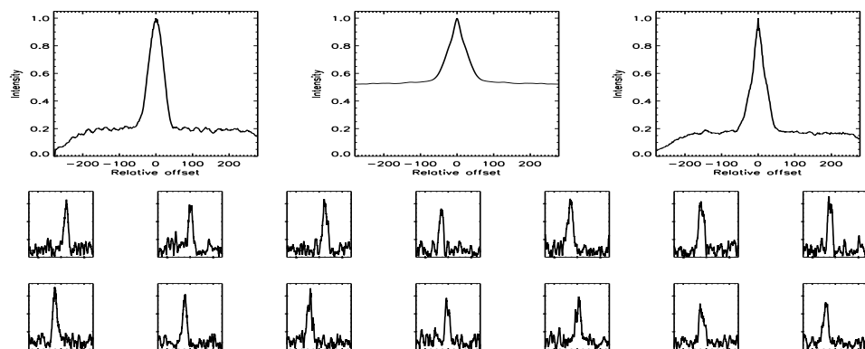
FIGURE B.589: SFP inspection for HD 202751 with S1-W1 on UT 2007/07/24, seq 001
