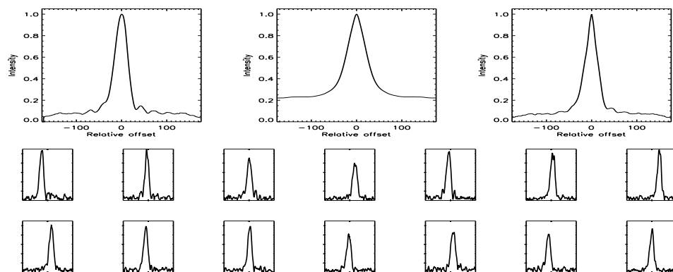
FIGURE B.445: SFP inspection for HD 155712 with S1-W1 on UT 2008/04/13, seq 001
