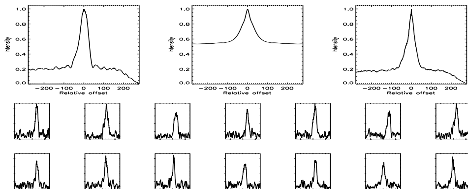
FIGURE B.404: SFP inspection for HD 139777 with S1-W1 on UT 2007/05/28, seq 001
