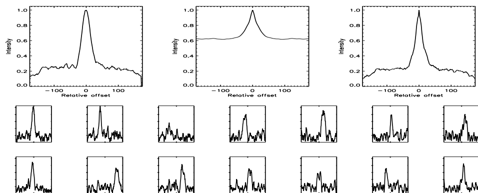
FIGURE B.43: SFP inspection for HD 008997 with S1-W1 on UT 2008/07/07, seq 001
