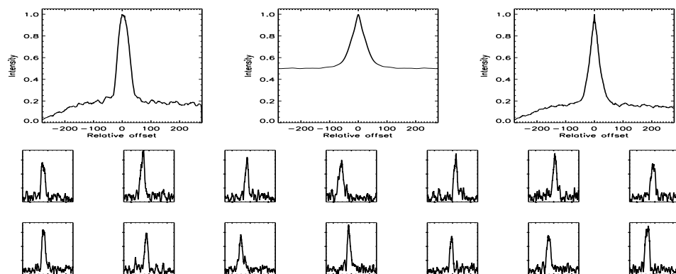
FIGURE B.34: SFP inspection for HD 007590 with S1-E1 on UT 2007/02/04, seq 001
