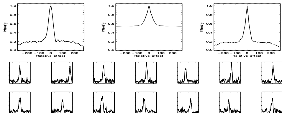
FIGURE B.606: SFP inspection for HD 210667 with S1-W1 on UT 2007/07/26, seq 002
