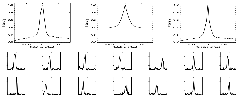
FIGURE B.324: SFP inspection for HD 124850 with S1-E2 on UT 2008/06/08, seq 001
