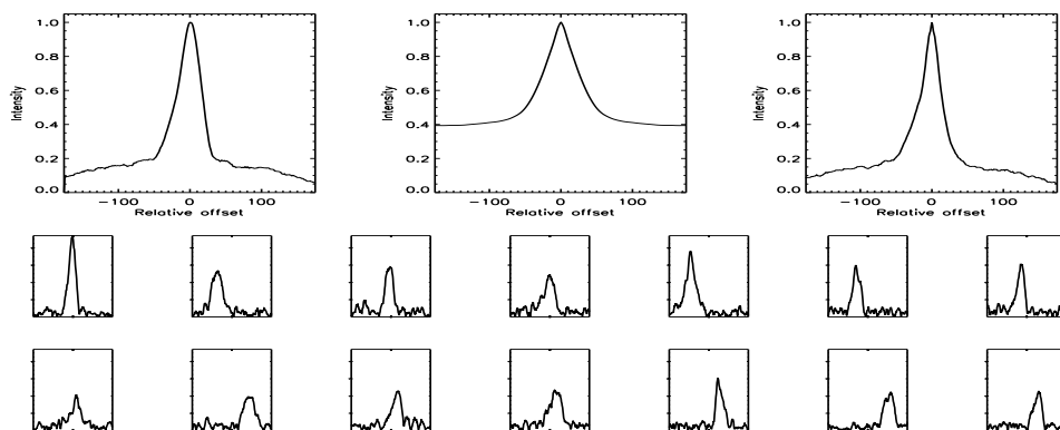
FIGURE B.598: SFP inspection for HD 210277 with S1-E1 on UT 2008/07/06, seq 001
