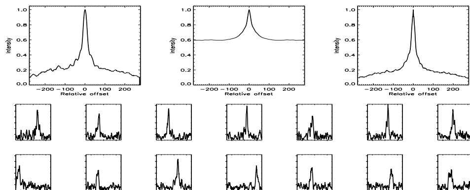
FIGURE B.216: SFP inspection for HD 079969 with S1-E1 on UT 2007/02/25, seq 001
