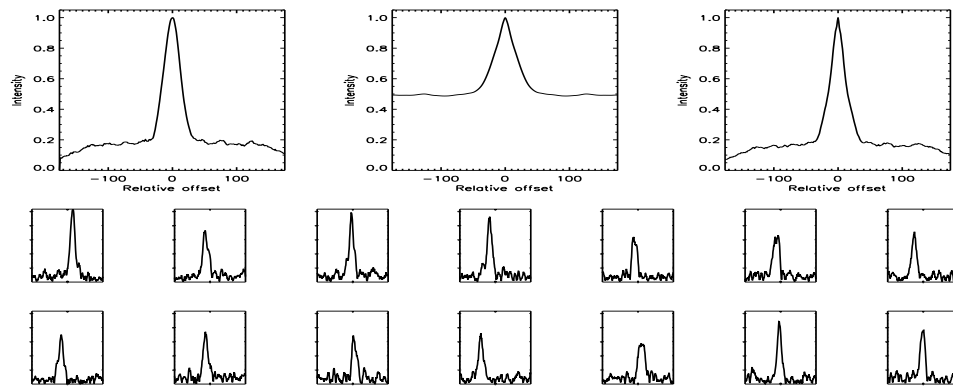
FIGURE B.537: SFP inspection for HD 189340 with S2-W2 on UT 2008/06/09, seq 001
