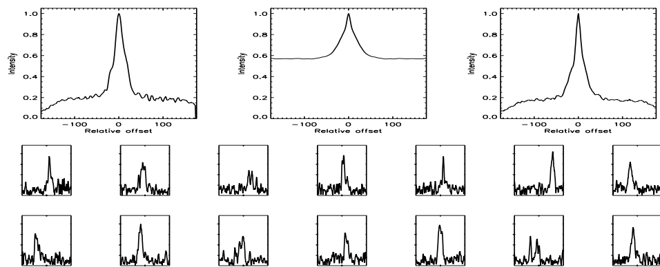
FIGURE B.21: SFP inspection for HD 003765 with S1-E1 on UT 2008/07/09, seq 001
