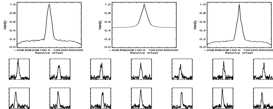
FIGURE B.635: SFP inspection for HD 220182 with S1-E1 on UT 2007/08/18, seq 002
