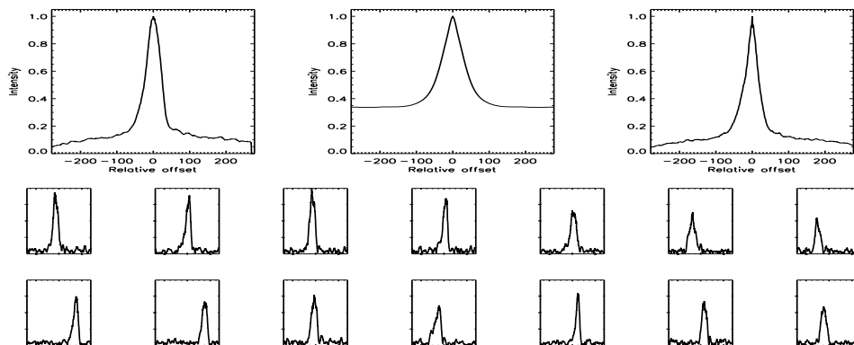
FIGURE B.323: SFP inspection for HD 124850 with S1-E2 on UT 2007/05/31, seq 001
