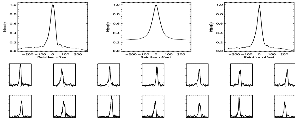
FIGURE B.362: SFP inspection for HD 135204 with S1-E1 on UT 2007/03/08, seq 001
