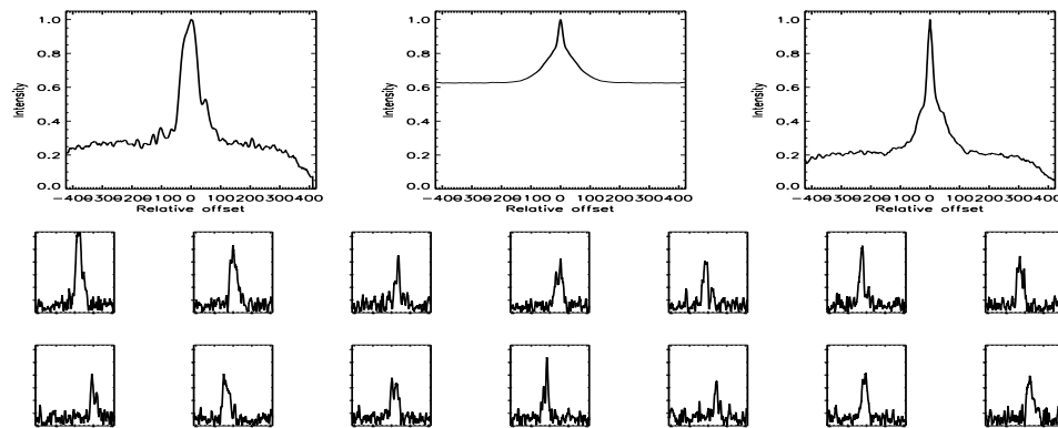
FIGURE B.81: SFP inspection for HD 018143 with S1-W1 on UT 2007/11/01, seq 001
