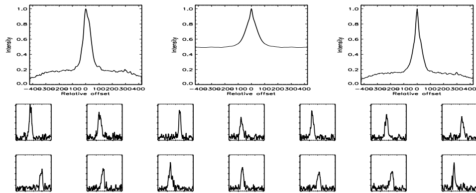
FIGURE B.186: SFP inspection for HD 059747 with S1-W1 on UT 2007/11/01, seq 001
