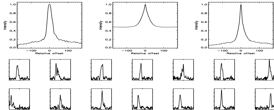
FIGURE B.191: SFP inspection for HD 065430 with S1-W1 on UT 2008/04/26, seq 001
