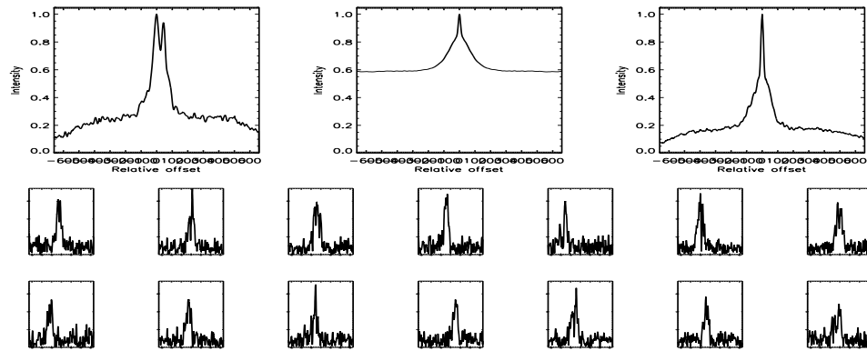
FIGURE B.447: SFP inspection for HD 155712 with S2-W1 on UT 2007/09/17, seq 001
