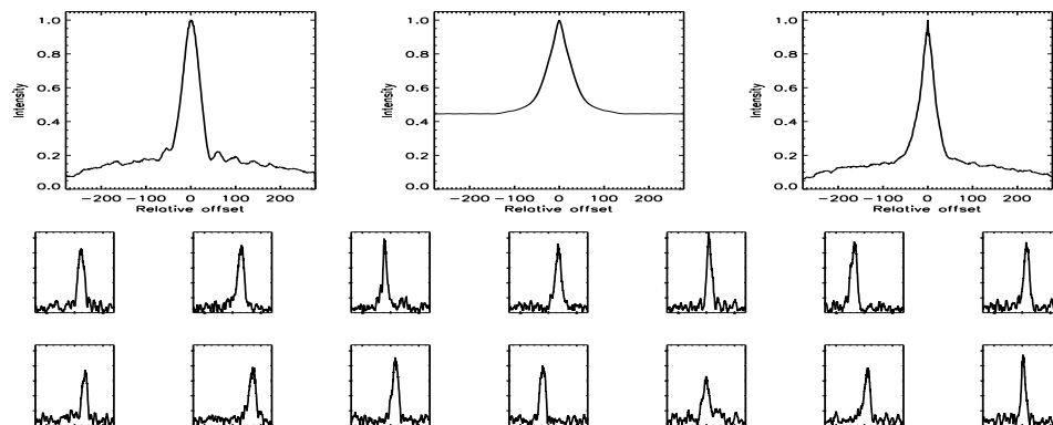
FIGURE B.458: SFP inspection for HD 159062 with S1-E1 on UT 2007/04/14, seq 001
