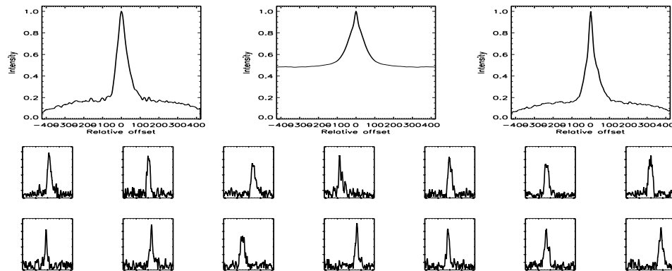
FIGURE B.226: SFP inspection for HD 082443 with S2-E2 on UT 2007/11/29, seq 001
