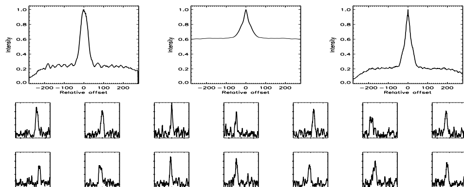
FIGURE B.591: SFP inspection for HD 208038 with S1-E1 on UT 2007/07/24, seq 002
