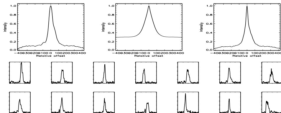
FIGURE B.168: SFP inspection for HD 046588 with S1-E1 on UT 2007/09/16, seq 001
