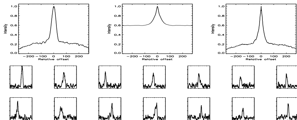
FIGURE B.475: SFP inspection for HD 164922 with S1-E2 on UT 2007/05/31, seq 001
