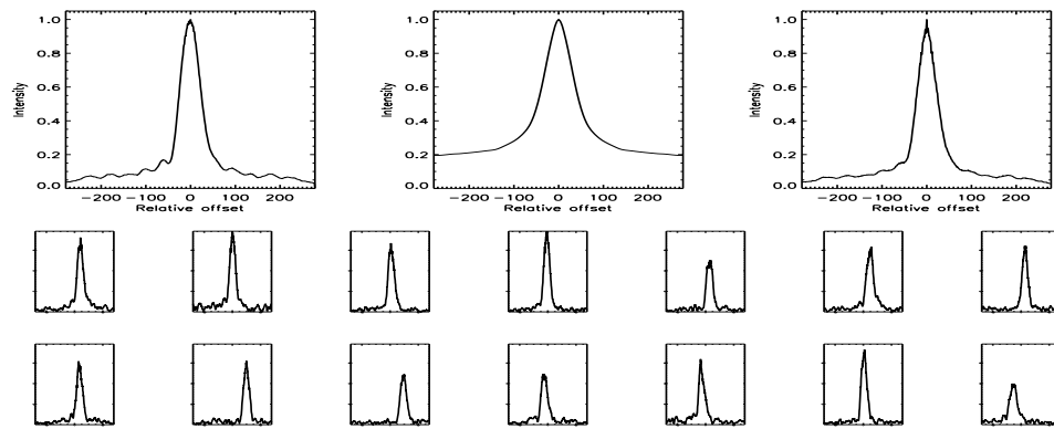
FIGURE B.627: SFP inspection for HD 219134 with S1-W1 on UT 2007/07/26, seq 003
