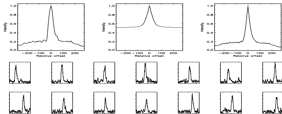
FIGURE B.270: SFP inspection for HD 101177 with S1-E1 on UT 2007/05/17, seq 001
