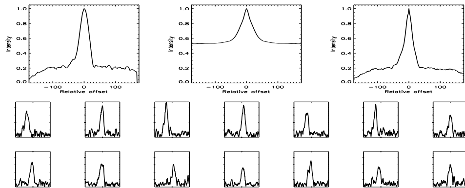
FIGURE B.192: SFP inspection for HD 065583 with S1-E1 on UT 2008/04/13, seq 001
