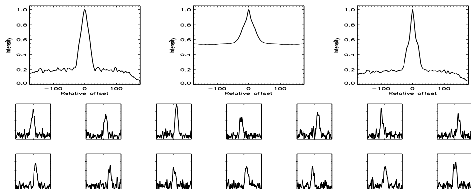
FIGURE B.42: SFP inspection for HD 008997 with S1-E1 on UT 2008/07/23, seq 001
