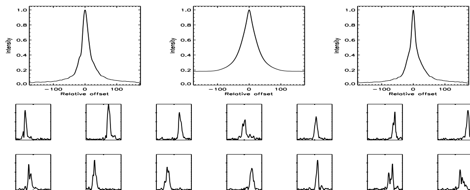
FIGURE B.229: SFP inspection for HD 082885 with S1-W1 on UT 2008/04/26, seq 001
