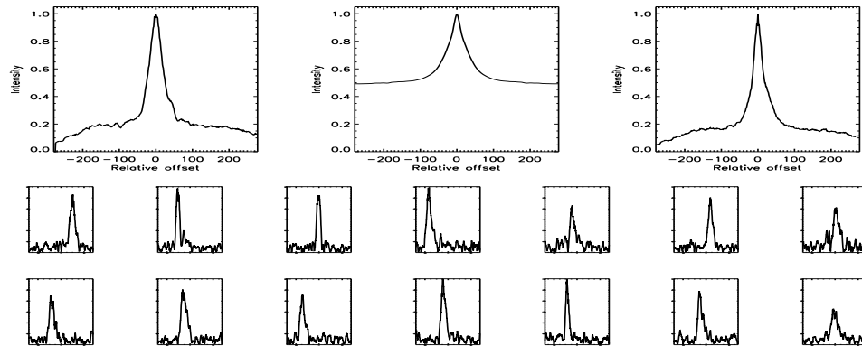
FIGURE B.197: SFP inspection for HD 067228 with S2-E2 on UT 2007/11/29, seq 003
