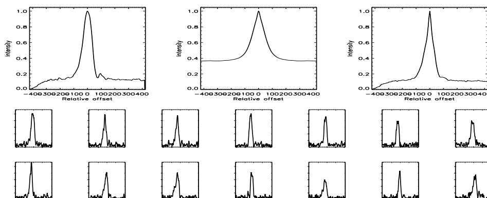
FIGURE B.546: SFP inspection for HD 190404 with S1-W1 on UT 2007/07/24, seq 002
