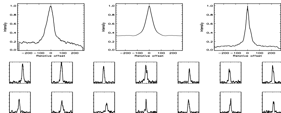
FIGURE B.456: SFP inspection for HD 158633 with S1-W1 on UT 2007/04/17, seq 002
