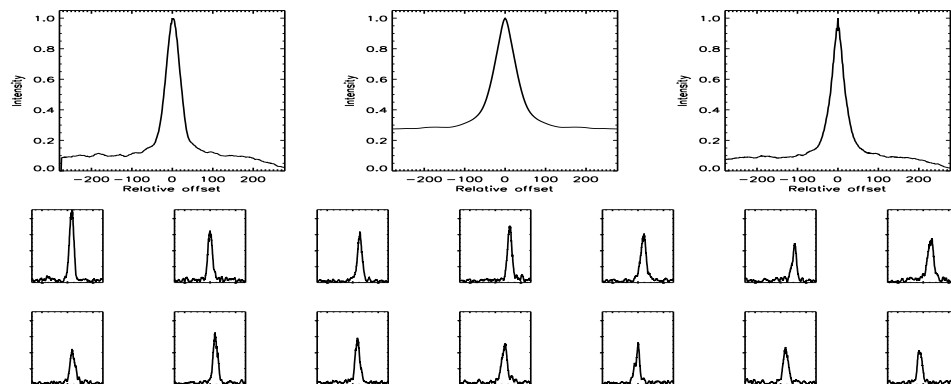
FIGURE B.455: SFP inspection for HD 158633 with S1-W1 on UT 2007/04/17, seq 001
