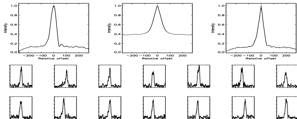
FIGURE B.620: SFP inspection for HD 217813 with S1-W1 on UT 2007/08/14, seq 002
