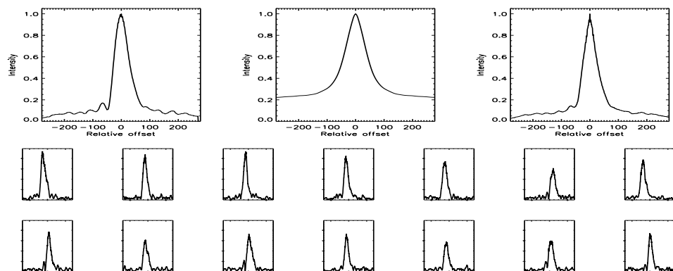
FIGURE B.18: SFP inspection for HD 003651 with S1-E1 on UT 2007/08/14, seq 001
