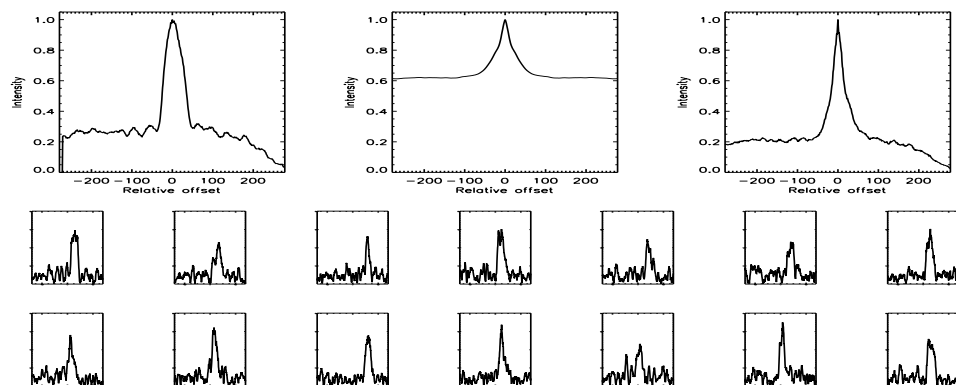
FIGURE B.513: SFP inspection for HD 179958 with S1-W1 on UT 2007/05/30, seq 002
