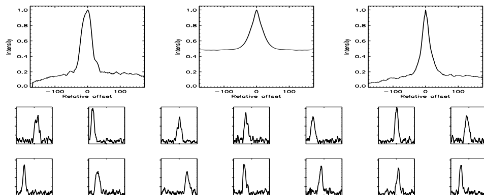
FIGURE B.12: SFP inspection for HD 003196 with S1-E1 on UT 2008/07/22, seq 001
