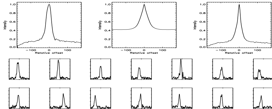
FIGURE B.407: SFP inspection for HD 139813 with S1-E1 on UT 2008/06/25, seq 001
