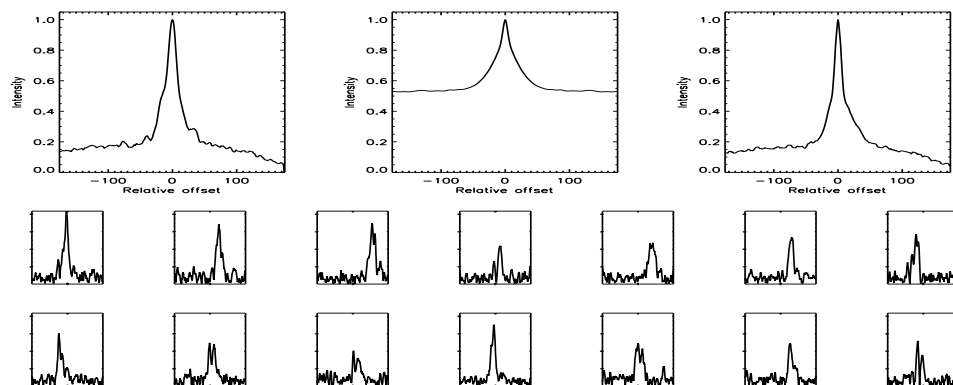
FIGURE B.444: SFP inspection for HD 155712 with S1-E1 on UT 2008/04/25, seq 001
