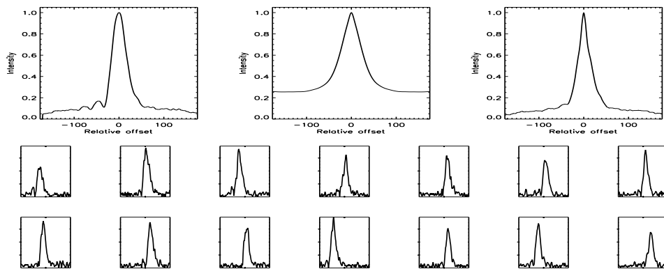
FIGURE B.364: SFP inspection for HD 135204 with S1-E1 on UT 2008/07/05, seq 001
