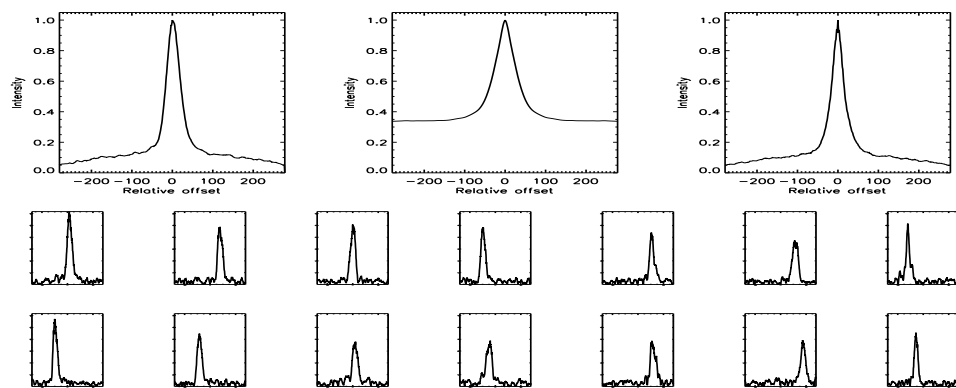
FIGURE B.286: SFP inspection for HD 110833 with S1-W1 on UT 2007/04/17, seq 002
