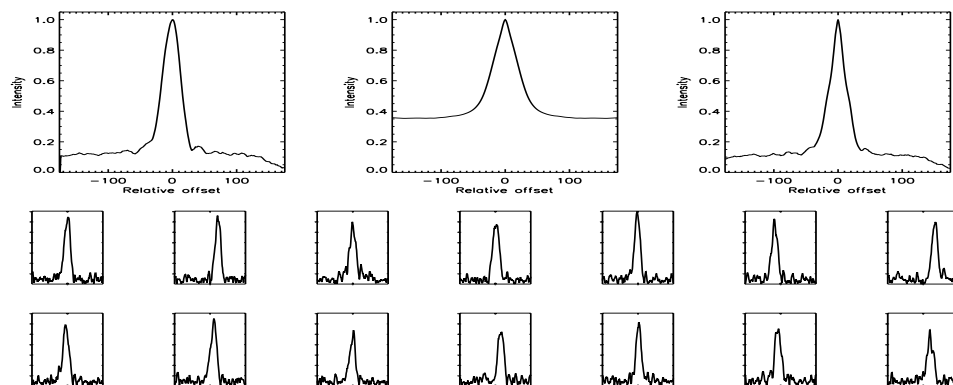
FIGURE B.462: SFP inspection for HD 159062 with S2-W1 on UT 2008/06/24, seq 001
