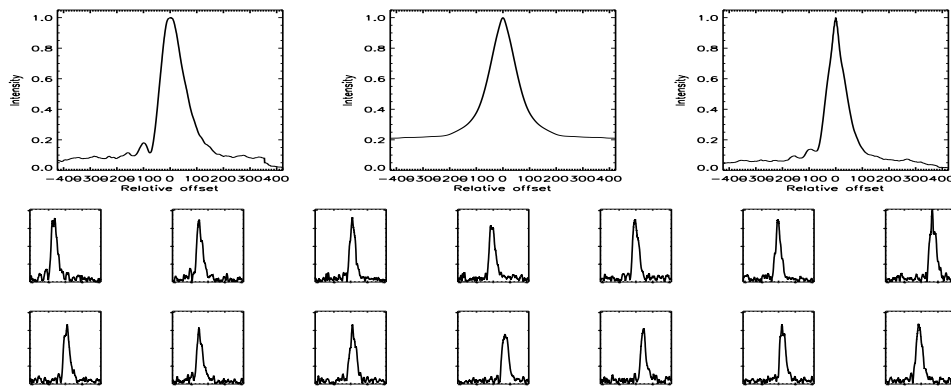
FIGURE B.630: SFP inspection for HD 219623 with S1-E1 on UT 2007/08/18, seq 002
