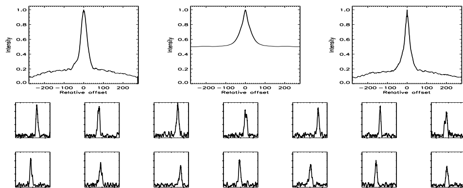
FIGURE B.280: SFP inspection for HD 108954 with S1-E1 on UT 2007/04/11, seq 001
