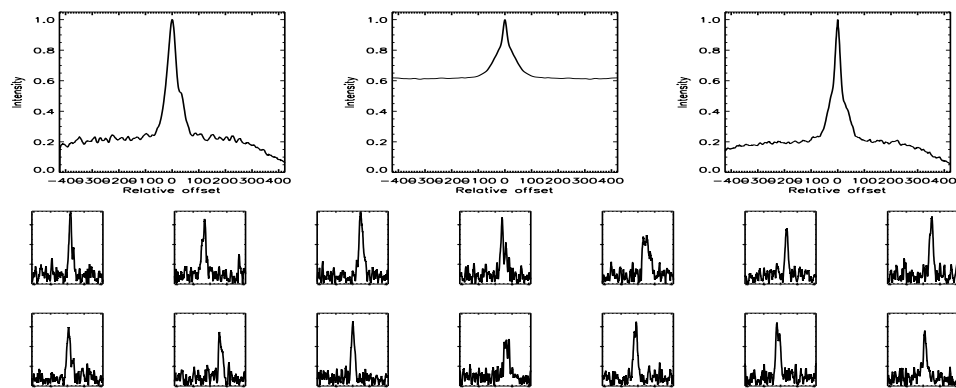
FIGURE B.84: SFP inspection for HD 018632 with S1-W1 on UT 2007/11/01, seq 002
