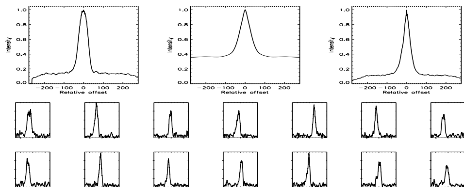
FIGURE B.616: SFP inspection for HD 217107 with S1-E1 on UT 2007/08/14, seq 001
