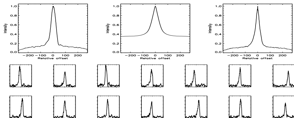
FIGURE B.514: SFP inspection for HD 180161 with S1-E1 on UT 2007/04/14, seq 001
