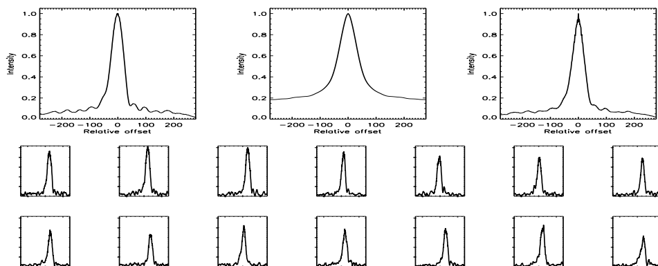
FIGURE B.528: SFP inspection for HD 185144 with S1-W1 on UT 2007/05/28, seq 001
