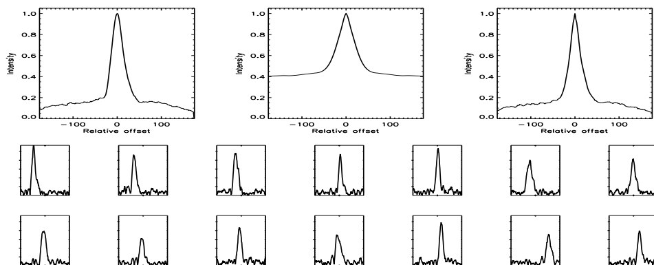
FIGURE B.417: SFP inspection for HD 144287 with S1-W1 on UT 2008/04/12, seq 001
