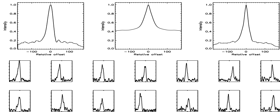
FIGURE B.238: SFP inspection for HD 094765 with S1-E1 on UT 2008/04/14, seq 001
