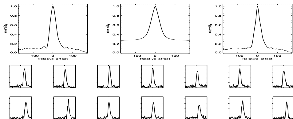
FIGURE B.409: SFP inspection for HD 139813 with S2-W1 on UT 2008/06/24, seq 001
