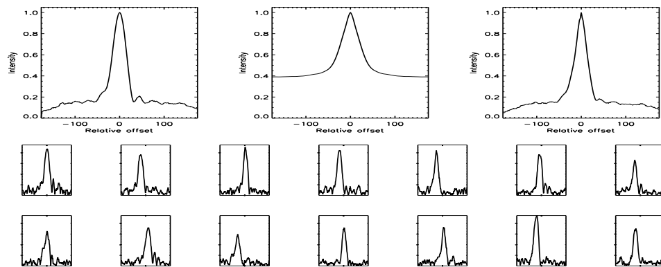
FIGURE B.223: SFP inspection for HD 082443 with S1-E1 on UT 2008/04/13, seq 001
