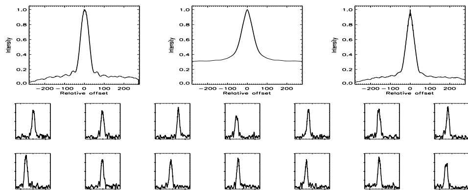
FIGURE B.561: SFP inspection for HD 191785 with S1-E1 on UT 2007/07/22, seq 001
