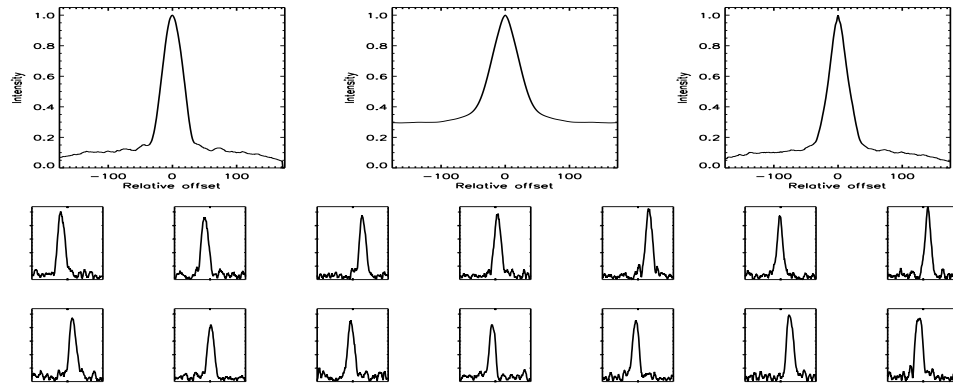
FIGURE B.32: SFP inspection for HD 004915 with S1-W1 on UT 2008/07/27, seq 001
