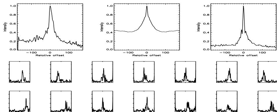
FIGURE B.649: SFP inspection for HD 222404 with S1-E1 on UT 2008/06/25, seq 001
