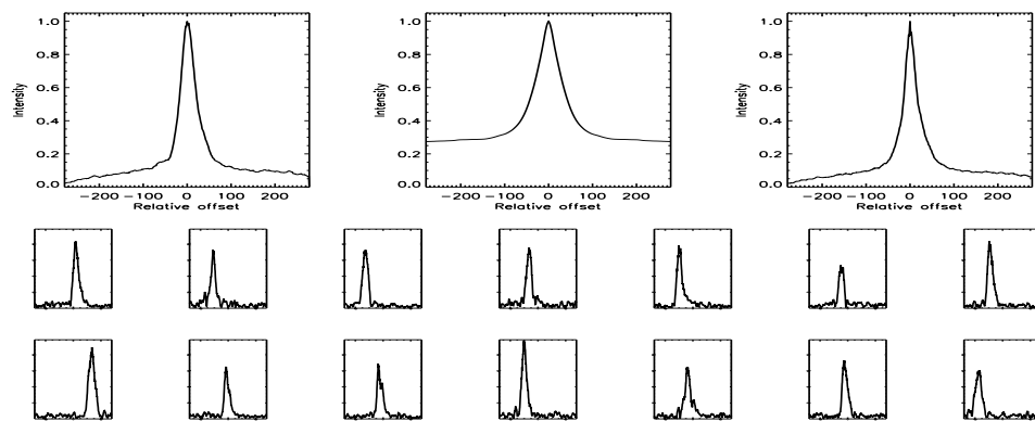
FIGURE B.228: SFP inspection for HD 082885 with S1-W1 on UT 2007/04/24, seq 001
