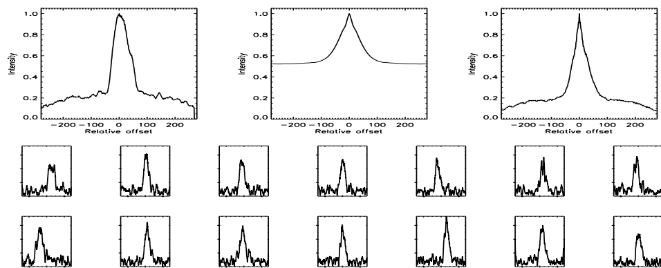
FIGURE B.99: SFP inspection for HD 022049 with S2-E2 on UT 2007/09/27, seq 001
