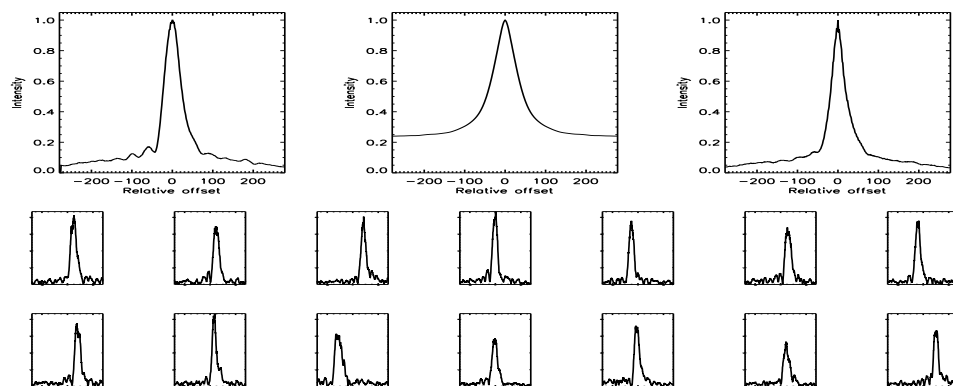
FIGURE B.487: SFP inspection for HD 166620 with S1-E1 on UT 2007/04/14, seq 001
