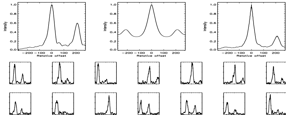
FIGURE B.11: SFP inspection for HD 003196 with S1-E1 on UT 2007/08/14, seq 003
