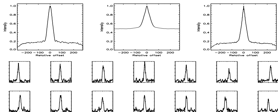
FIGURE B.520: SFP inspection for HD 182488 with S1-W1 on UT 2007/08/18, seq 001
