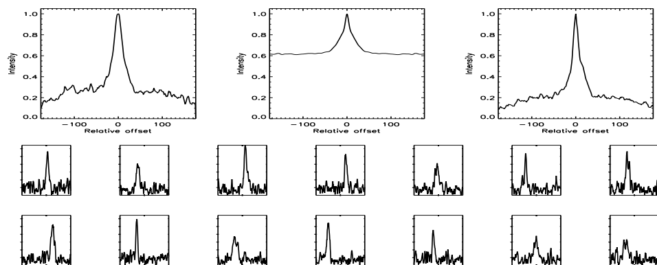
FIGURE B.340: SFP inspection for HD 128311 with S1-E1 on UT 2008/04/13, seq 001
