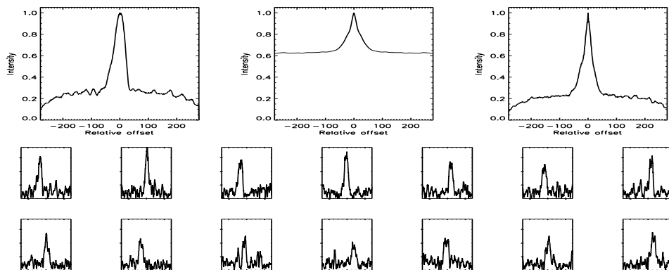
FIGURE B.508: SFP inspection for HD 179957 with S1-E1 on UT 2007/07/25, seq 002
