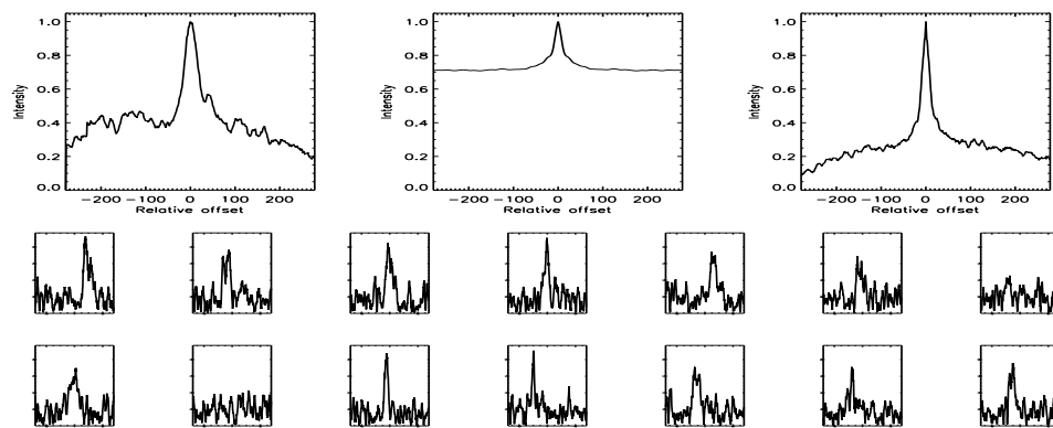
FIGURE B.399: SFP inspection for HD 139341 with S1-E1 on UT 2007/04/14, seq 001
