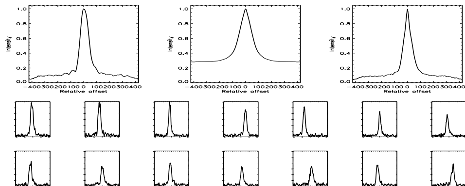
FIGURE B.530: SFP inspection for HD 185144 with S2-E1 on UT 2007/08/20, seq 001
