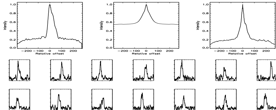
FIGURE B.158: SFP inspection for HD 038858 with S2-E2 on UT 2007/09/26, seq 001
