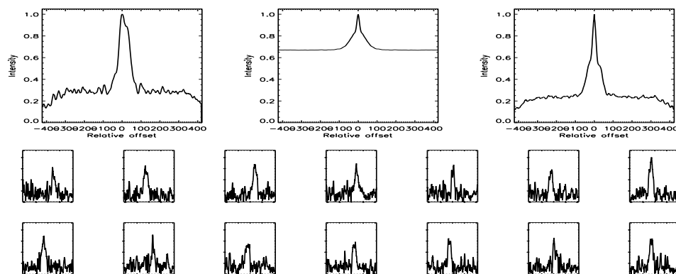
FIGURE B.7: SFP inspection for HD 001562 with S1-E1 on UT 2007/08/16, seq 002
