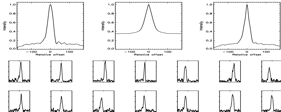
FIGURE B.413: SFP inspection for HD 142267 with S1-E1 on UT 2008/04/13, seq 001
