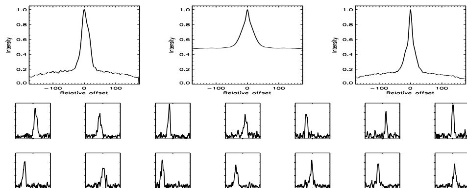
FIGURE B.330: SFP inspection for HD 125455 with S1-E1 on UT 2008/04/25, seq 001
