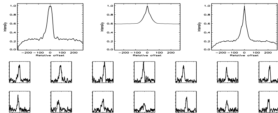
FIGURE B.549: SFP inspection for HD 190470 with S1-W1 on UT 2007/07/24, seq 002
