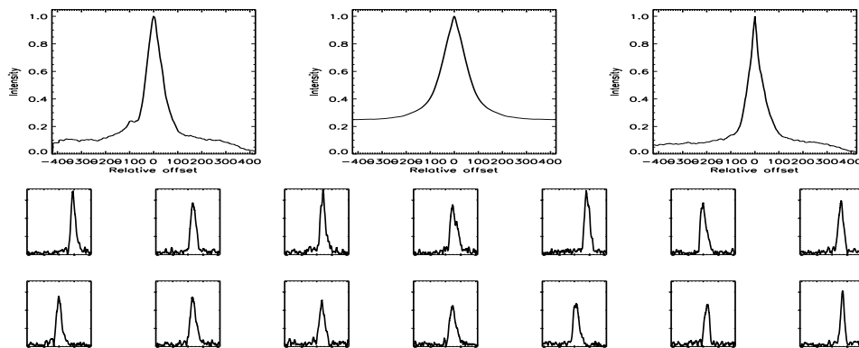
FIGURE B.526: SFP inspection for HD 185144 with S1-E1 on UT 2007/07/28, seq 001
