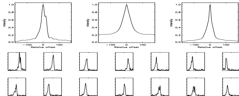
FIGURE B.422: SFP inspection for HD 146233 with S1-E1 on UT 2008/04/25, seq 001
