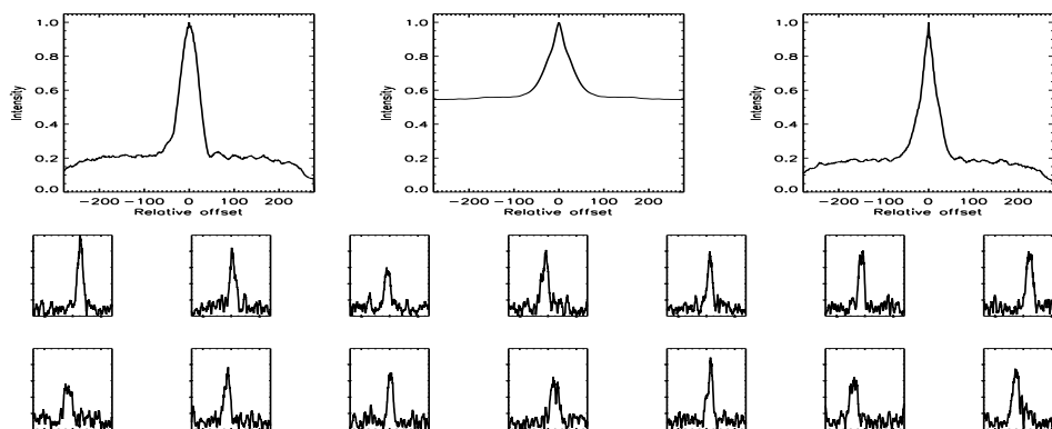
FIGURE B.547: SFP inspection for HD 190470 with S1-E1 on UT 2007/07/24, seq 001
