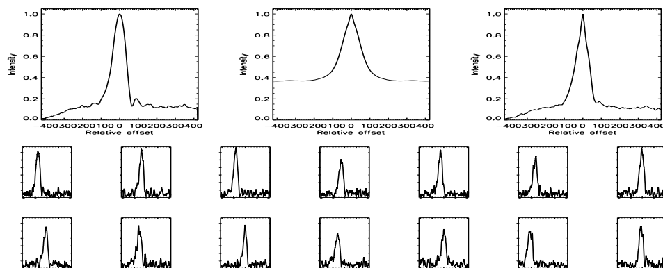
FIGURE B.544: SFP inspection for HD 190067 with S1-W1 on UT 2007/07/22, seq 001
